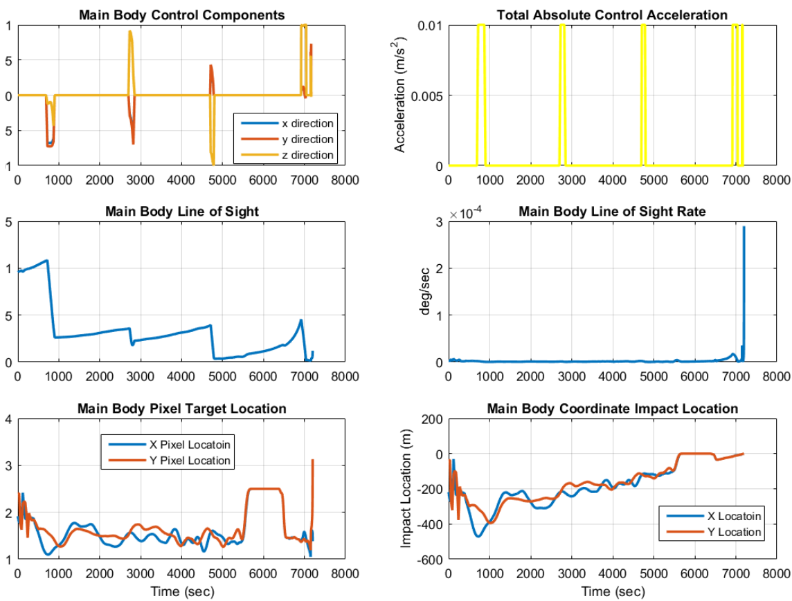
Figure 4.16: CV control accelerations and mission variables using filtered camera information.
