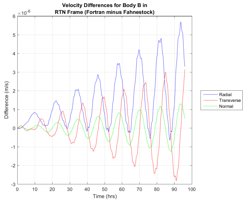
Figure 5.18: RTN frame velocity difference for Didymoon.
