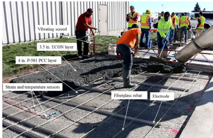
Figure 3. ECON HPS construction procedure at DSM
