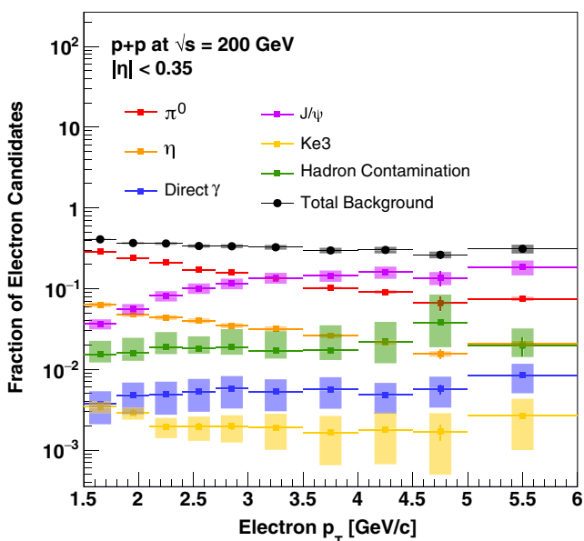
FIG. 10. Fraction of the measured candidate electron sample attributable to various sources of background electrons as a function of p_T .
