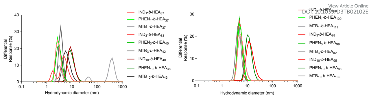
Figure 4. Size distribution (Volume %) of copolymers' self-assemblies (1 mg/mL) in DI water as determined by DLS.
