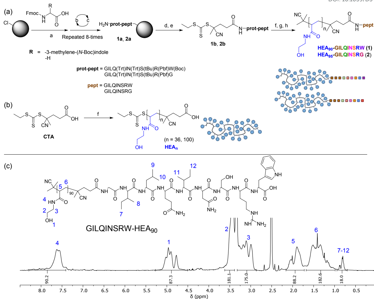
Figure 1. (a) Synthesis of HEA 90 -GILQINSRW, and HEA 95 -GILQINSRG; (b) synthesis of HEA n as control polymers; (c) 1 H NMR (400 MHz, DMSO-d 6 ) spectra of obtained GILQINSRW-HEA 90 conjugation. Reagents and conditions: a) DMF, DIPEA, rt; b) DMF, piperidine, rt; c) DMF, Fmoc-amino acid, HATU, DIPEA, rt; d) CTA, HATU, TEA, DMF, rt; e) DCM/TFE 8:2 v/v, rt; f) N -Hydroxyethyl acrylamide, V501, DMF, 70 °C; g) AIBN, DMF, 80 °C; h) 0.1 N HCl in hexafluoro-2-propanol (HFIP), rt.
