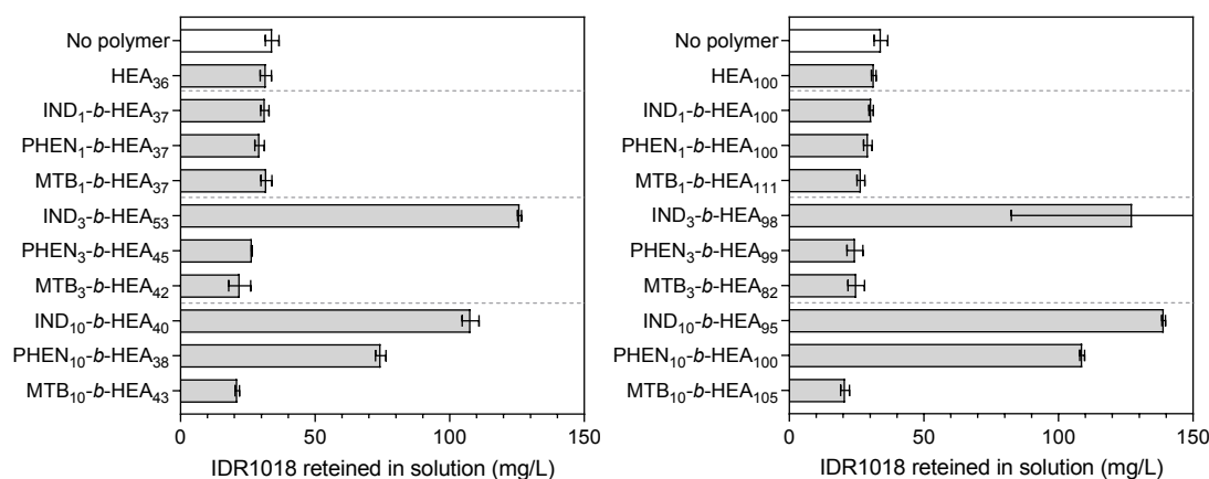
Figure 7. The concentration of IDR 1018 remaining in a solution after incubation in aggregation conditions (100 mM phosphate buffer, pH 7.2) for 5 h without and with synthesised copolymers at 1:1 molar ratio; the initial concentration of the peptide was 0.153 mg/mL. Higher values in the graph correspond to better protein stabilisation and hence reduced aggregation.
