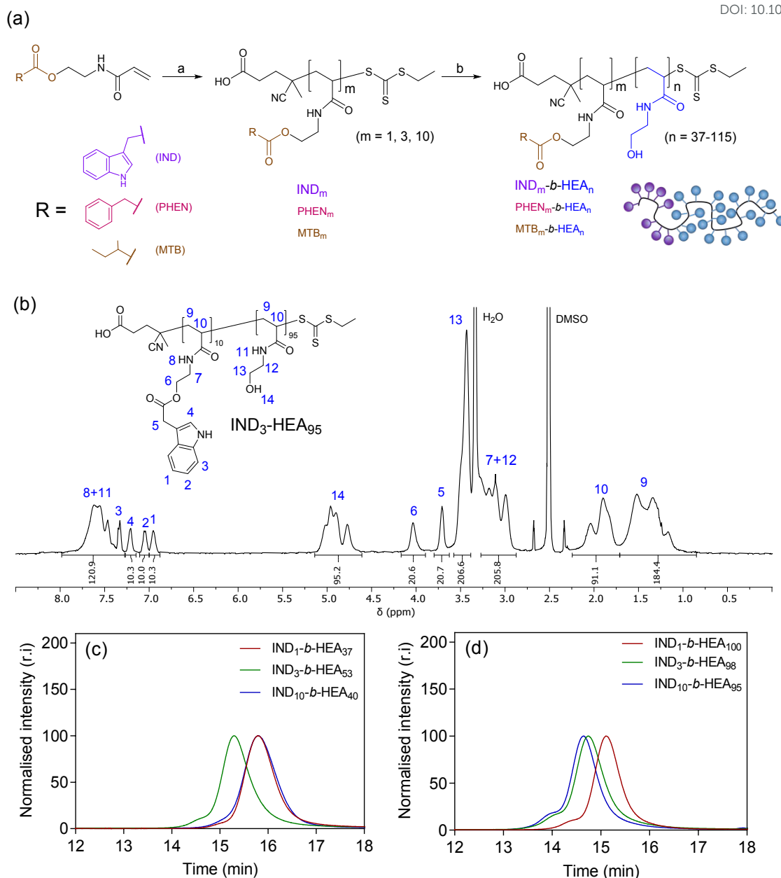
Figure 3. (a) Synthesis of \text{IND}_m^- , \text{PHEN}_m^- , \text{MTB}_m^- - b - \text{HEA}_n block copolymers. Reagents and conditions: a) AIBN, CTA, DMF, 80 °C; b) N -hydroxyethyl acrylamide, V501, DMF, 70 °C; (b) ^1\text{H} NMR (DMSO- d_6 , 400 MHz) spectrum of \text{IND}_3 - \text{HEA}_{95} as a representative spectrum of the synthesised block copolymers; SEC chromatograms of \text{IND}_m^- - b - \text{HEA}_n copolymers with (c) shorter and (d) longer hydrophilic blocks, using DMF with 0.1% LiBr as the mobile phase. Spectra and SEC chromatograms of all polymers are shown in Sections 5.3.1 and 5.3.2 in the supporting information.
