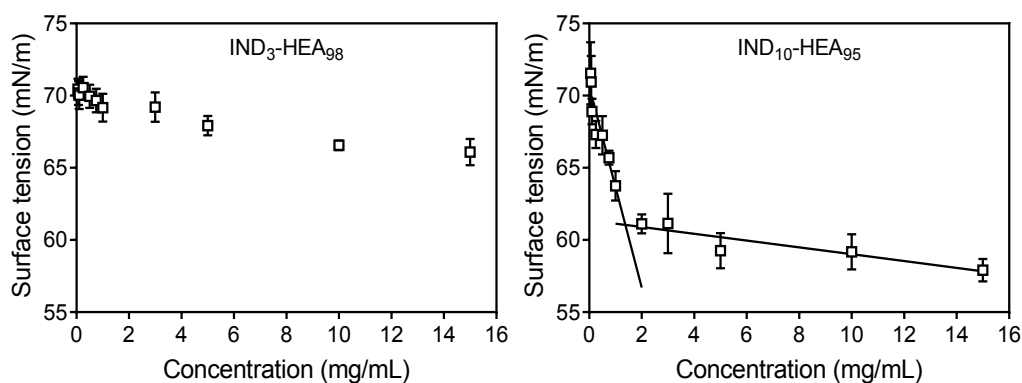
Figure 5. Surface tension measurements of representative copolymers \text{IND}_{3^{-}b}\text{-HEA}_{98} and \text{IND}_{10^{-}b}\text{-HEA}_{95} carried out in water by pendant drop method. 36
