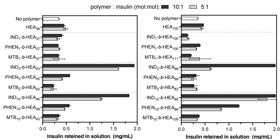
Figure 6. Insulin aggregation in the presence of \text{IND}_m -, \text{PHEN}_m - and \text{MTB}_m - b - \text{HEA}_n materials. Concentration of insulin remaining in a solution after incubation in the aggregation inducing conditions (pH 5.2) for 20 h without and with synthesised copolymers at different molar ratio; the initial concentration of insulin was 2 mg/mL. Higher values in the graph correspond to better protein stabilisation and hence reduced aggregation.
