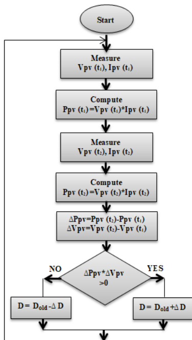
Figure 6. The improved P&O flowchart.
