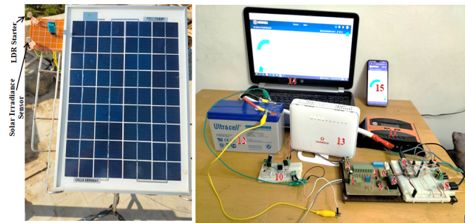
Figure 4. The implemented IoT prototype a) The installed PV panel, LDR starter, and solar irradiance sensor and b) The practical control system, 1) LDR starter jumper, 2) 5V from regulator, 3) Operational amplifier, 4) Transistor BC547BP, 5) 5V Relay, 6) 5V to Node MCU, 7) 2 jumpers from solar radiation sensor to 3.3V of Node MCU and analog pins A0, 8) Usb cable, 9) Node MCU ESP8266, 10) Regulator LM7805CT and diode 1N4007, 11) Solar charger controller (12V, 10A), 12) Rechargeable PV battery (12V, 7.2A), 13) Router, 14) Laptop, 15) Mobile phone.
