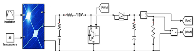
Figure 5. The PV source linked with DC-DC boost converter.
