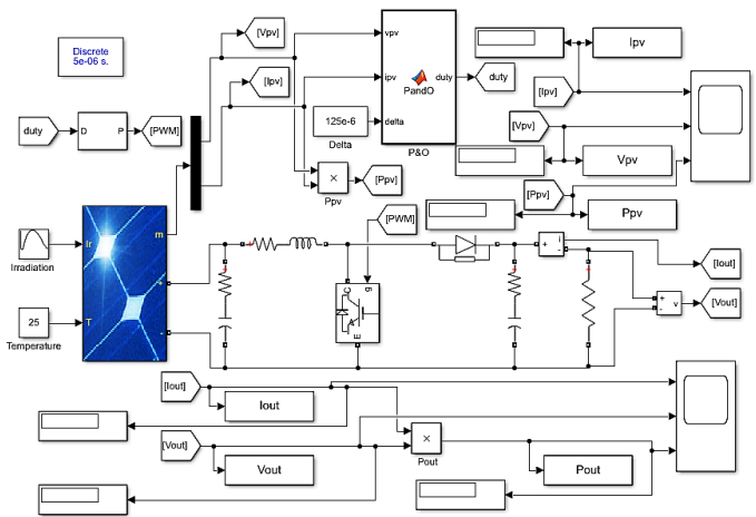
Figure 7. The block diagram of P&O MPPT controller.
