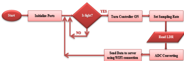
Fig. 2. The proposed IoT block diagram and flow chart.
