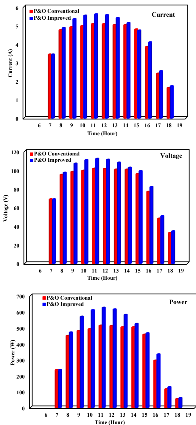
Figure 9. The output current, voltage, and maximum output power of the conventional and improved P&O.
