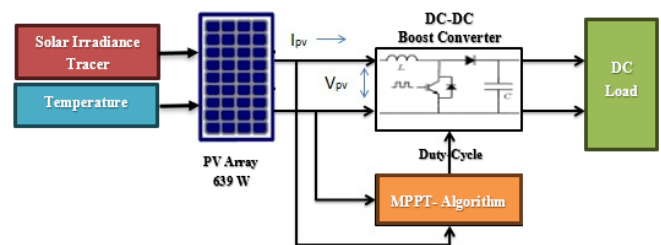
Figure 1. The block diagram of the proposed IoT and P&O system.
