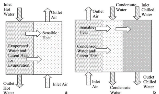
Figure 2. Schematic illustrating the heat and mass transfer processes occurring in both the humidifier (a) and (b) the dehumidifier [17].
