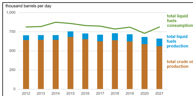
Fig. 2. Total annual fuel production and consumption in Egypt [18]
