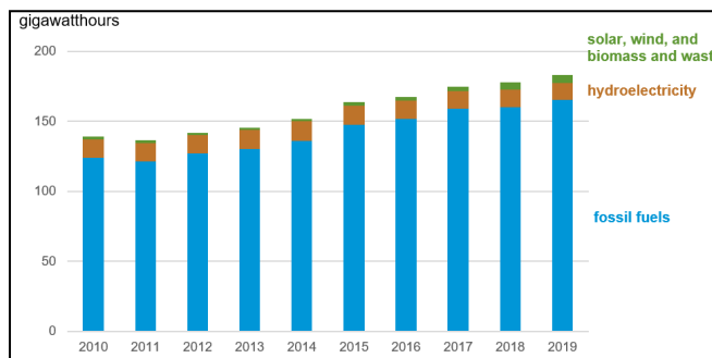
Fig. 3. Net electricity generation in Egypt [18]
