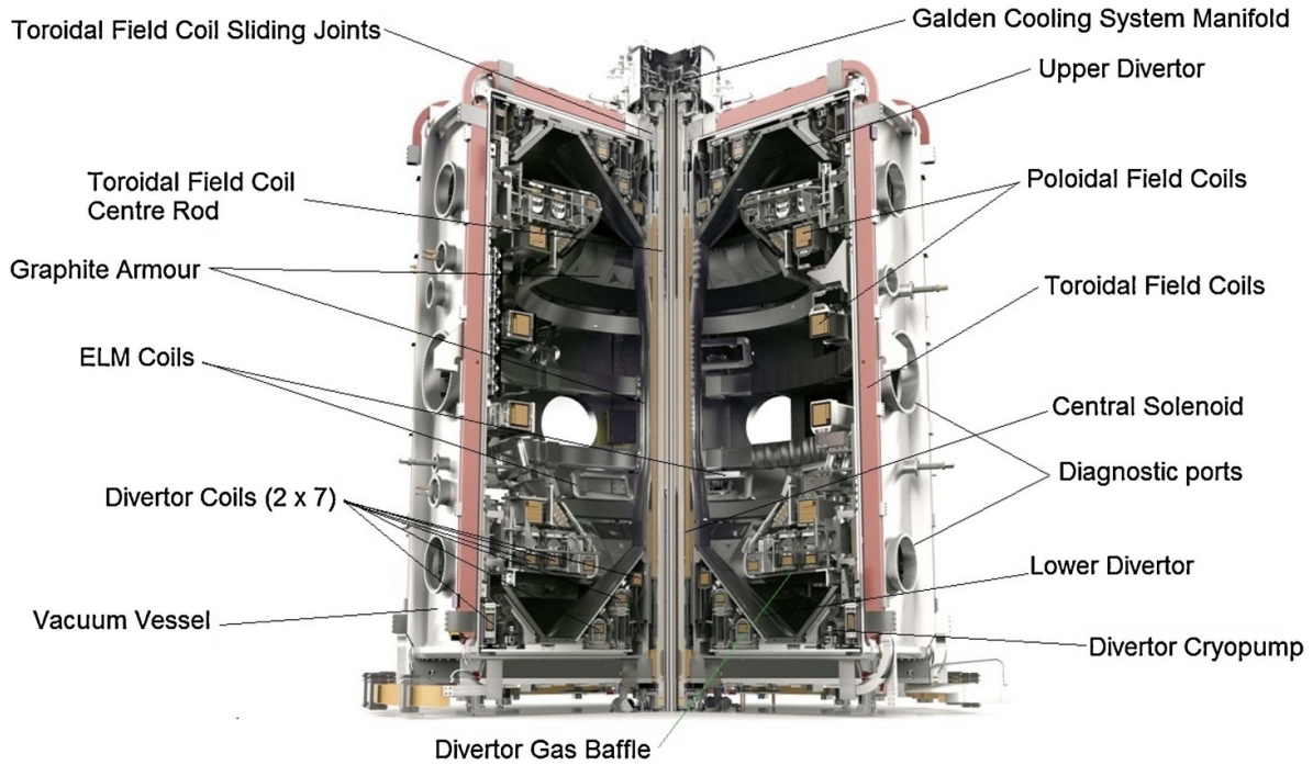
Figure 1. Annotated cross-sectional schematic of MAST Upgrade. Reprinted from [6], Copyright (2015), with permission from Elsevier.
