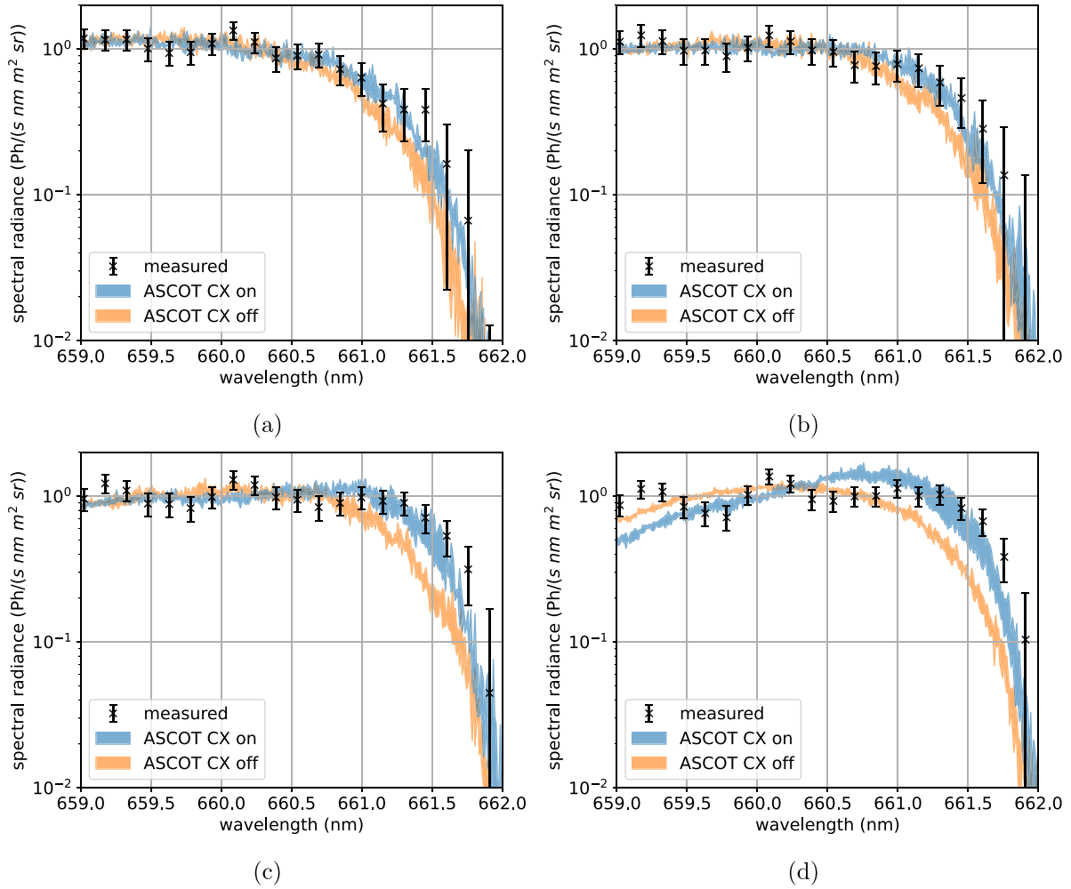
Figure 11. Normalized ASCOT5-FIDASIM-simulated and bremsstrahlung-corrected measured passive FIDA spectra (logarithmic scale) for channels 8 (a), 9 (b), 10 (c) and 11 (d) (out of 11 channels) in shot 45091 at 0.35 s. Each spectrum was normalized by division with its average value between wavelengths 659.0 and 661.0 nm. Graphs for the normalized spectra predicted using the best-estimate and limiting-estimate neutral density profiles were merged into a single colour band whose borders at each wavelength are the minimum and maximum values from across the three individual spectra. Those neutral density profiles were used whose TRANSP parts include recombination atoms.
