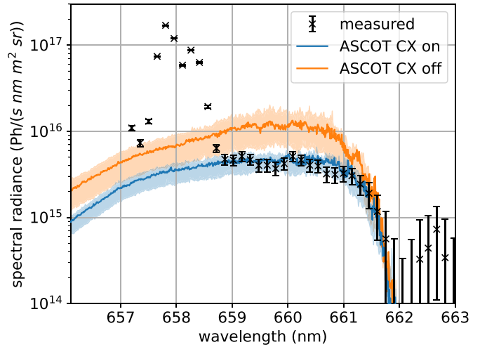
Figure 7. ASCOT5-FIDASIM-simulated and measured passive FIDA spectra (logarithmic scale) for channel 9 (out of 11 channels), with tangency radius 1.29 m ( \rho_p = 0.70 ), in shot 45091 at 0.35 s. Bremsstrahlung has been estimated as the signal average between 662.0 and 662.4 nm and subtracted from the measured spectrum. Predictions using the best-estimate neutral profile whose TRANSP part includes recombination atoms are shown using solid lines. The corresponding limiting-estimate cases are indicated with shaded colour bands.
