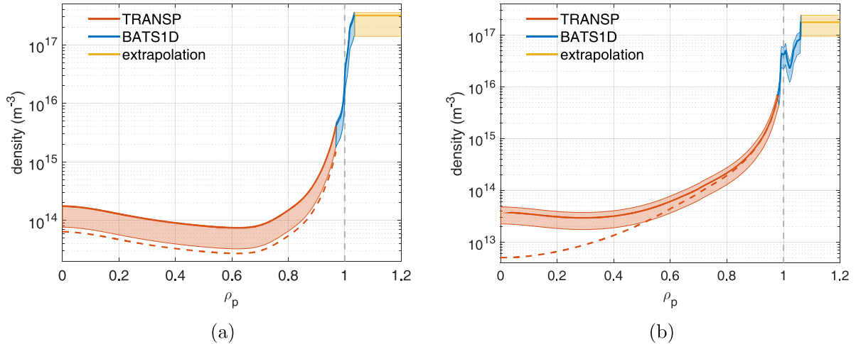
Figure 2. Outer-midplane neutral deuterium density reconstructions for shot 44623 at time 0.40 s (a) and shot 45091 at 0.35 s (b) as functions of the normalized poloidal flux \rho_p = \sqrt{(\psi_p - \psi_{p,ax}) / (\psi_{p,sep} - \psi_{p,ax})} , where \psi_p is the poloidal flux, and \psi_{p,ax} and \psi_{p,sep} are its values at the magnetic axis and inside the separatrix, respectively. In (a), BATS1D part based on proxy shot 44578 at 0.32 s. Extrapolation of maximum BATS1D value in yellow. Best-estimate profile shown using solid lines, limiting-estimate profiles using shaded colour bands. In (a), TRANSP-part version that was not scaled to BATS1D part is shown using dashed orange line. In (b), TRANSP-part version with both wall atoms and recombination atoms shown using solid orange line and orange colour band, while best-estimate TRANSP-part version with only wall atoms is shown using dashed orange line.
