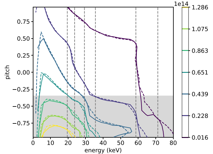
Figure A2. Distribution functions predicted by ASCOT4 (solid) and ASCOT5 (dashed) for beam ions in MAST-U shot 44623 at 0.39 s, integrated over the whole spatial domain. Each distribution is an average of the predictions from eight simulations of the same case, differing only in the random seeds of the markers. Pitch = v_{\parallel} / v , where v_{\parallel} is the velocity component parallel to the magnetic field line and v is the total speed. Neutral-beam injection energies are indicated using grey dashed lines and the range of initial pitch values using a shaded grey band.
