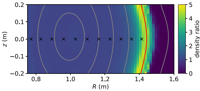
Figure 10. Ratio between the beam-ion density around the outer midplane in shot 45091 at 0.35 s predicted by ASCOT5 when CX is off and the one predicted when CX is simulated using the best-estimate neutral density profile whose TRANSP part includes recombination atoms. Equilibrium is illustrated using contours for \rho_p = 0.2, 0.4, 0.6, 0.8 and 1.2 in grey and for \rho_p = 1.0 in red. Tangency points of FIDA channels are indicated by black crosses.
