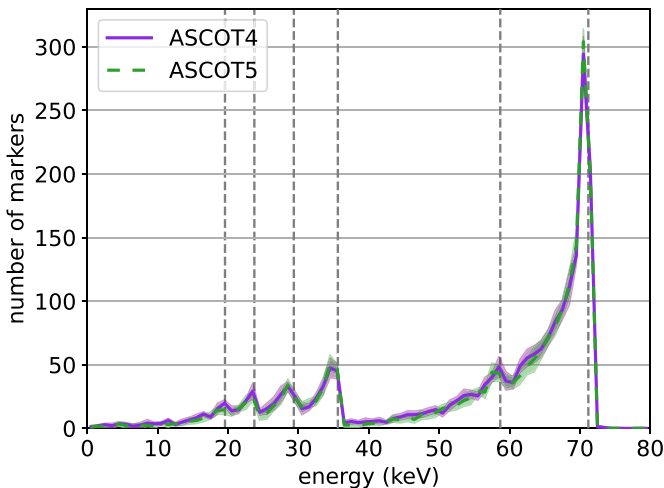
Figure A3. Simulated spectra for the final kinetic energies of beam-particle markers that hit the wall in MAST-U shot 44623 at 0.39 s. Each spectrum is an average of the predictions from eight simulations of the same case, differing only in the random seeds of the markers. The shaded colour bands indicate estimated margins of standard error, with colours matching the corresponding average spectrum. Neutral-beam injection energies are indicated using grey dashed lines.
