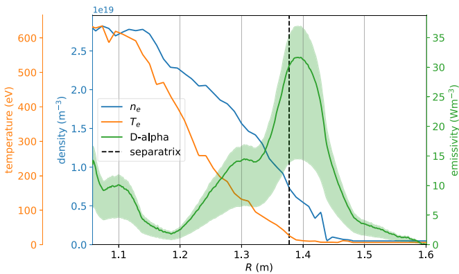
Figure 3. Outer-midplane HOMER D-alpha and Thomson scattering electron density n_e and temperature T_e data used for estimating the neutral density in shot 45469 at 0.40 s, plotted as functions of major radius. For the D-alpha profile, the result when scaling with the best-estimate scaling factor for this case, 4.8, is shown with the solid green line. The results using the minimum and maximum scaling factors, 2.2 and 5.6, respectively, are indicated using a shaded green band.
