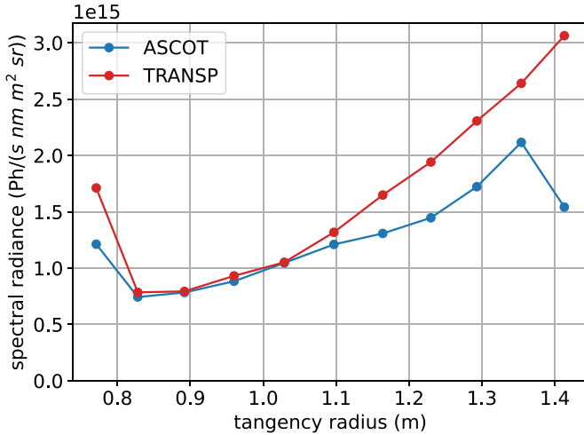
Figure 8. Passive FIDA signals in shot 45091 at 0.35 s predicted by ASCOT5-FIDASIM and TRANSP-FIDASIM as functions of the tangency radii of the FIDA channels (corresponding \rho_p coordinates range from \rho_p = 0.47 on the high-field side to \rho_p = 0.95 on the low-field side). For each model and each channel, the passive FIDA spectrum has been averaged between wavelengths 659.0 and 661.0 nm.
