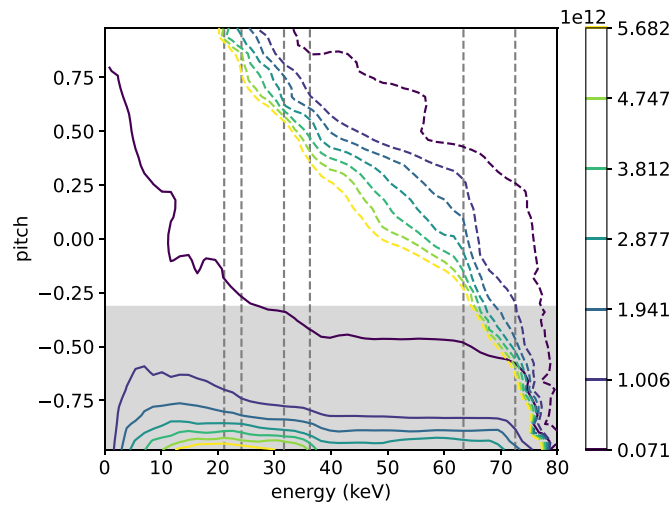
Figure 12. Distribution functions for beam ions in shot 45091 at 0.35 s predicted by ASCOT5 when CX is off (dashed) and when CX is simulated using the best-estimate neutral density profile whose TRANSP part includes recombination atoms (solid), integrated over the spatial domain where R = 1.33\text{--}1.60 m and z = -0.10\text{--}0.10 m (figure 10). Pitch = v_{\parallel}/v , where v_{\parallel} is the velocity component parallel to the magnetic field line and v is the total speed. Neutral-beam injection energies are indicated using grey dashed lines and the range of initial pitch values using a shaded grey band.
