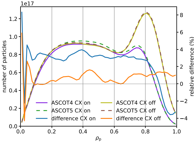
Figure A1. Simulated beam-ion content in MAST-U shot 44623 at 0.39 s as a function of the normalized poloidal flux \rho_p = \sqrt{(\psi_p - \psi_{p,ax}) / (\psi_{p,sep} - \psi_{p,ax})} , where \psi_p is the poloidal flux, and \psi_{p,ax} and \psi_{p,sep} are its values at the magnetic axis and inside the separatrix, respectively. Beam-ion content is given as number of particles in the volume corresponding to the \rho_p coordinate. Each profile is an average of the predictions from eight simulations of the same case, differing only in the random seeds of the markers. Relative differences in the profiles from the two ASCOT versions are shown on a separate axis.
