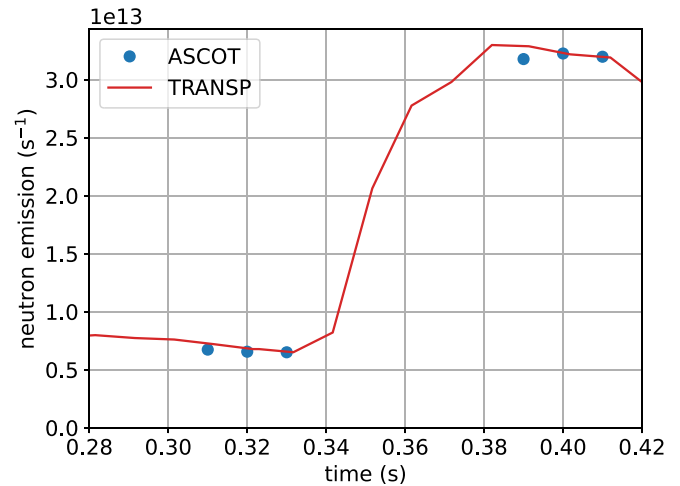
Figure 5. Total neutron rate from the plasma in shot 44623 as predicted by ASCOT4-AFSI and TRANSP using the TRANSP neutral density and including CX.
