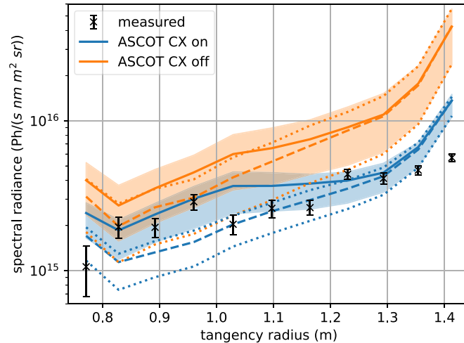
Figure 9. ASCOT5-FIDASIM-simulated and bremsstrahlung-corrected measured passive FIDA signals (logarithmic scale) in shot 45091 at 0.35 s as functions of the tangency radii of the FIDA channels. For each channel, the simulated and measured passive FIDA spectra have been averaged between wavelengths 659.0 and 661.0 nm. Predictions using the best-estimate neutral profile whose TRANSP part includes recombination atoms are shown using solid lines. The corresponding limiting-estimate cases are indicated with shaded colour bands. Predictions using the best-estimate neutral profile excluding recombination atoms are shown using dashed lines. The corresponding limiting-estimate cases are indicated with dotted lines.
