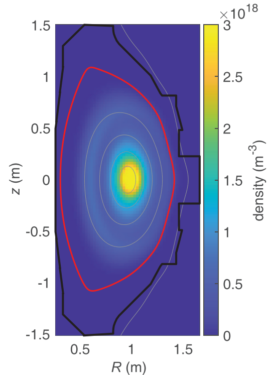
Figure 4. Beam-ion density predicted by ASCOT4 in shot 44623 at 0.39 s when CX reactions are not accounted for. Equilibrium contours for \rho_p = 0.2, 0.4, 0.6, 0.8 and 1.2 in grey and for \rho_p = 1.0 in red, and the 2D wall representation in black are indicated.
