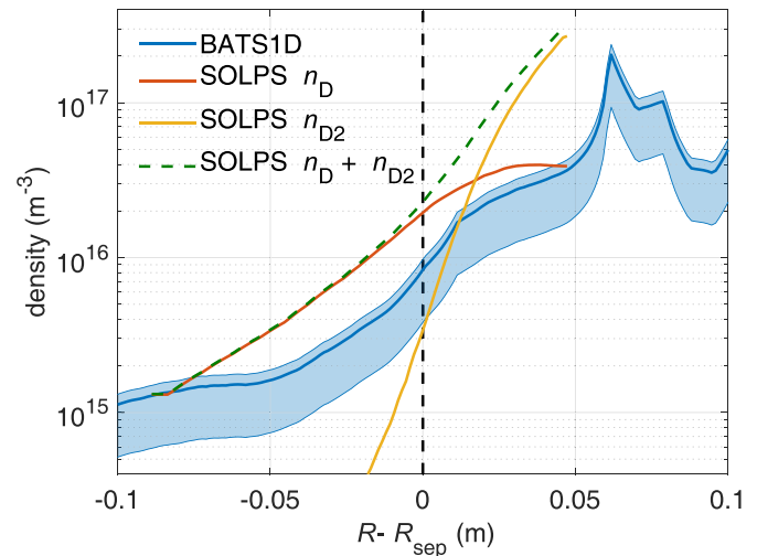
Figure C1. Estimates by BATS1D and SOLPS-ITER of the outer-midplane neutral deuterium density near the separatrix in shot 45469 at 0.40 s as a function of major radius minus the major-radius coordinate of the separatrix. For SOLPS-ITER, atomic ( n_D ) and molecular ( n_{D2} ) densities are also shown separately. For BATS1D, the result when scaling with the best-estimate scaling factor for this case, 4.8, is shown using a solid blue line. The results using the minimum and maximum scaling factors, 2.2 and 5.6, respectively, are indicated using a shaded blue band.
