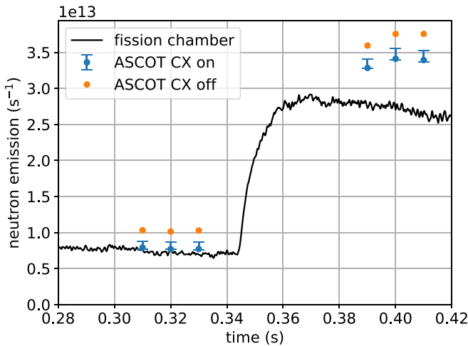
Figure 6. Total neutron rate from the plasma in shot 44623 as measured by the fission chamber, with an additional scaling factor of 3.0, and as predicted by ASCOT4-AFSI, with and without the inclusion of CX. CX was simulated using the neutral density reconstructions based on BATS1D calculations. Predictions when CX was simulated using the best-estimate neutral profiles are shown using blue dots and the limiting-estimate cases are indicated with blue error bars.
