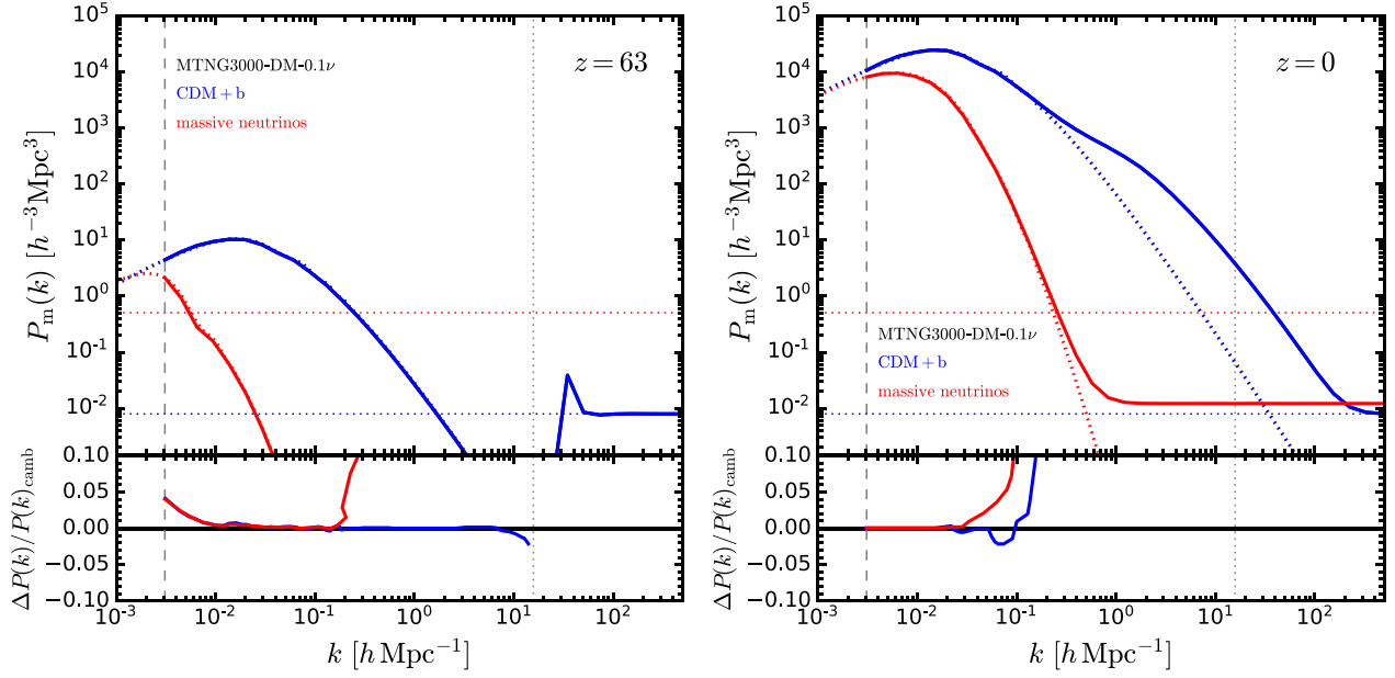
Figure 3. Power spectrum measurements for our MTNG3000-DM-0.1 \nu run at the initial time (left-hand panel, z = 63 ) and the final time (right-hand panel, z = 0 ). In both cases we show the measured power spectrum of the cold matter particles (CDM and baryons; solid blue line) and of the neutrino particles (solid red line), and we compare to the expected linear theory power spectrum (thin dotted curves) as computed by CAMB (Lewis et al. 2000) for this cosmology (which includes neutrinos that transition from the relativistic into the non-relativistic regime, as well as a photon background). The dashed vertical line shows the fundamental mode of the box, while the vertical thin dotted line gives the Nyquist frequency of the initial DM particle grid. The dotted horizontal lines give the nominal shot noise of the two particle sets, 10240^3 for the DM, and 2560^3 for the neutrinos. Despite this, the actual shot noise realized by the neutrinos at late times is much lower, thanks to the \delta f -simulation technique (Elbers et al. 2021), and is in fact close to the one of the dark matter at late times. In the bottom panel, we give the relative deviation of the measured power spectrum modes relative to linear theory. Note that in the initial conditions, we deliberately create a small boost in the linear power at the largest scales in order to offset the fact that our code treats super-horizon modes with Newtonian gravity. With this correction, the simulation-evolved linear power spectrum is fully correct at z = 0 at large scales by construction, while at higher redshift, there will be a small residual difference. However, at z = 5 , when the outputting of our deepest light cone starts, the difference to the relativistic result at the fundamental mode of the box has already dropped to just 0.7 per cent, and this value shrinks rapidly further towards lower redshift, and in any case also quickly towards higher k .
