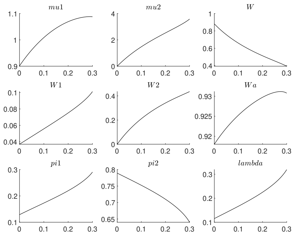
Figure D.5: Nash-bargaining equilibrium outcomes as a function of \beta_2 when \beta_1 = 0.7
