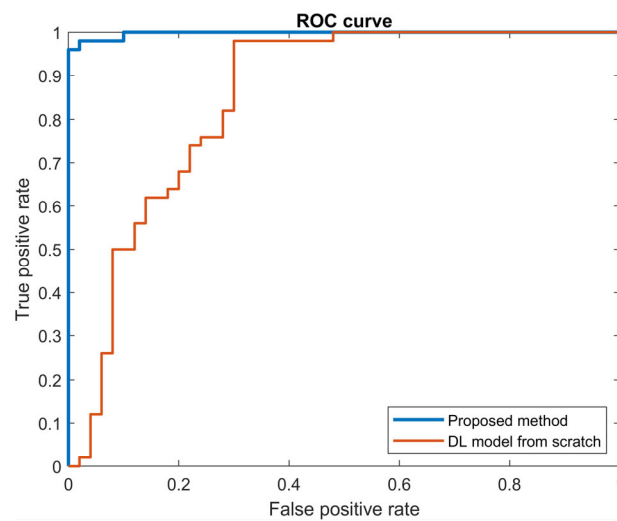
Figure 8. ROC curves.
