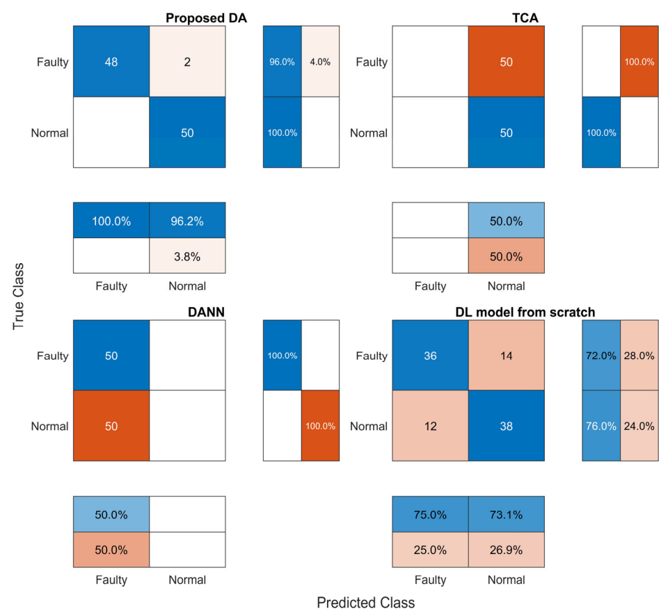
Figure 7. Confusion matrix.
