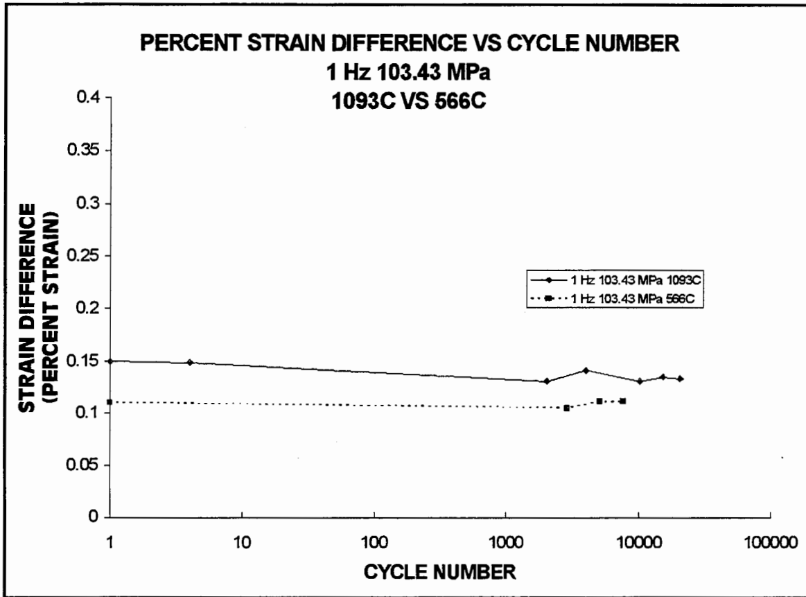
Figure 62. Strain Difference 1 Hz 103.43 MPa 566 °C vs 1093 °C
