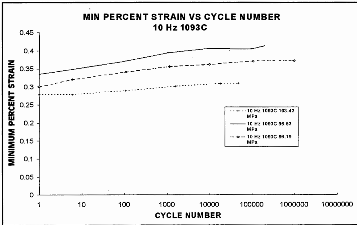
Figure 43. Minimum Strain 10 Hz 1093°C
