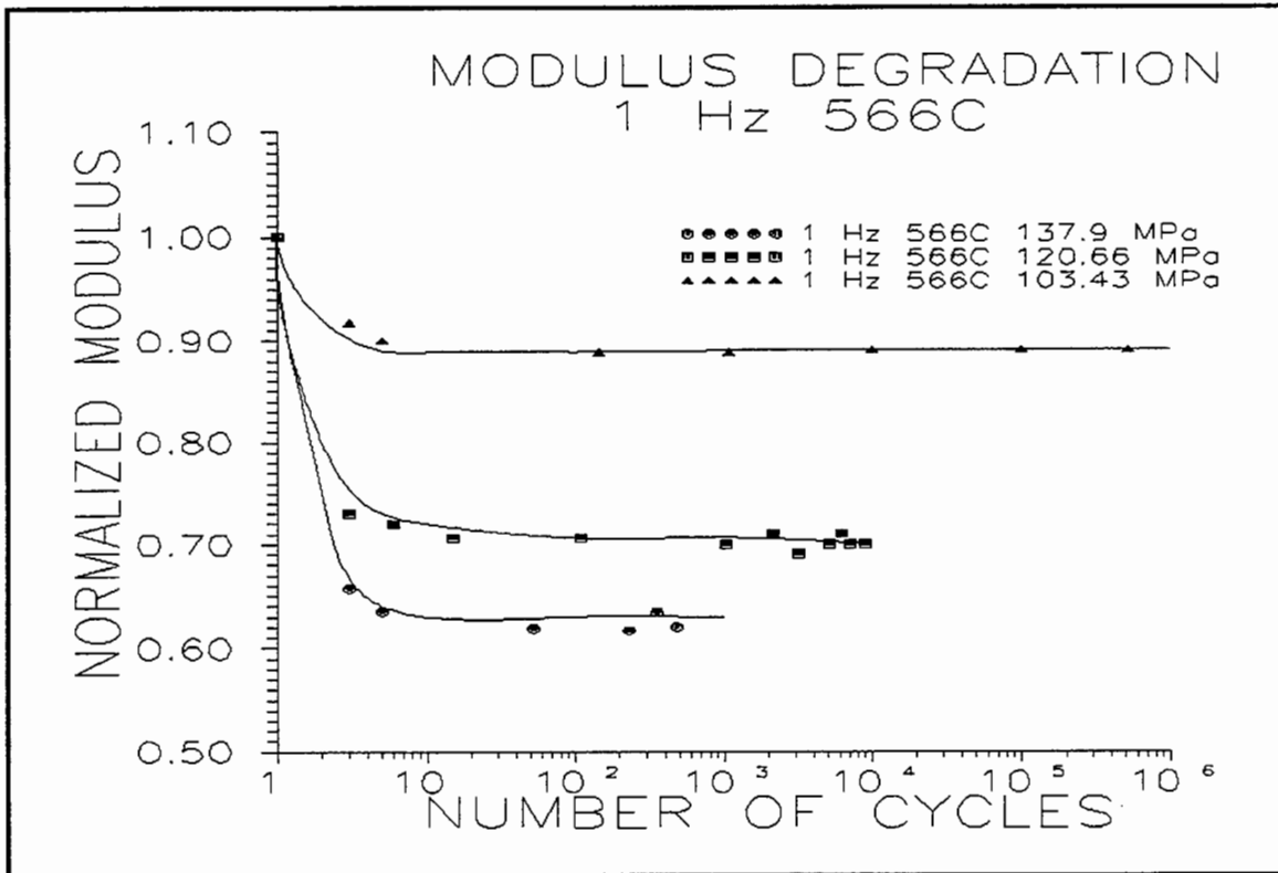
Figure 19. Modulus Degradation 566°C 1 Hz
