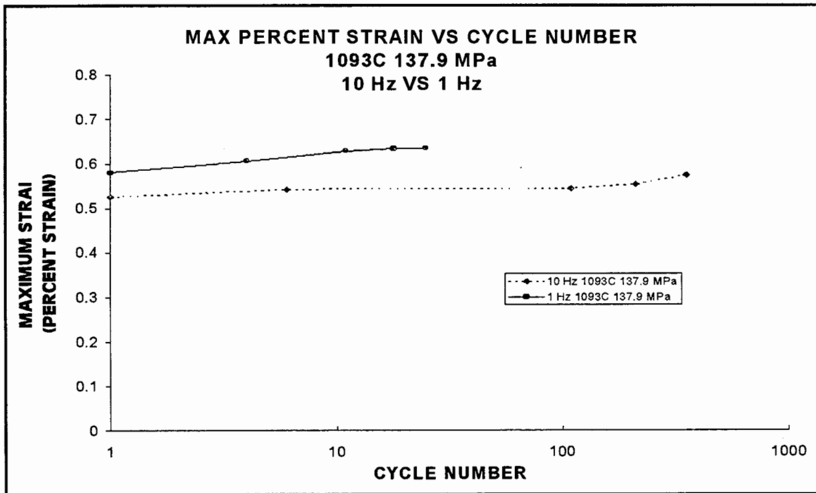
Figure 48. Maximum Strain 1093°C 137.9 MPa 1 Hz vs 10 Hz
