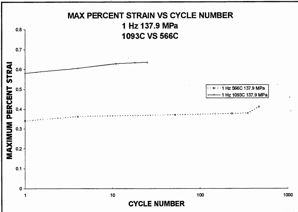
Figure 59. Maximum Strain 1 Hz 137.9 MPa 566°C vs 1093°C
