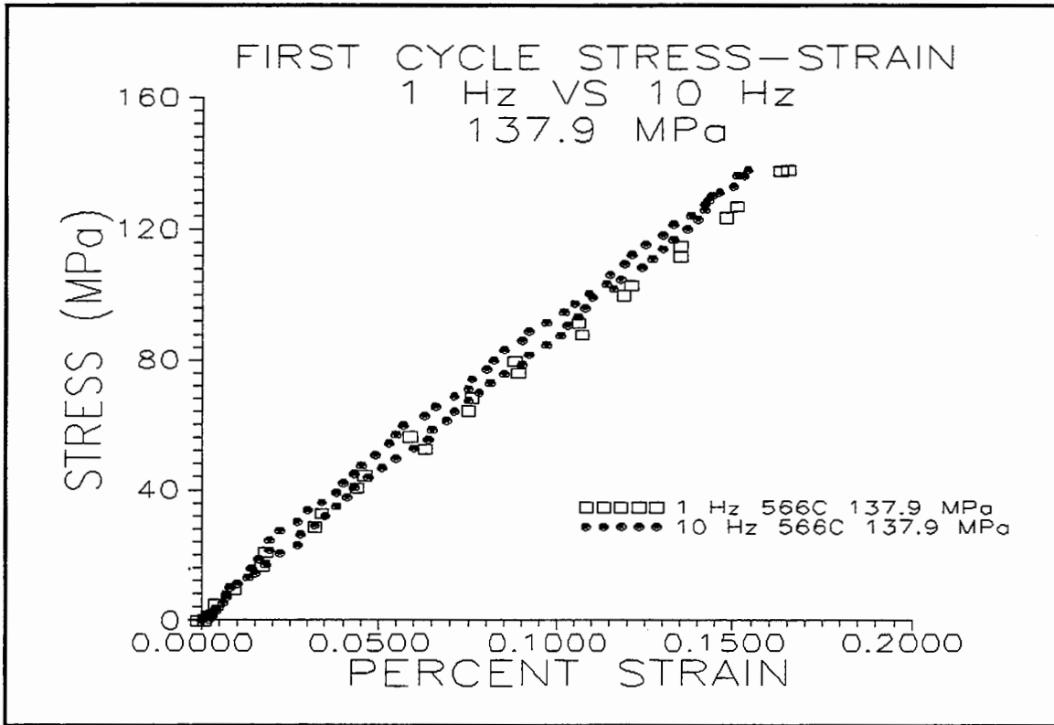
Figure 53. First Cycle Stress Strain 566°C 1 Hz vs 10 Hz
