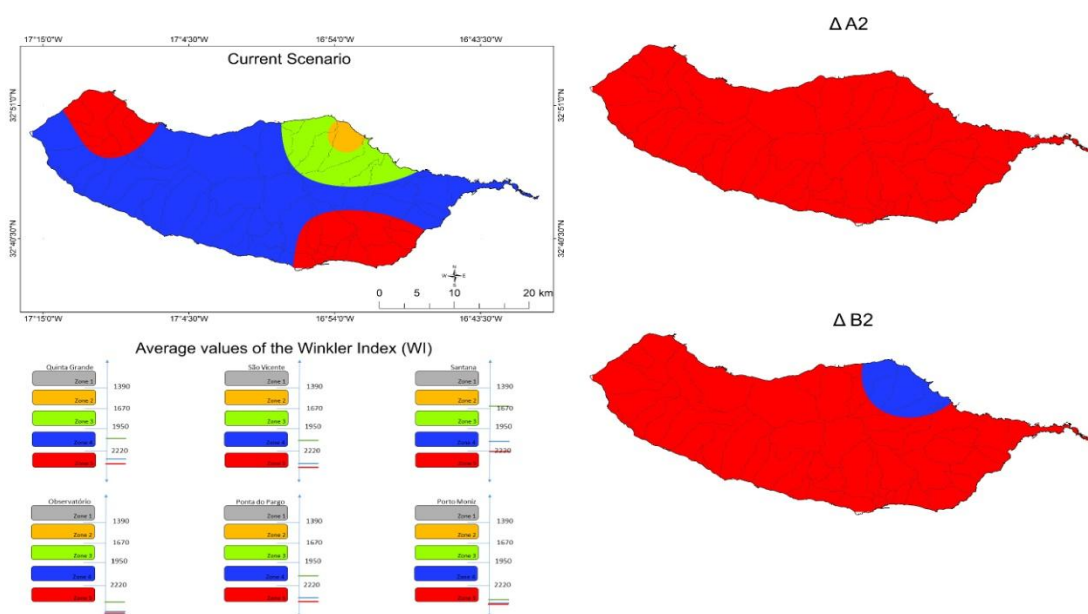
Figure 6. Interpolation of the Winkler Index (WI), for the current scenario and for the \Delta A2 and \Delta B2 scenarios proposed by Madeira Climate Strategy for 2070-2099
