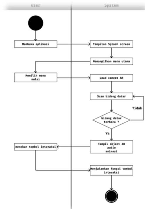
Gambar 5. Activity Diagram
