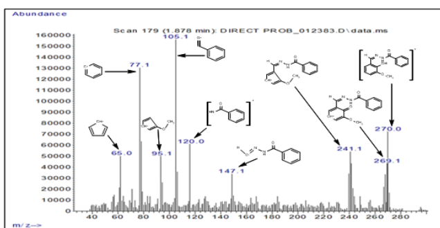
Figure (17) Mass spectra of the complex (3b).
