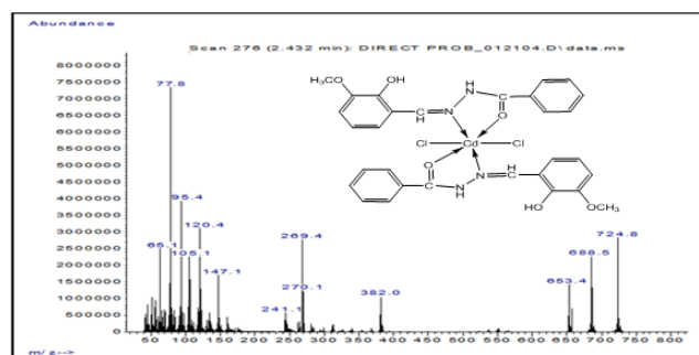
Figure (14) Mass spectra of (L 2 ).
