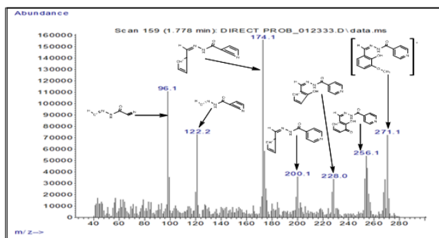
Figure (16) Mass spectra of the complex (2b).
