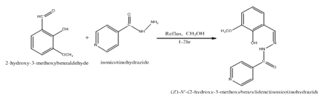
Scheme (1) Formation of Schiff Base Ligand L_1
