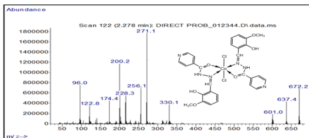
Figure (17) Mass spectra of the complex (3b).
