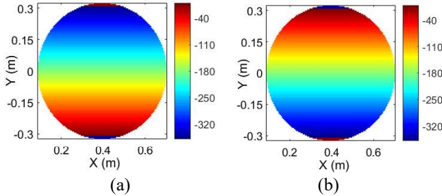
Fig. 9. Phase adjustment (in degrees) on the flat RAS at 19.7 GHz to deviate (a) the X-polarized beam to 0.28^\circ and (b) the Y-polarized beam to -0.28^\circ .
