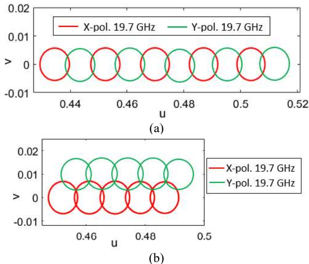
Fig. 7. Contour patterns at -4 dB level for the beams produced at 19.7 GHz by the bifocal DRAAs designed to provide (a) 1.12^\circ beam spacing and (b) 0.56^\circ beam spacing.
