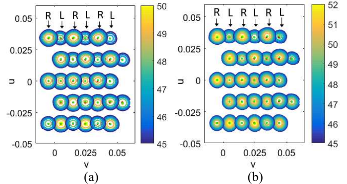
Fig. 10. Gain levels (in dBi) for the multi-spot coverage produced by the DRAA in RHCP (R) and LHCP (L): (a) at 19.7 GHz and (b) at 29.5 GHz.
