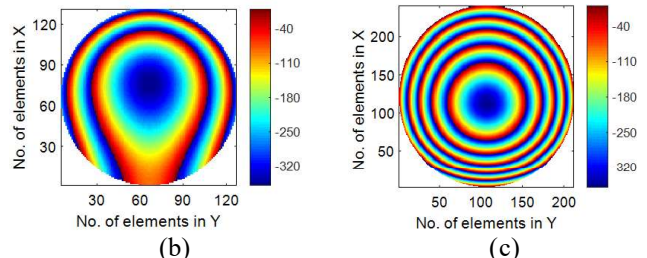
Fig. 6. (a) Dual-offset configuration of the DRAA, including the position of the foci (F1 and F2) and their associated beam directions. Bifocal phase distributions (in degrees) required at 19.7 GHz in X-polarization (b) on the sub-reflectarray and (c) on the main reflectarray.
