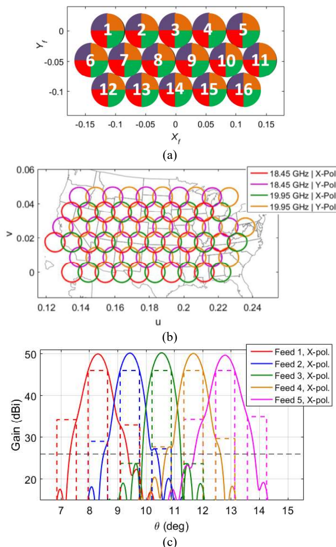
Fig. 3. (a) Configuration with 16 adjacent feed-horns. (b) Contours at 46-dBi gain for the 64 beams produced. (c) Cut of the radiation patterns in the plane ' v = 0 ' for the beams generated at 19.95 GHz in X-pol., including the masks for EOC gain (46 dBi), maximum interference levels of each beam, and the single-entry C/I target (20 dB below the EOC gain).
