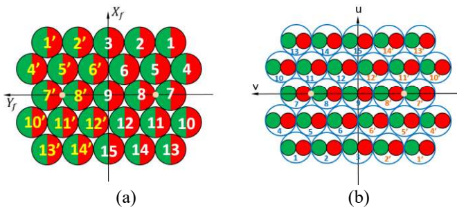
Fig. 4. (a) Configuration with 27 adjacent feed-horns and (b) the 54 beams generated (two beams per feed), using a different color for the orthogonal polarizations.
