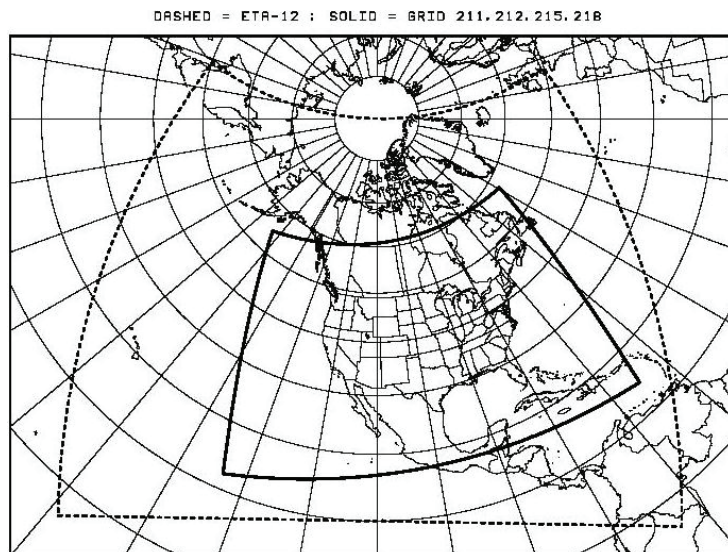
Figure 18. Domain of Lambert conformal NAM model grid #218 (solid line).
