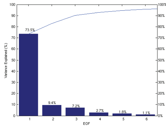
Figure 23. Percentage of the total variance in the seasonal anomalies of the low-pass filtered NAM 3-h wind stress forecasts captured by each EOF mode. EOFs were calculated over the two years from March 2003 through February 2005 for those measurements made at the same times as the measurements used in the calculation of the surface current EOFs.
