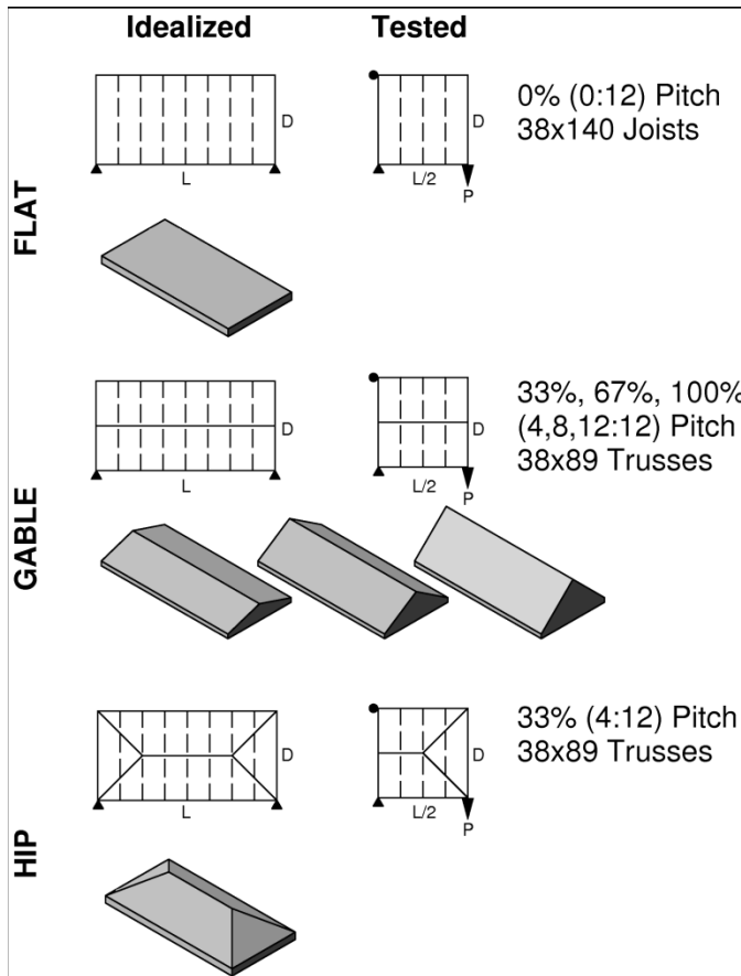
Figure 1. Test specimens.
