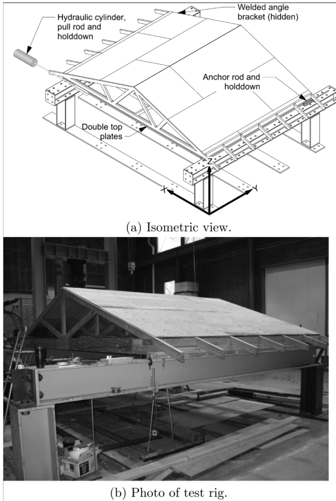
Figure 2. Test rig diagram and 33% (4:12) test sample without eaves.
