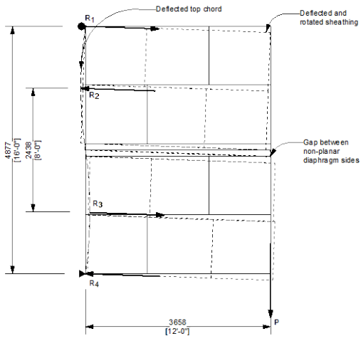
(c) Forces developed in tested roof.
