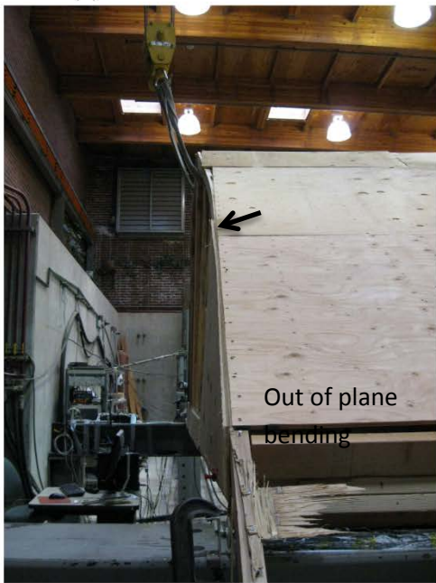
(b) East end from NE corner.
