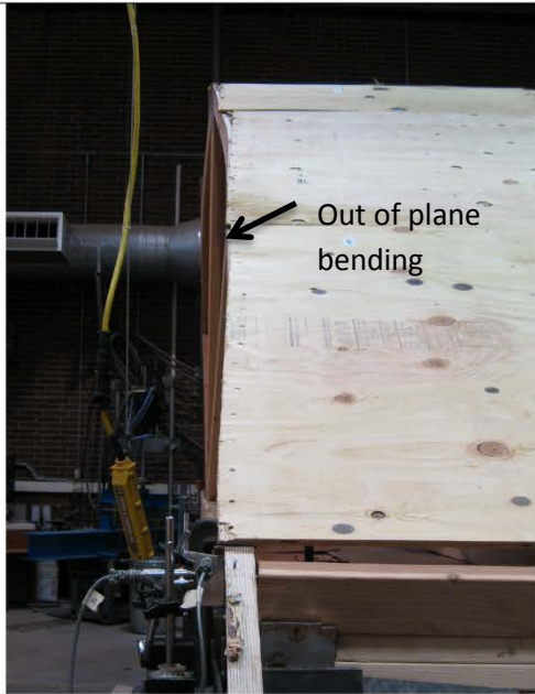
(a) West end from SW corner.
