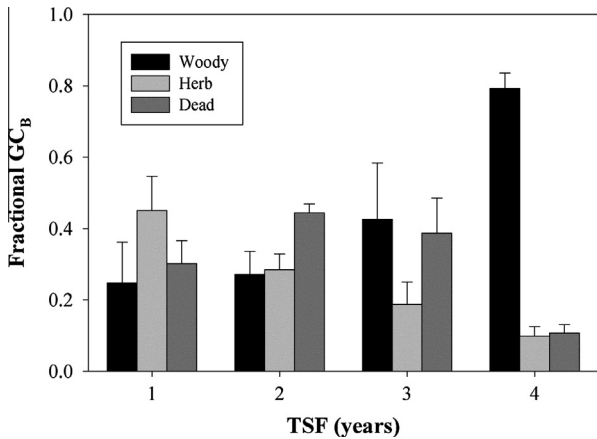
Fig. 4. Model fit to estimate ground cover biomass recovery from time since last prescribed fire (TSF) after fire as a proportion of initial biomass.
