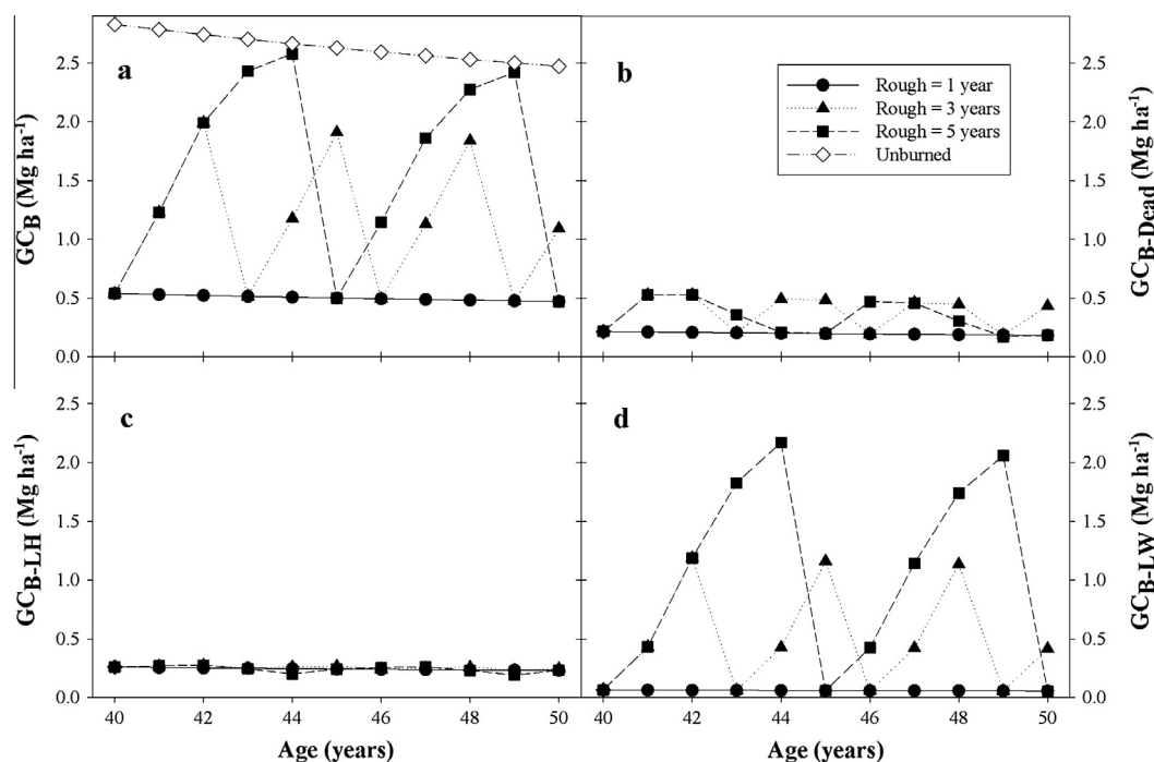
Fig. 9. Simulated effect of prescribed burning frequency on (a) total ( GC_B ), (b) dead ( GC_{B-Dead} ), (c) living herbaceous ( GC_{B-LH} ) and (d) living woody ( GC_{B-LW} ) ground cover biomass. Prescribed burning was initiated at age 40 years with a frequency of 1 (filled circle), 3 (filled triangle), or 5 (filled square) years. In (a) GC_B for unburned stands is also shown (open diamond).
