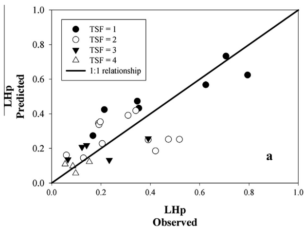
Fig. 5. Relationship between observed and predicted (a) ratio of living herbaceous (LHp) and (b) ratio of living woody (LWp) to total ground cover biomass for different time since last prescribed fire (TSF) for longleaf pine stands in Georgia, Louisiana and North Carolina.
