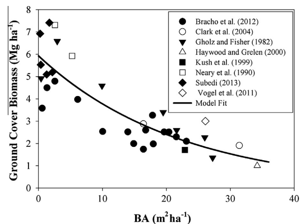
Fig. 2. Relationship between overstory basal area (BA) and ground cover biomass (GCB) for southern pine stands without periodic prescribed burning.
