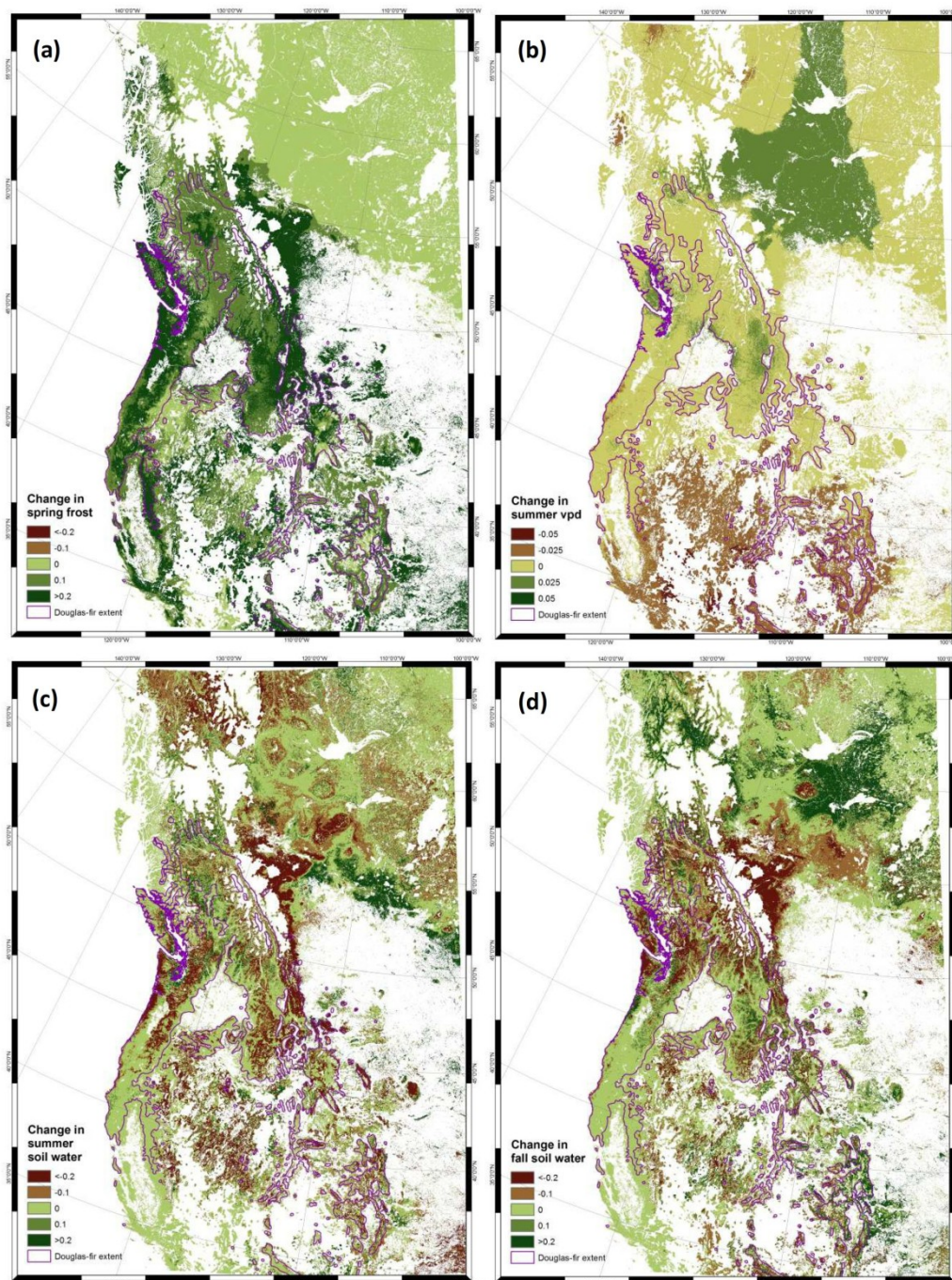
Figure 3. Modeled average changes from 2000 to 2009 in (a) spring frost frequency, (b) summer evaporative demand, (c) summer soil water stress and (d) fall soil water stress compared to the cooler and wetter period (1950–1975). The units represent the proportional change in environmental constraints on GPP in reference to the first period. The range of Douglas-fir is from [28].
