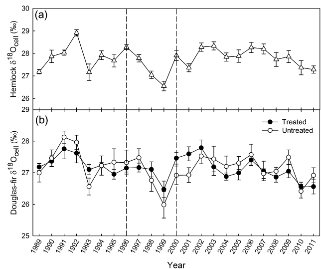
Figure 5. Mean tree-ring \delta^{18}O_{\text{cell}} of western hemlock (a), and fungicide-treated and untreated Douglas-firs (b) at the Beaver, Oregon site during the years of observation (1989–2011; n = 6 trees per treatment group). The treatment period is indicated by vertical dashed lines (1996–2000, inclusive). Bars represent 1 SE.
