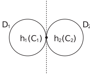
FIGURE 2. Wedge of Cantor sets
