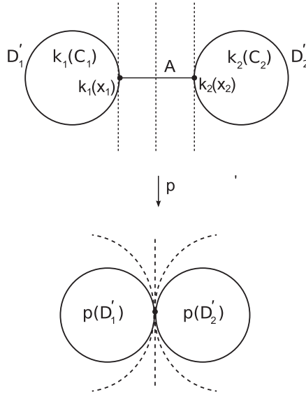
FIGURE 3. Alternate construction for wedge
