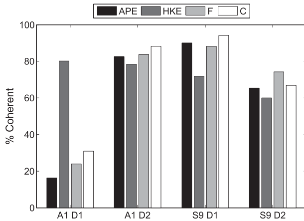
FIG. 15. Percent coherence of internal tides at A1 and S9 in both frequency bands, computed via Eq. (32).
