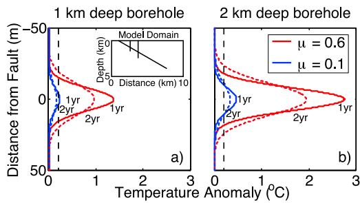
Figure 1. Frictional temperature anomalies in the absence of fluid circulation resulting from a thrust earthquake with 5 m of slip on a fault with 30° dip and assuming a thermal diffusivity of 10^{-6} \text{ m}^2 \text{ s}^{-1} . The separate curves illustrate how a temperature anomaly from frictional heating evolves as a function of time and depth for both large and small coefficients of friction during slip assuming hydrostatic pore pressure. (a) Temperature anomalies for a borehole intersecting the fault at a depth of 1 km. The vertical axis represents the perpendicular distance from the fault zone. Red and blue lines correspond to friction coefficients of 0.6 and 0.1, respectively, assuming hydrostatic pore pressure. Solid and dashed lines show the frictional heating anomaly 1 and 2 years after the earthquake, respectively. The dashed vertical black line shows a conservative detection threshold of 0.2°C. (b) Temperature anomaly for a borehole intersecting the fault at a depth of 2 km.
