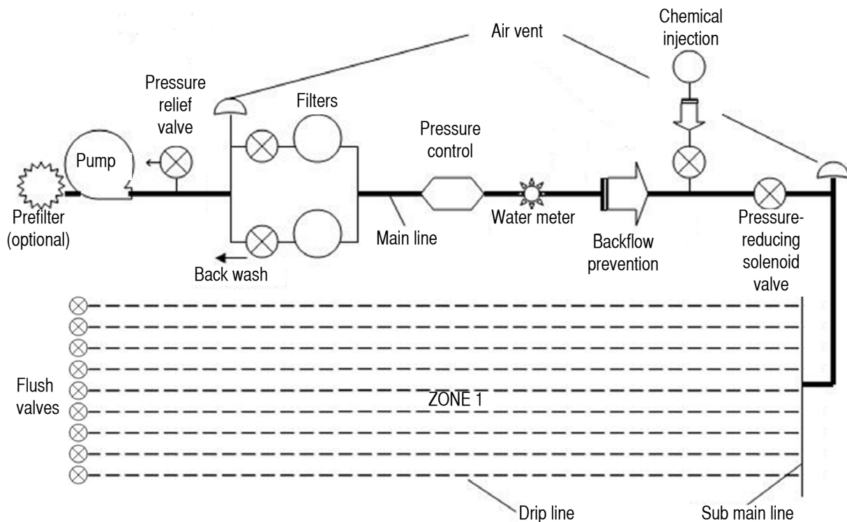
Figure 2. Drip irrigation system with a prefilter, pump station with backflow prevention, and chemical injection site. A pressure control valve is recommended to adjust the water pressure as desired before it enters the drip lines. A water meter can be placed after the pressure control or between a solenoid valve and each zone. An air vent provides vacuum relief. Vacuum relief is necessary between the solenoid valve and the drip tapes to avoid suction of soil into the emitters when the system is shut off.
