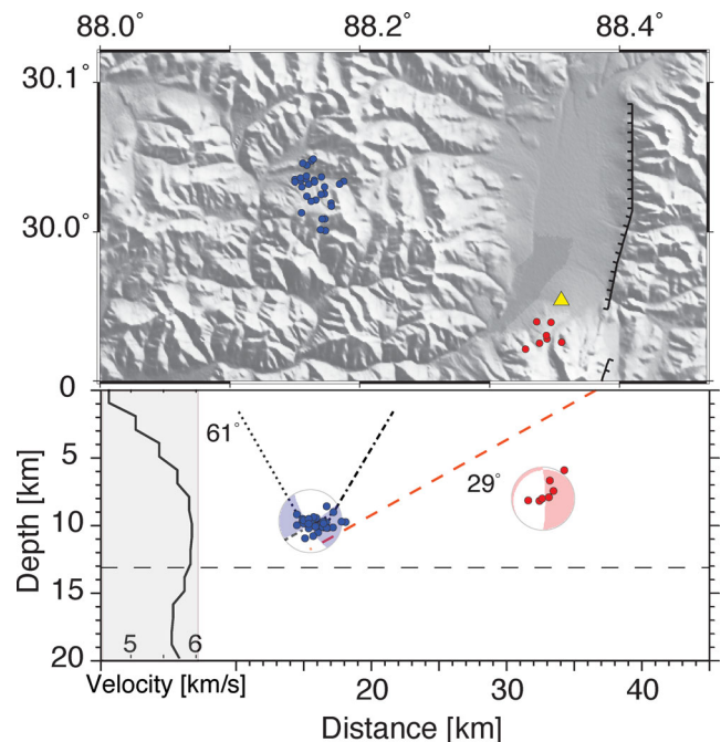
Figure 3. Shaded relief map highlighting topography (top panel) and possible tectonic interpretations (bottom panel). Highest quality hypocentres (best geometrical coverage) follow Fig. 2 colour scheme. Receiver function velocity model from Nabelek et al. (2009) is embedded to the left within profile view. Horizontal black dashed line marks the top of the low-velocity zone, likely corresponding to base of the seismogenic upper crust. Possible faulting interpretations illustrated: planar 29^\circ west dipping low-angle fault surfacing at the PXR east wall (red dashed line), west dipping listric fault (black dash-dotted line), and planar high-angle 61^\circ east dipping fault (black dotted line). Only the 29^\circ west dipping fault interpretation is associated with a surface expression.
