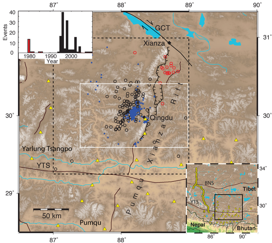
Figure 1. Map of the Pumqu-Xianza Rift. PXR fault scarps were identified from satellite imagery; tick marks indicate clear hangingwall slip directions. Gyaring Co Transform fault (GCT) and Yarlung-Tsangpo Suture (YTS) are also plotted. Nearby HiCLIMB seismic stations indicated by yellow triangles. International Seismological Center (ISC) earthquake locations are shown as open circles (red: 1980s, black: 1994–2012). Blue dots are epicentres from the Carpenter et al. (2010) HiCLIMB catalogue within the black-dashed box. Black diamonds are towns. White box is area of Fig. 2. Upper inset shows histogram of ISC reported ( m_b \geq 4.0 ) seismicity. Lower inset shows HiCLIMB phase-2 stations; YTS and BNS (Bangong-Nujiang Suture) bound the Lhasa Block. Black box shows the area of the main figure.
