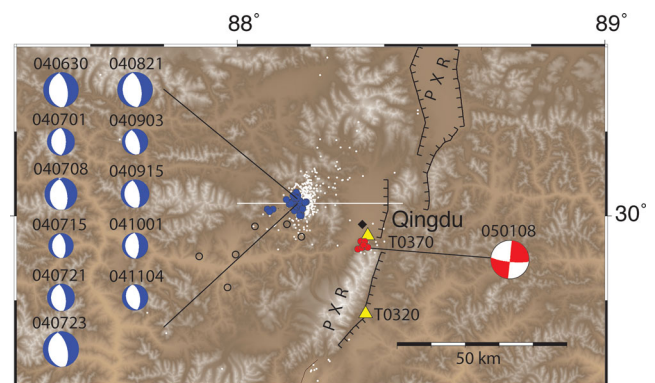
Figure 2. Epicentres for manually located earthquakes, blue for events west of the Qingdu segment and red for events near station T0370. White dots are epicentres from the Carpenter et al. (2010) HiCLIMB catalogue. White line shows profile location for Fig. 3. Fault plane solutions from RMT analysis are identified by event date (YYMMDD) and colour-coded by faulting type. Complete results are provided in the electronic supplement. Telesismic ISC locations for six earthquakes (black circles) relocate into the blue cluster. Delineated faults are as in Fig. 1.
