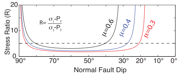
Figure 4. Ratio of effective principal stresses ( R ) for reactivation of a cohesionless fault plotted against normal fault dip (after Colletini & Sibson 2001) for vertical principal stress ( \sigma_1 ). For normal friction, \mu = 0.6 , a fault dipping \leq 30^\circ is completely locked and cannot move; slip on faults dipping between 30^\circ and 40^\circ requires high stress ratios making slip less likely as dip decreases. A reduction to \mu = 0.3 – 0.4 is necessary to accommodate slip along faults with 22^\circ – 33^\circ dip. Dashed line indicates approximate dip limit for active slip, about 40^\circ under normal conditions ( \mu = 0.6 ), as indicated by global observations.
