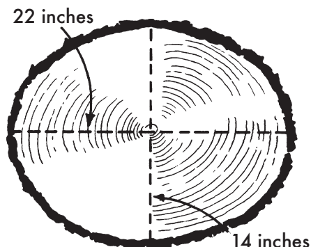
Figure 5. Method of measuring the diameter of oval logs: add 22 to 14 and divide by 2; the diameter is 18 inches.
