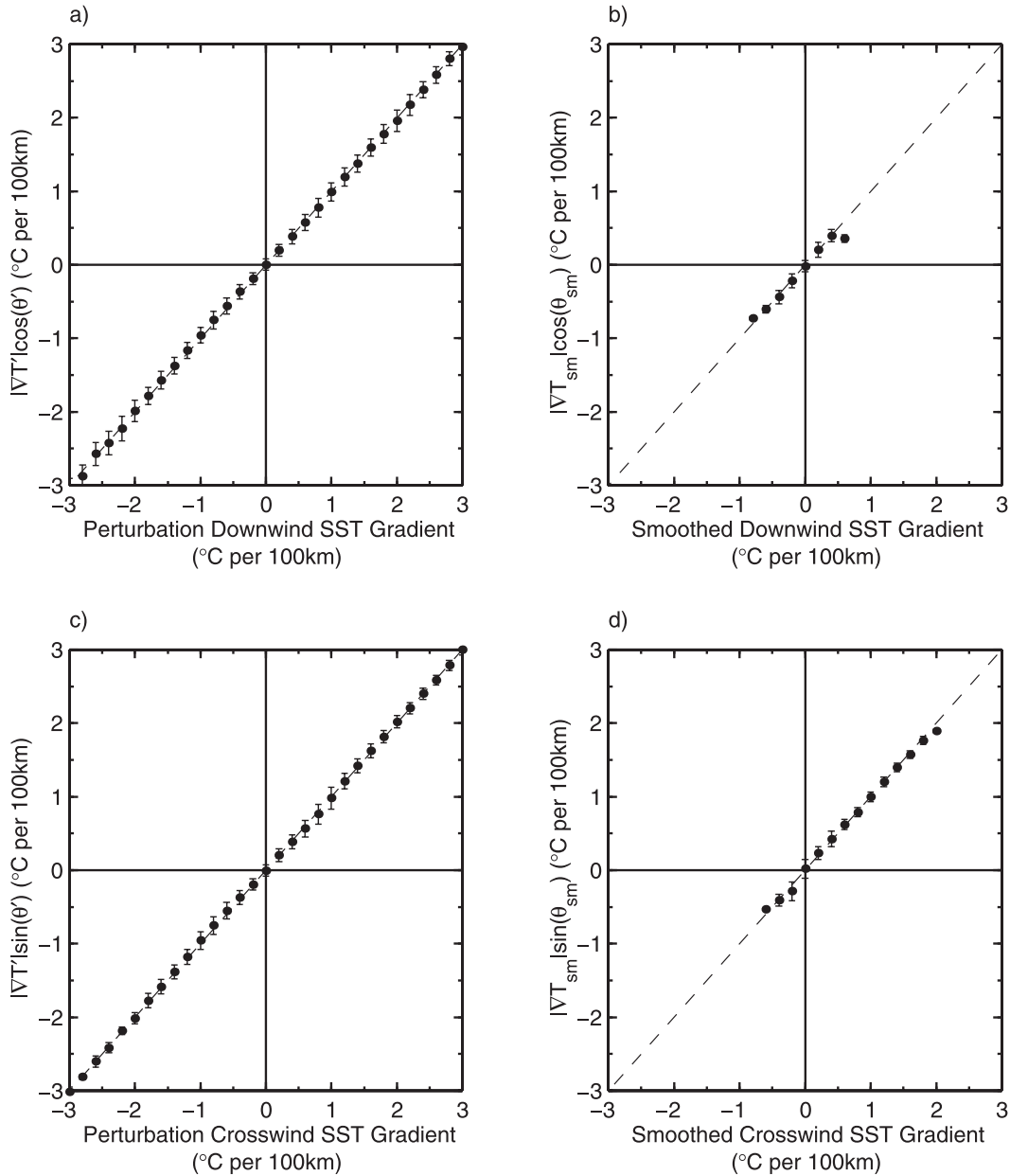
FIG. A1. Binned scatterplots of the relations expressed by Eqs. (A5)–(A8). (a) |\mathbf{V}T'| \cos\theta' vs. (\partial T/\partial s)' ; (b) |\mathbf{V}\tilde{T}'| \cos\tilde{\theta}' vs. (\partial\tilde{T}/\partial s)' ; (c) |\mathbf{V}T'| \sin\theta' vs. (\partial T/\partial n)' ; (d) |\mathbf{V}\tilde{T}'| \sin\tilde{\theta}' vs. (\partial\tilde{T}/\partial n)' . The points and error bars in each panel represent the means and \pm 1 std dev within each bin computed from the first monthly averaged AMSR-E SST and QuikSCAT wind fields used in this study over the Agulhas Return Current. The dashed line in each panel has unit slope and is shown for reference.
