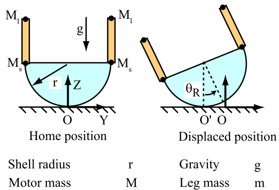
Fig. 8 RRRobot's roll freedom (side view).
