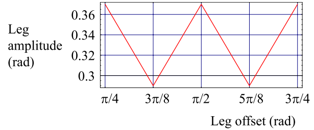
Fig. 20 Amplitude modulation used in the decoupled yaw model.
