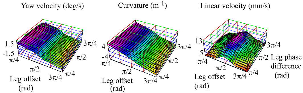
Fig. 19 RRrobot translation as a function of offset and leg phase difference as predicted using the decoupled models (compare with Fig. 18)
