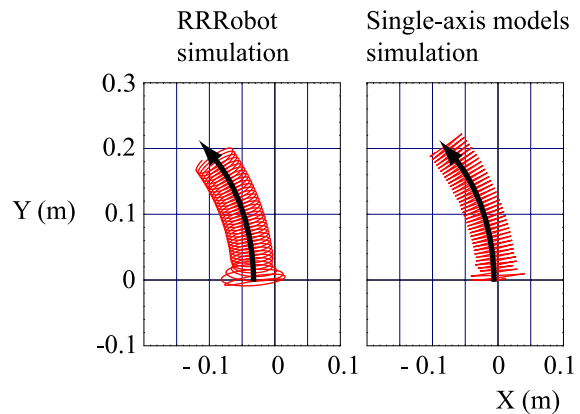
Fig. 16 The circular translation gait: comparison of RRRobot's motion with motion predicted by the single-axis models over thirty seconds. Leg 1 trajectory: \pi/4 + 0.3 \sin(8t) , and leg 2 trajectory: \pi/4 + 0.3 \cos(8t) .
