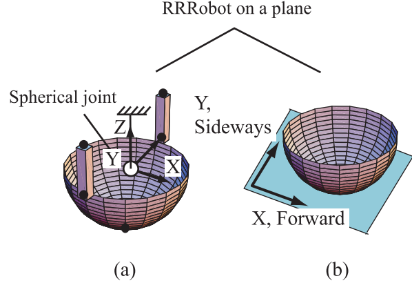
Fig. 3 The Pivoting Dynamics model simplifies the RRRobot-on-a-plane model (see Figure 1) into two parts: (a) RRRobot pivoted at its geometric center on a spherical joint and (b) a sphere on a plane.
