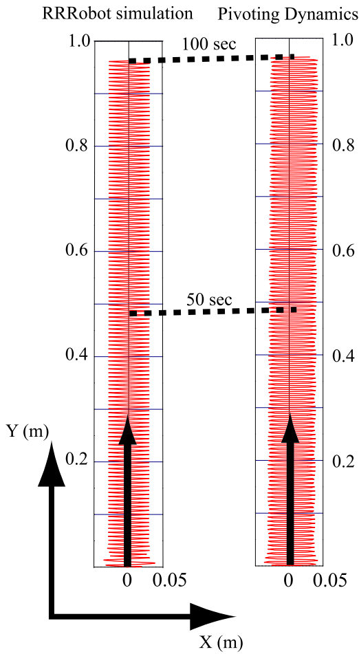
Fig. 6 Planar plots of contact-point time profile during sideways locomotion produced by Gait 1 in RRRobot-on-a-plane simulation and Pivoting Dynamics simulation. The solid arrow gives robot motion direction, and the dotted lines indicate the robot position at the specified time.
