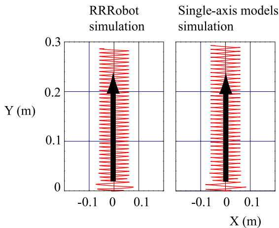
Fig. 15 The lateral translation gait: comparison of RRRobot's motion with motion predicted by the single-axis models over thirty seconds. Leg 1 trajectory: \pi/2 + 0.3 \sin(8t) , and leg 2 trajectory: \pi/2 + 0.3 \cos(8t) .
