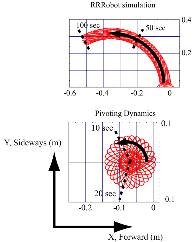
Fig. 7 Planar plots of contact-point time history during counter-clockwise circular locomotion produced by Gait 2 in RRRobot-on-a-plane simulation and Pivoting Dynamics simulation. The solid arrow gives robot motion direction, and the dotted lines indicate the robot position at the specified time.
