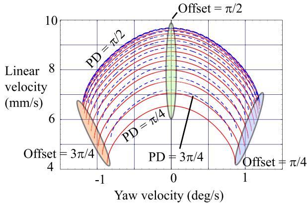
Fig. 21 Mapping between RRrobot linear velocity and yaw velocity and leg offset and phase difference (PD).
