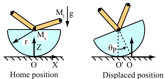
Fig. 9 RRRobot's pitch freedom (side view).
