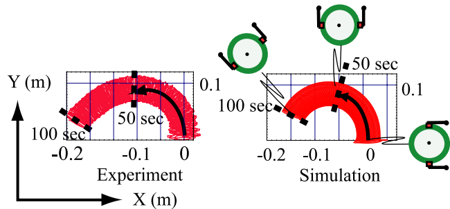
Fig. 2 The path traced by a legless locomotion gait (sinusoidal leg motions) that produces counter-clockwise translation through body roll-pitch-yaw oscillations [16]. The broad red patch is a result of the back-and-forth pitch oscillations. The figure also shows RRRobot’s changing orientation over time.
