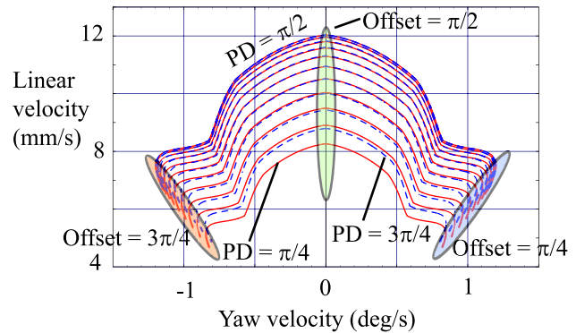
Fig. 22 Mapping between RRrobot linear velocity and yaw velocity and leg offset and phase difference (PD) as predicted by the decoupled models.
