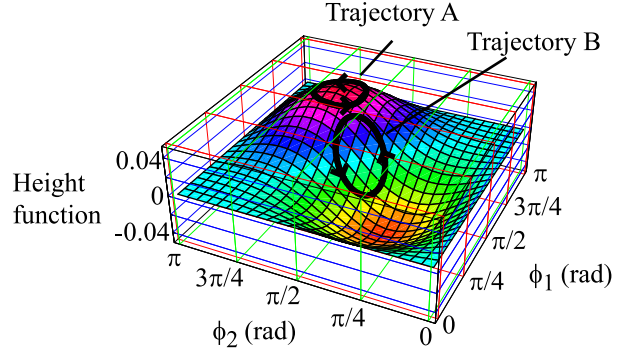
Fig. 13 Yaw model height function. Trajectory A (leg 1: 5\pi/8 + 0.15 + 0.3 \sin(8t) and leg 2: 5\pi/8 + 0.15 + 0.3 \cos(8t) ) produces net body yaw, while trajectory B (leg 1: \pi/2 + 0.3 \sin(8t) and leg 2: \pi/2 + 0.3 \cos(8t) ) does not produce net yaw.
