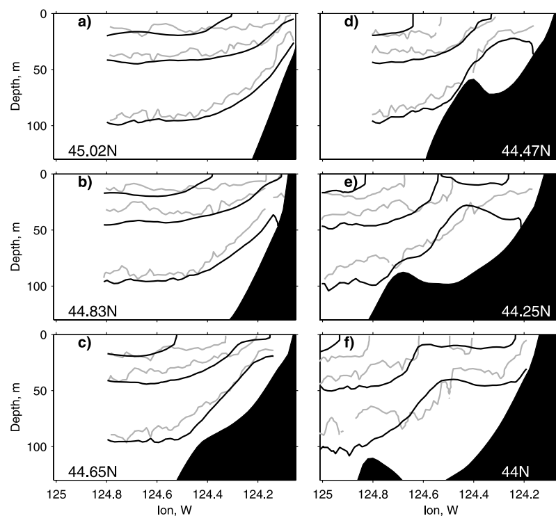
Figure 4. Contours of potential density \sigma_{\theta} = 24, 25, and 26 \text{ kg m}^{-3} in vertical sections of the SeaSoar survey Big Box 1 (BB1) (days 144.4–145.8). SeaSoar data are half-toned, and modeled contours (no DA) are black.
