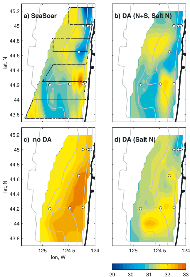
Figure 17. Salinity (psu) at 5 m depth during SeaSoar survey BB5, days 162.2–164.3: (a) SeaSoar data, with the cruise track (dotted line) originating in the southeast; (b) solution DA (N+S, Salt N); (c) no DA solution; (d) DA (Salt N). Model maps are plotted using the same sampling strategy as the SeaSoar survey. Bathymetry contours are at 50, 100, 200, and 1000 m. Circles show mooring locations.
