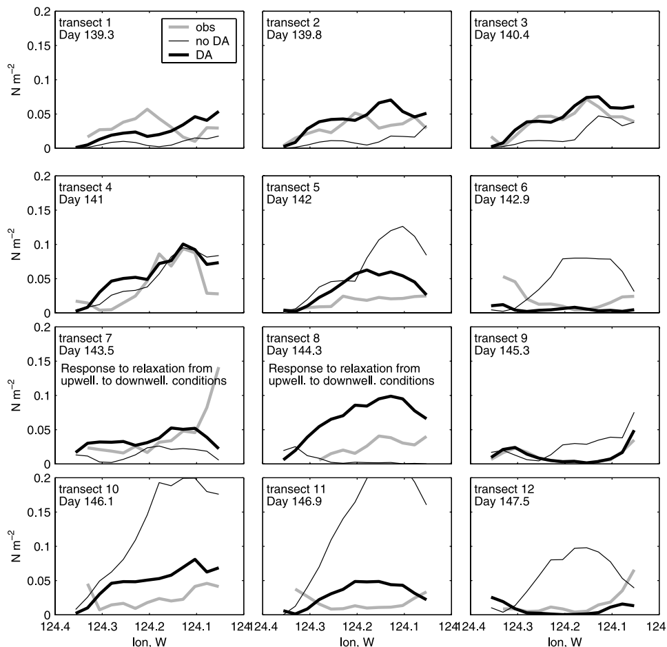
Figure 20. Bottom stress magnitude at 45^{\circ}\text{N} from turbulence microstructure observations (shaded lines), model without DA (thin lines), and case DA (NMS+NIS) (bold lines). Model-data statistics are given in Figure 21.
