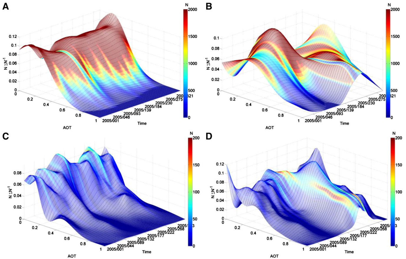
Fig. 6. Variation in aerosol optical thickness (AOT) over a northern (7°30' N, 70° W, Figure A) and a southern (7°30' S, 70° W, Figure B) subset of the study area (size 500 × 500 km 2 each). The x-axis represents the time (year 2005), the y-axis shows AOT bins (width 0.01) and the z-axis represents counts per AOT bin (as fraction of total number of observation at a particular time). The color corresponds to the total number of observation at a particular time. Figures C and D show the same AOT estimates, but derived from MYD04 at 10 km resolution.
