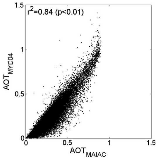
Fig. 7. Comparison between MAIAC AOT and MYD04 for the entire study area (MAIAC data were resampled to 10 \text{ km}^2 to match the MYD04 resolution) between 2002 and 2010, filtered by both, the MYD35 and MAIAC cloud masks.
