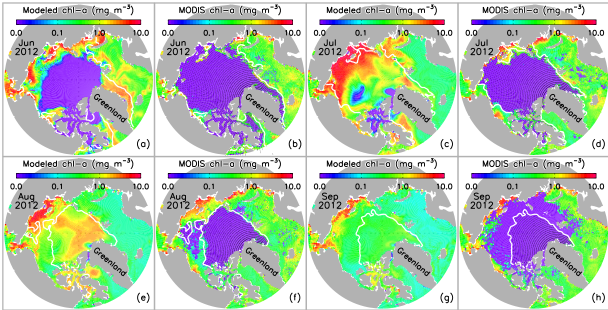
Figure 4. Model (CNTL)-simulated monthly mean and MODIS-Terra observed monthly composite surface concentration of chl a for June to September 2012. The white line represents satellite observed ice edge defined as 0.15 ice concentration. There are no MODIS chl a data under ice (dotted areas). MODIS chl a data are available from http://oceancolor.gsfc.nasa.gov/ . Satellite ice concentration data are from http://nsidc.org/data/nsidc-0081.html .
