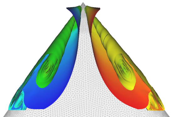
Figure 8: The formation of vortices at the apex of a delta wing illustrated with the use of a stream surface. Image courtesy of C.Garth et al. [GTS*04].
