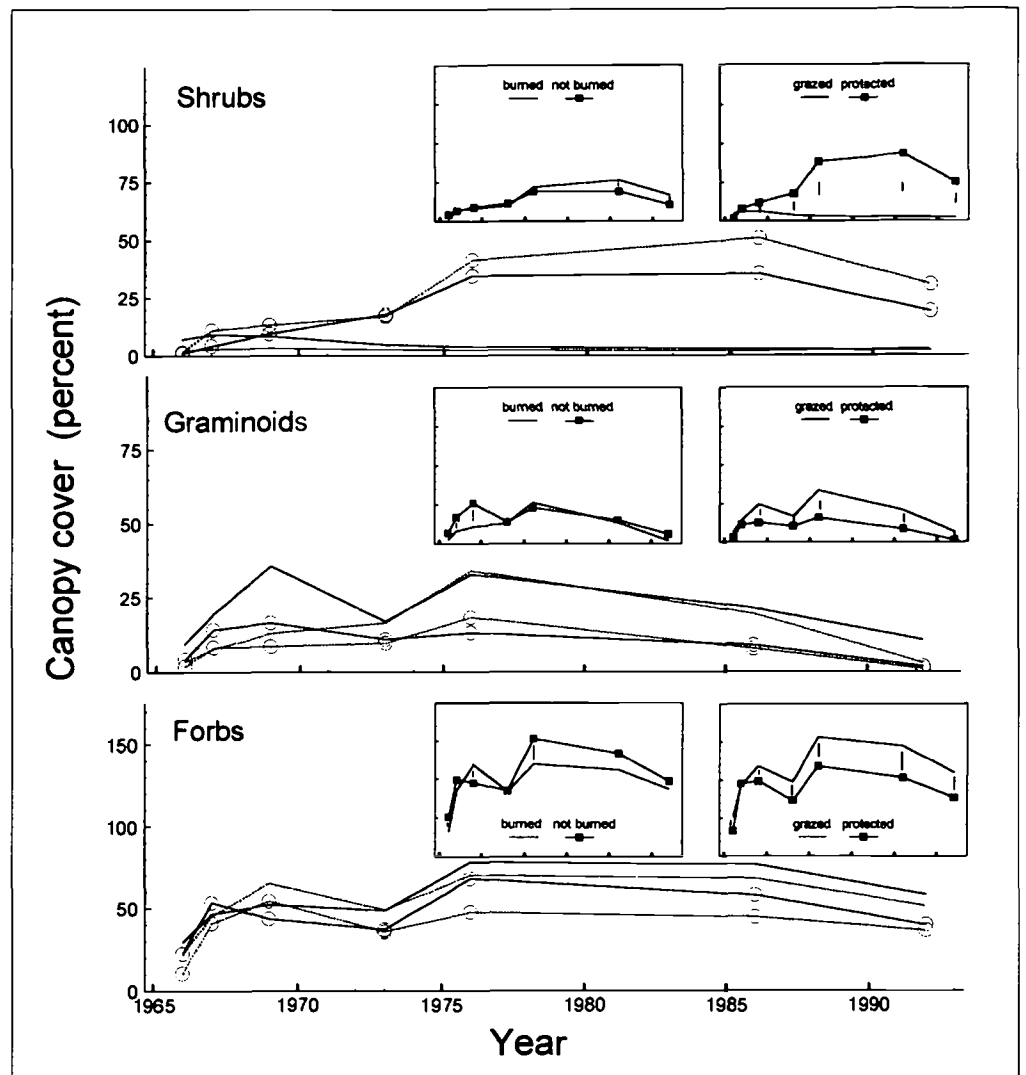
Figure 5—Aggregate canopy cover for shrubs, graminoids, and forbs in the Mottet clearcut: burn, graze (.....); burn, protect (---○---); no burn, graze (—○—); and no burn, protect (—○—). Inset graphs contrast the observed influence of burning with that of herbivory. Vertical bars in the inset approximate year-specific LSD_{0.05} values for significant differences between means.
