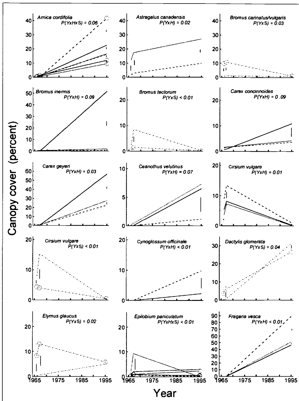
Figure 10—Cover trajectories for Hall Ranch taxa exhibiting Y \times S \times H effects (cattle only, no seed .....; cattle only, seed --○--; dual use, no seed ---; dual use, seed --○--; game only, no seed —; game only, seed —○—), Y \times H effects (cattle only .....; dual use ---; game only —), and Y \times S effects (no seed ----; seed -○-). Vertical bars approximate year-specific LSD values at the significance level indicated in each graph.
