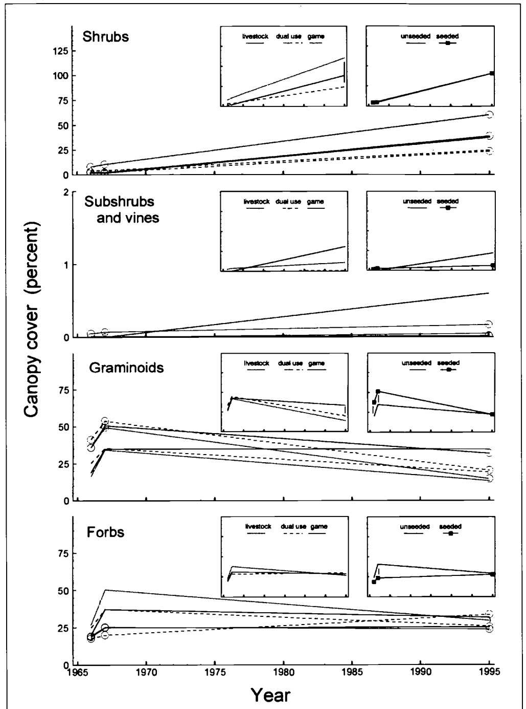
Figure 9—Aggregate canopy cover trajectories for shrubs, subshrubs and vines, graminoids, and forbs, at the Hall Ranch clearcut: cattle only, no seed (---); cattle only, seed (---○); dual use, no seed (---); dual use, seed (---○); and game only, no seed (---); game only, seed (---○). Vertical bars in the insets approximate year-specific LSD_{0.05} values for differences between means.
