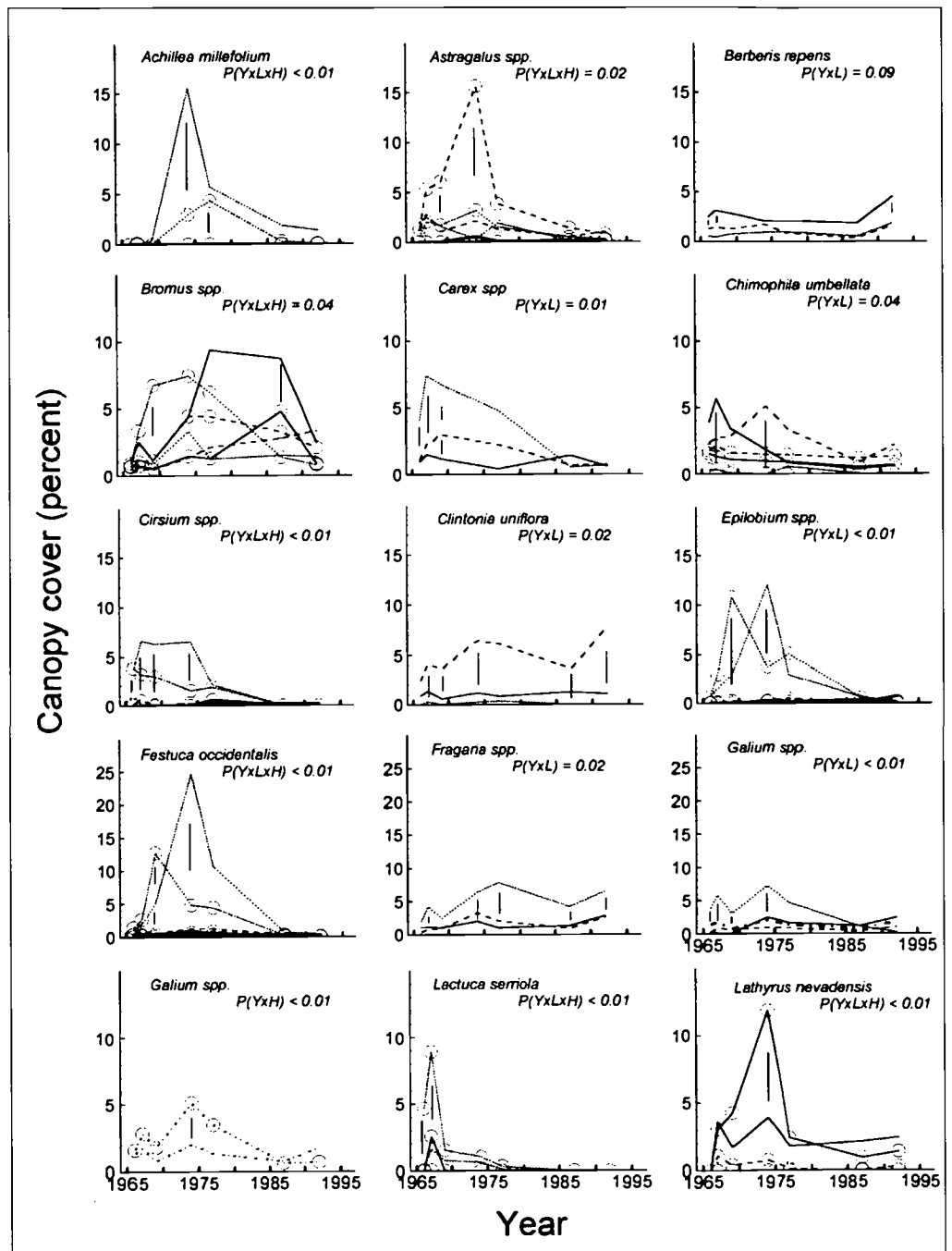
Figure 8—Canopy cover trajectories for Hoodoo taxa exhibiting Y \times L \times H effects (clearcut, graze ----; clearcut, protect -○-; selective cut, graze --; selective cut, protect -○-; no cut, graze —; no cut, protect -○-), for Y \times L effects (clearcut ----, selective cut --, no cut —), and Y \times H effects (graze ---, protect -○-). Vertical bars approximate year-specific LSD values at the significance level indicated in each graph.
