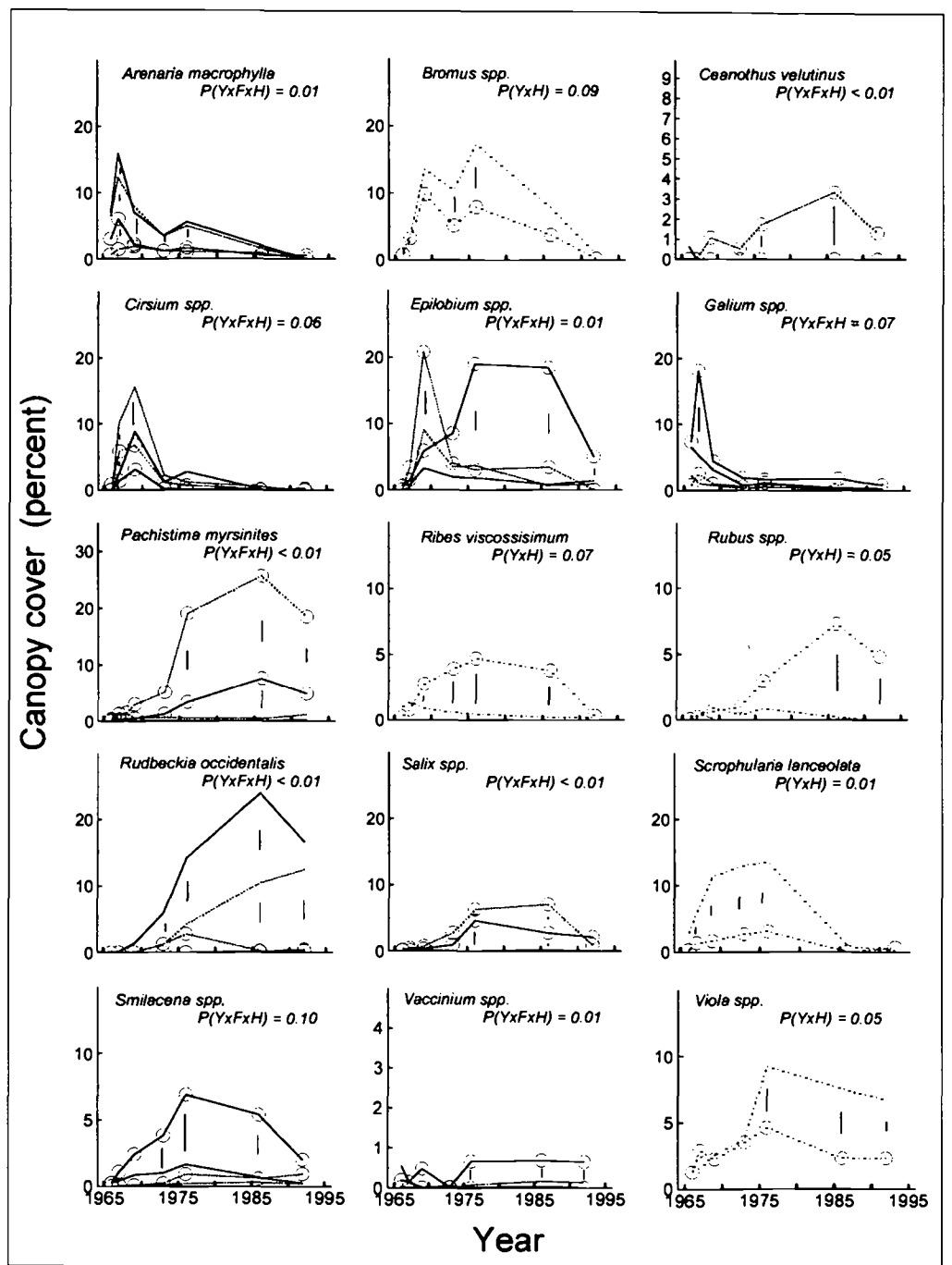
Figure 6—Canopy cover trajectories for Mottet taxa exhibiting YxFxH effects (burn, graze ----; burn, protect--○--; no burn, graze —; no burn, protect —○—). Vertical bars approximate year-specific LSD values at the significance level indicated in each graph.
