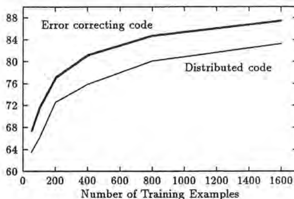
Figure 1: Learning curves showing % phonemes correct for the distributed output code and for the 93-bit error-correcting code (63 phoneme bits with d = 31 , 30 stress bits with d = 15 ).
