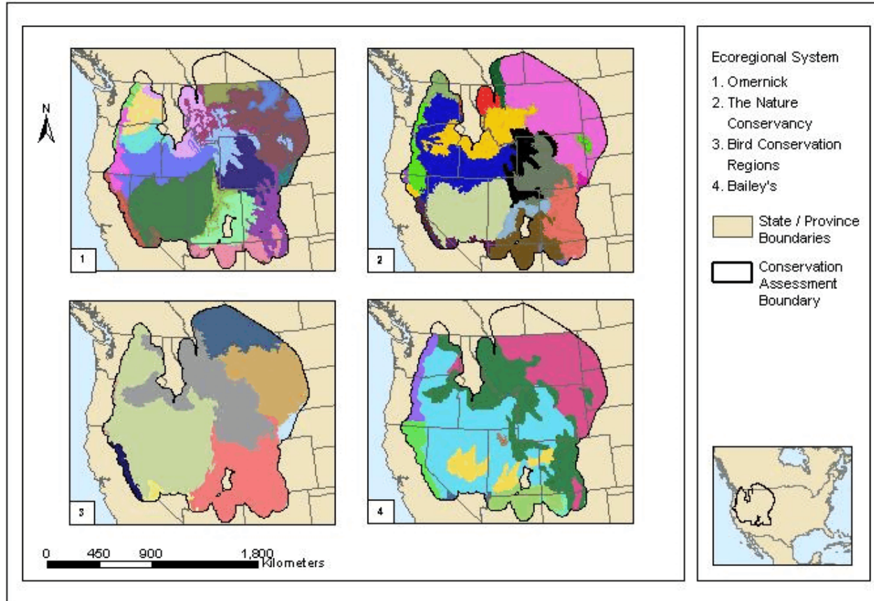
Fig. 1.4. Pre-settlement distribution of sage-grouse with overlays of boundaries for (1) Omernik Regions, (2) The Nature Conservancy ecoregions, (3) Bird Conservation Regions, and (4) Bailey's ecoregions.
