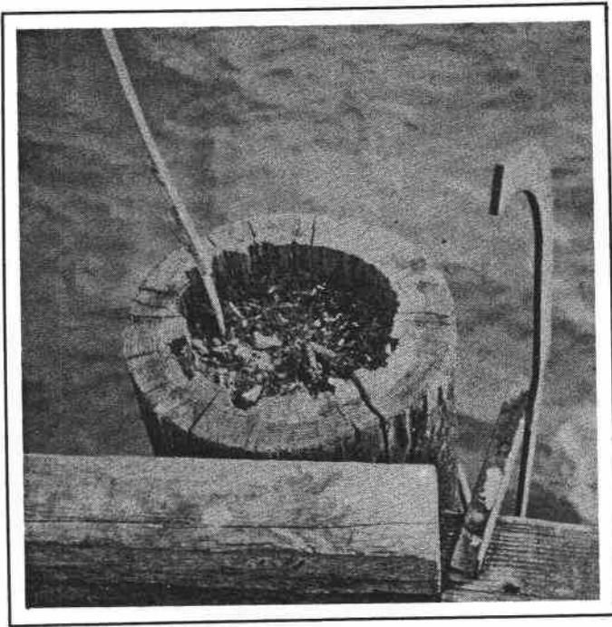
FIGURE 21. THE COMMON COASTAL PRACTICE OF CUTTING THE TOP OFF PRESSURE-TREATED PILING EXPOSES UNTREATED HEARTWOOD TO DECAY FUNGI AND OFTEN RESULTS IN A HOLLOW PILE TOP.
