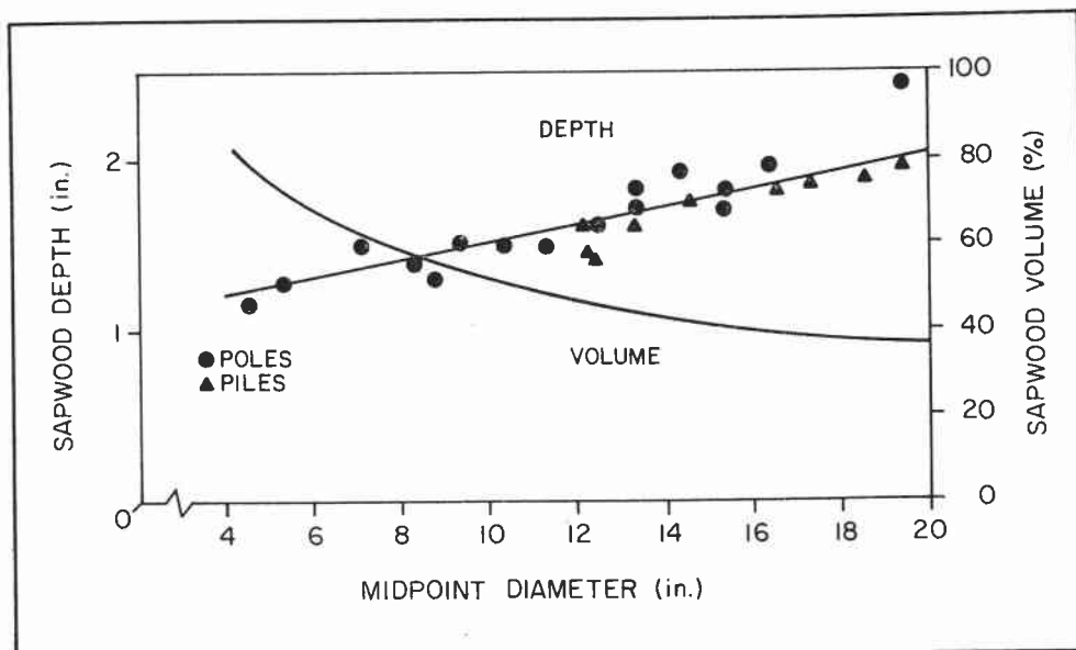
FIGURE 2. VARIATION IN DEPTH AND VOLUME OF SAPWOOD WITH INCREASING POLE DIAMETER OF COAST DOUGLAS-FIR. FROM GRAHAM AND HELSING (1979).
