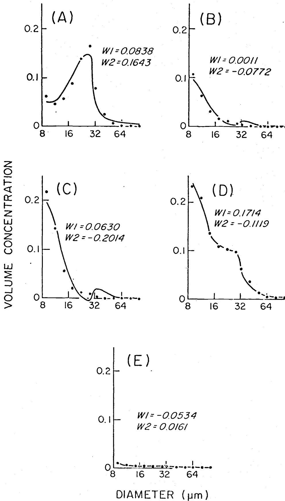
Figure 5. Volume concentration (ppm/m bandwidth) as given by the measured data (dots) and by the characteristic vector representations (lines) for samples taken d km from shore at a depth z, (d,z) as follows: A, (1.85,1); B, (37.1); C, (15.5); D, (9.25); and E, (7.5,20).
