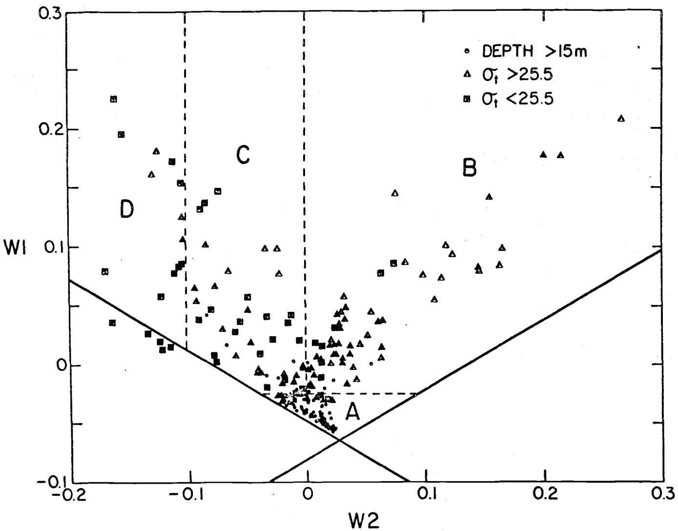
Figure 3. The distribution of the first characteristic vector weighting factors ( W1 ) versus the second characteristic vector weighting factors ( W2 ). Points in region A represent primarily samples taken below the euphotic zone. The other groups are predominantly samples from the top 15 m. Samples from the surface layer are symbol coded according to their sigma-t values.
