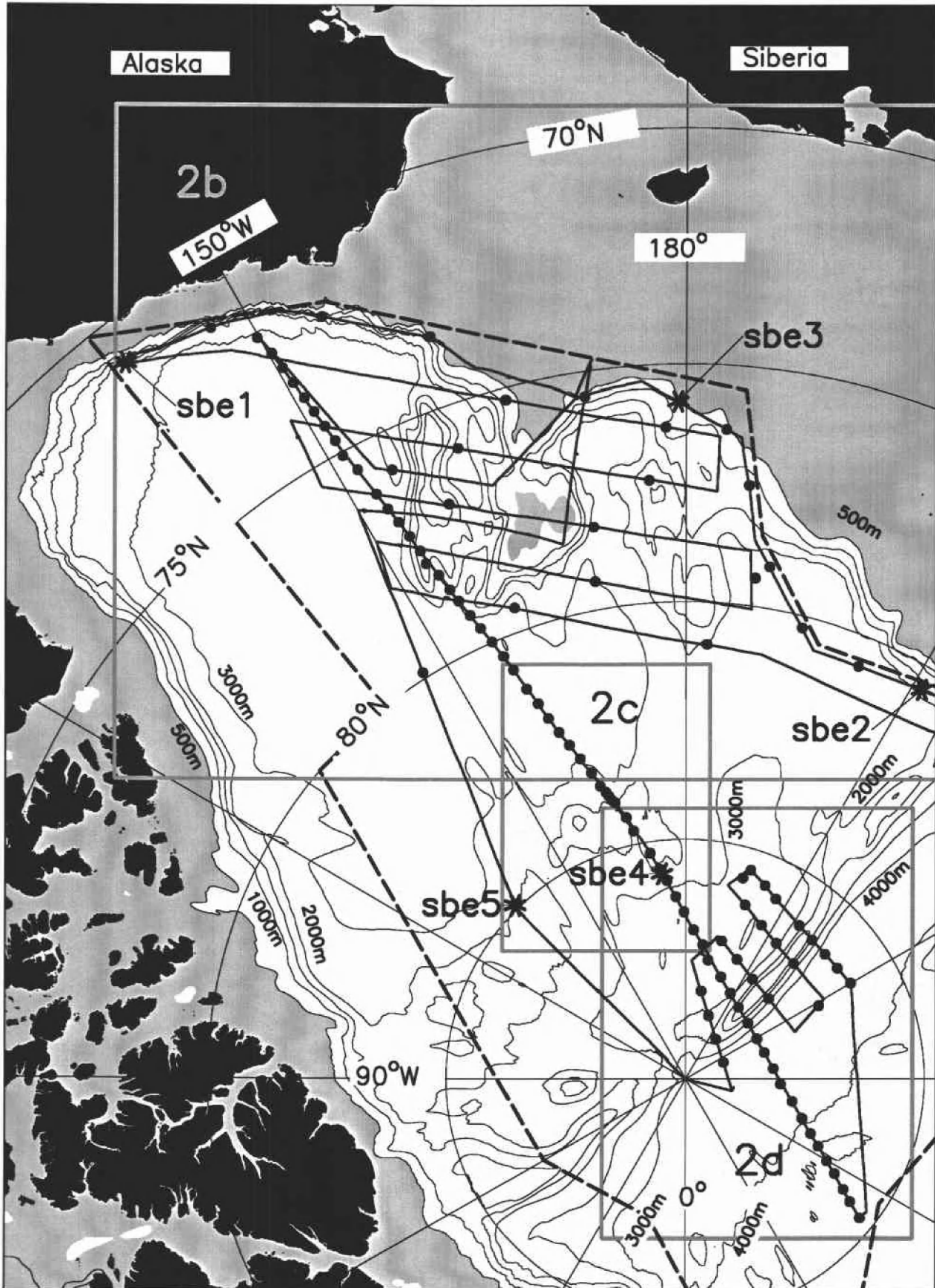
Figure 2a. SCICEX-95 cruise track with XCTD locations and CTD surface stations superimposed. The outlined areas are enlarged in Figures 2b, 2c, and 2d.
