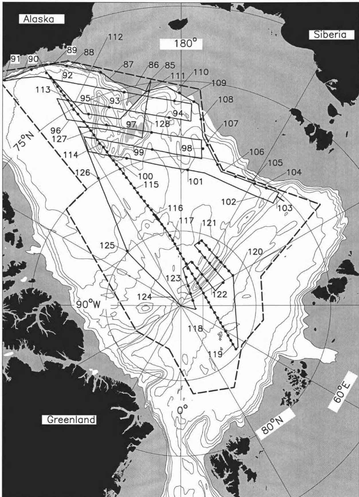
Figure 1. SCICEX-95 cruise track with XCTD locations and 1995 year-days superimposed
