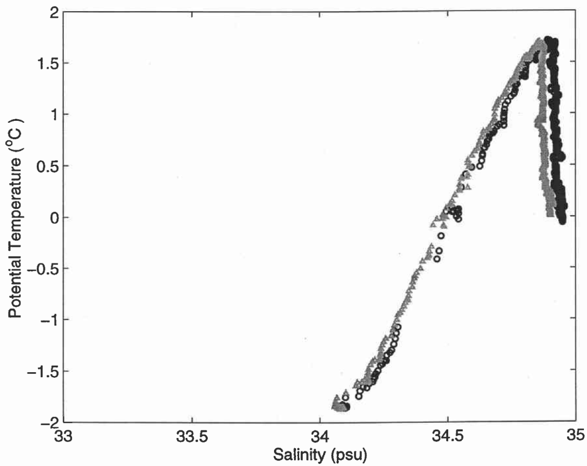
Figure 5b. Potential temperature vs. salinity for XCTD 81 (o) and XCTD 82 ( \Delta )
