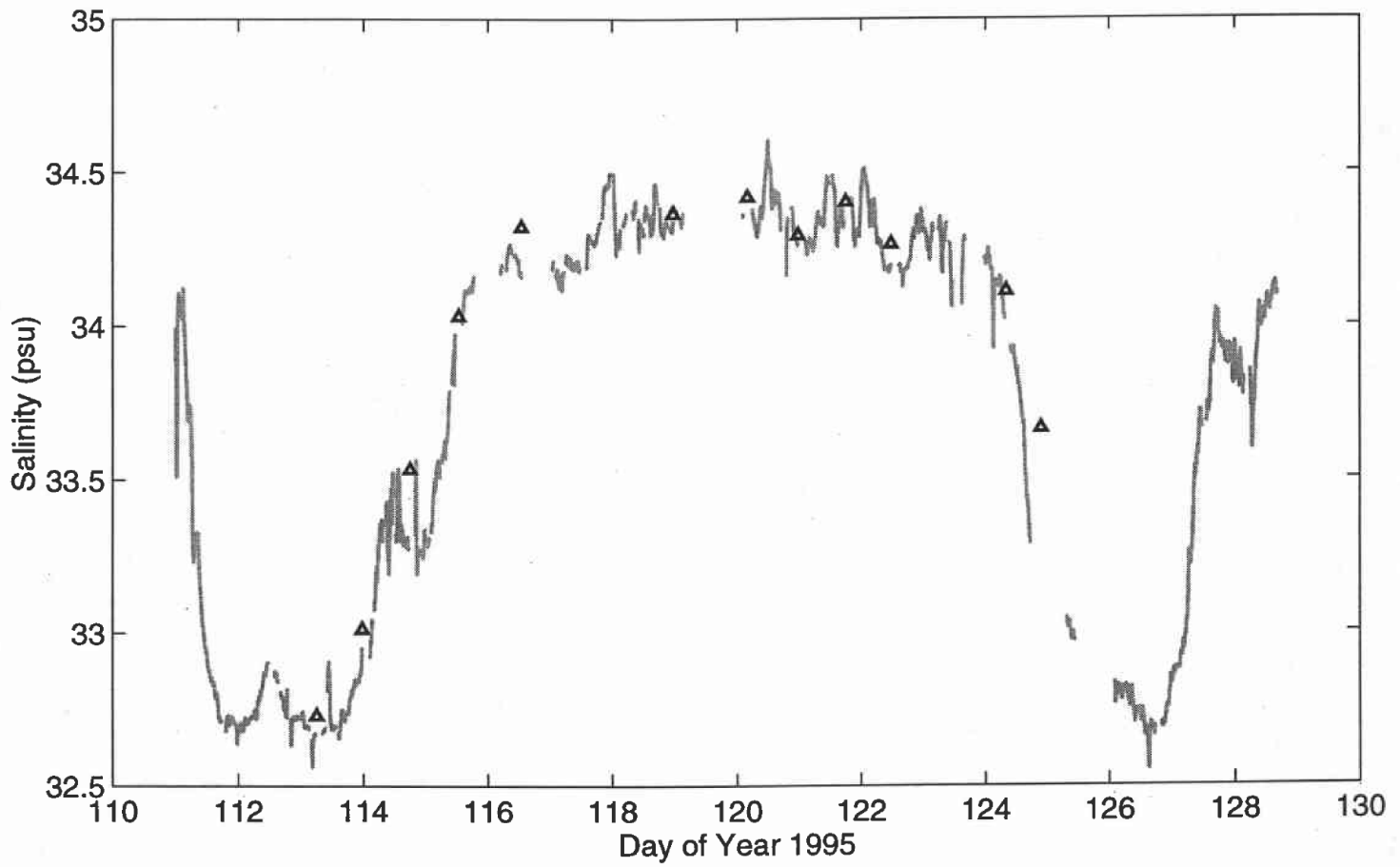
Figure 7. Salinity from the sail CTD at 120 m and bottle samples from 132–134 m
