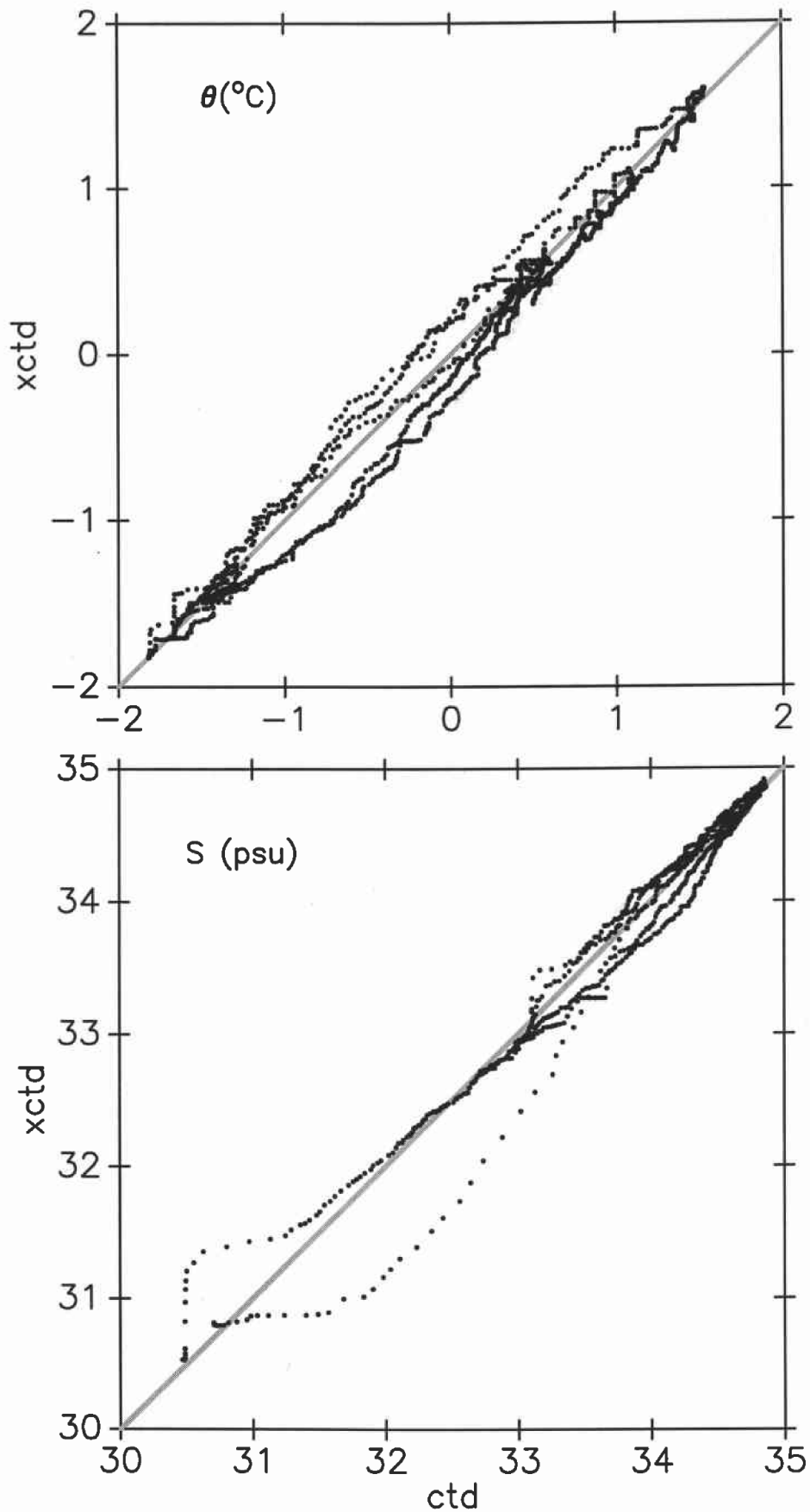
Figure 3c. Scatter plots of temperature and salinity from CTD and XCTD casts, with the XCTDs depth-corrected as an ensemble
