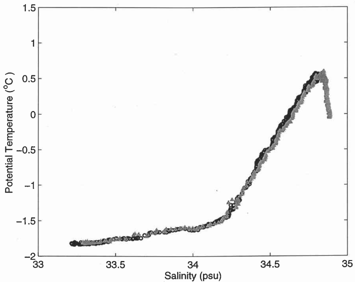
Figure 5a. Potential temperature vs. salinity for XCTD 77 (o) and XCTD 78 ( \Delta )
