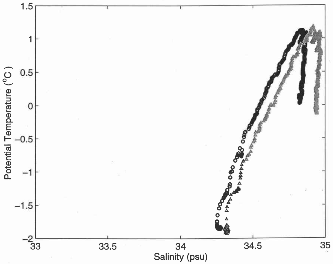
Figure 5c. Potential temperature vs. salinity for XCTD 87 (o) and XCTD 88 (Δ)
