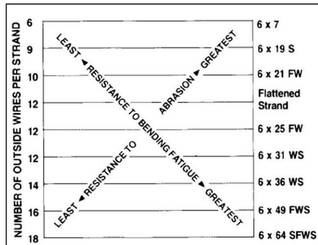
Figure 31 “X” Chart: Wire Rope Bending and Fatigue
