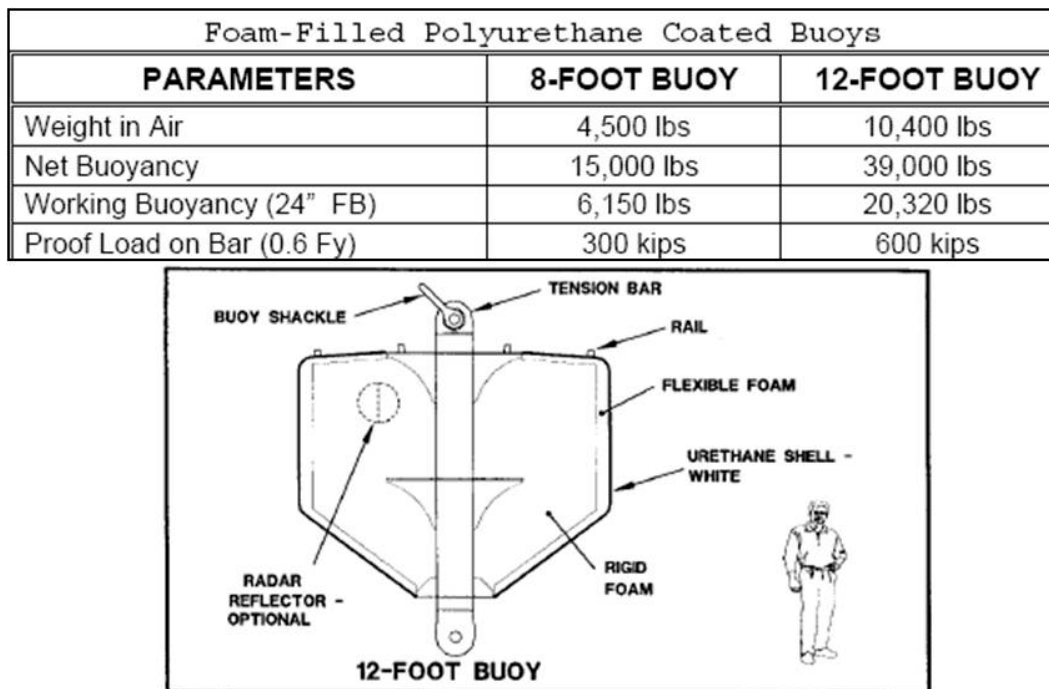
Figure 25 Example US Navy Fleet Mooring Buoy (MIL-HDBK-1026/4A)
