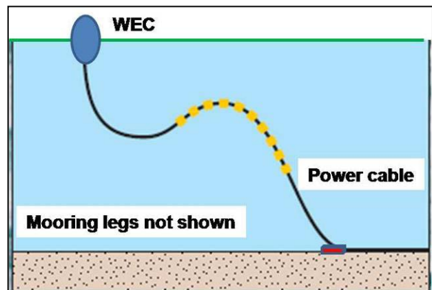
Figure 29 Distributed Cable Buoyancy
