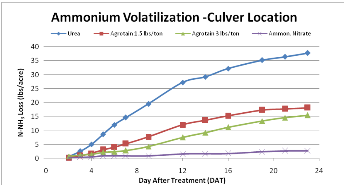
Figure 1. Ammonia volatilization loss from four nitrogen sources at Culver initiated October 12, 2011.
