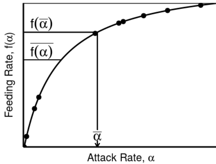
Figure 4.2: The Holling Type II functional response f is a concave function of the attack rate \alpha . Variation among individuals in attack rates causes the average feeding rate among individuals \overline{f(\alpha)} to be less than the feeding rate evaluated at the average attack rate f(\bar{\alpha}) .
