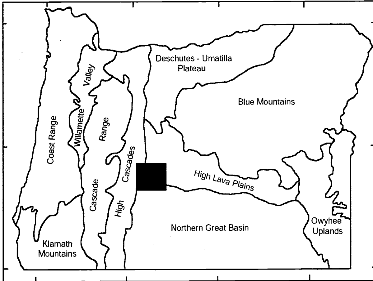
Figure 2.1. Physiographic provinces of Oregon.
