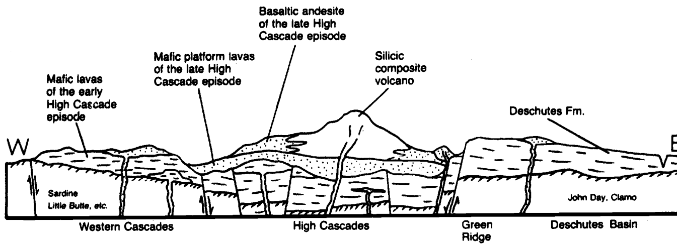
Figure 2.2. Cross-section of Cascade Range in Central Oregon(from Baldwin 1976).
