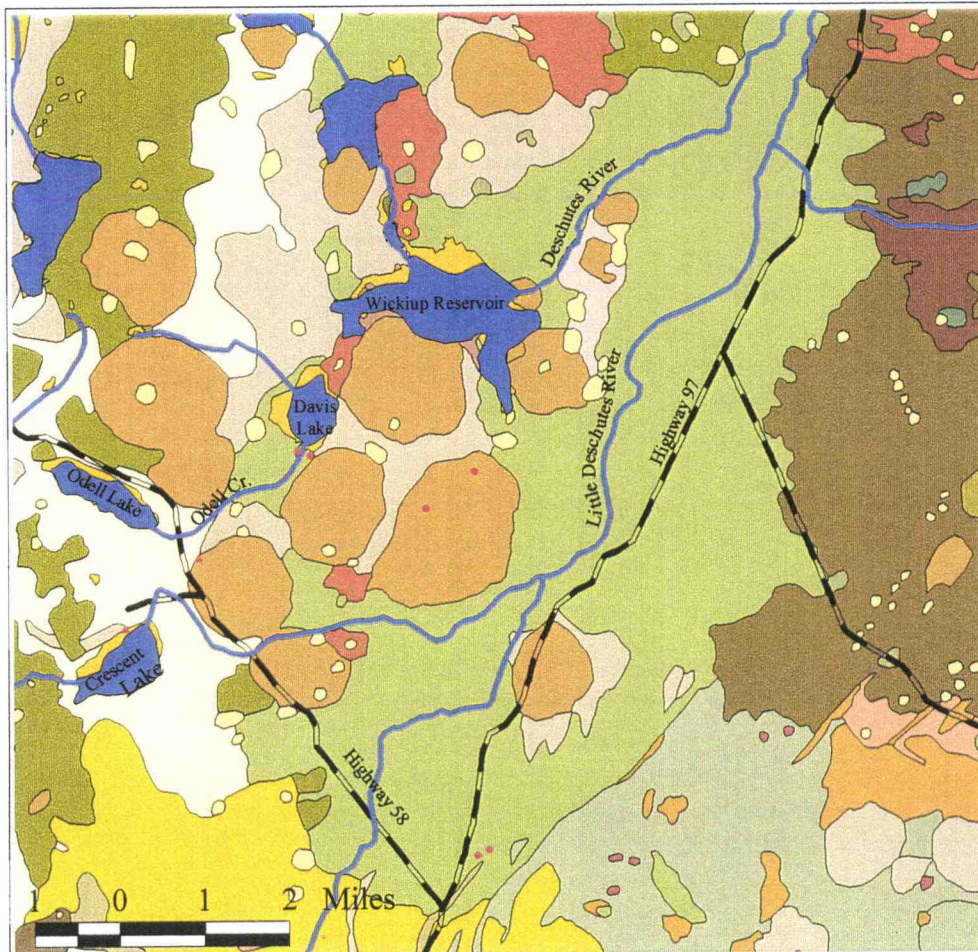
Figure 2.4. Surface geology of the Upper Deschutes River Basin.
