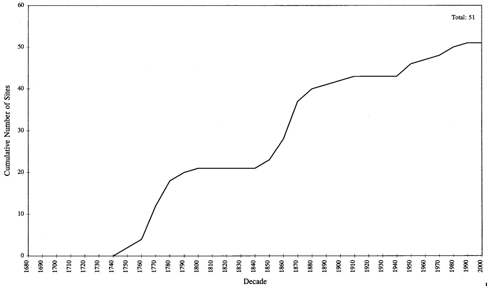
Figure 5.3 Cumulative Number of Old Growth (>200 years) Sites Over Time based on the 20 Stems/ha Criterion
