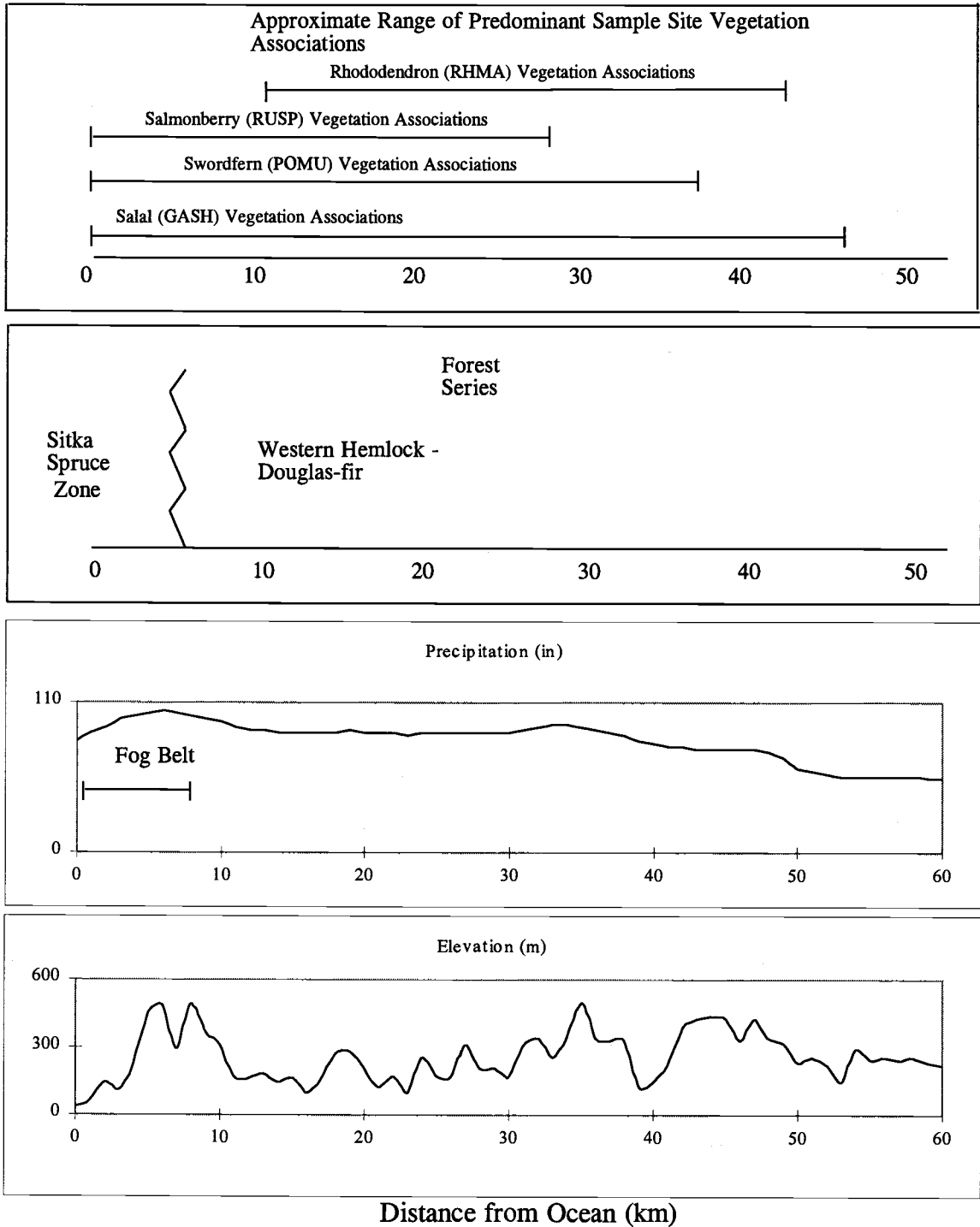
Figure 2.34 A Study Area Transect of Vegetation Type, Precipitation and Elevation
