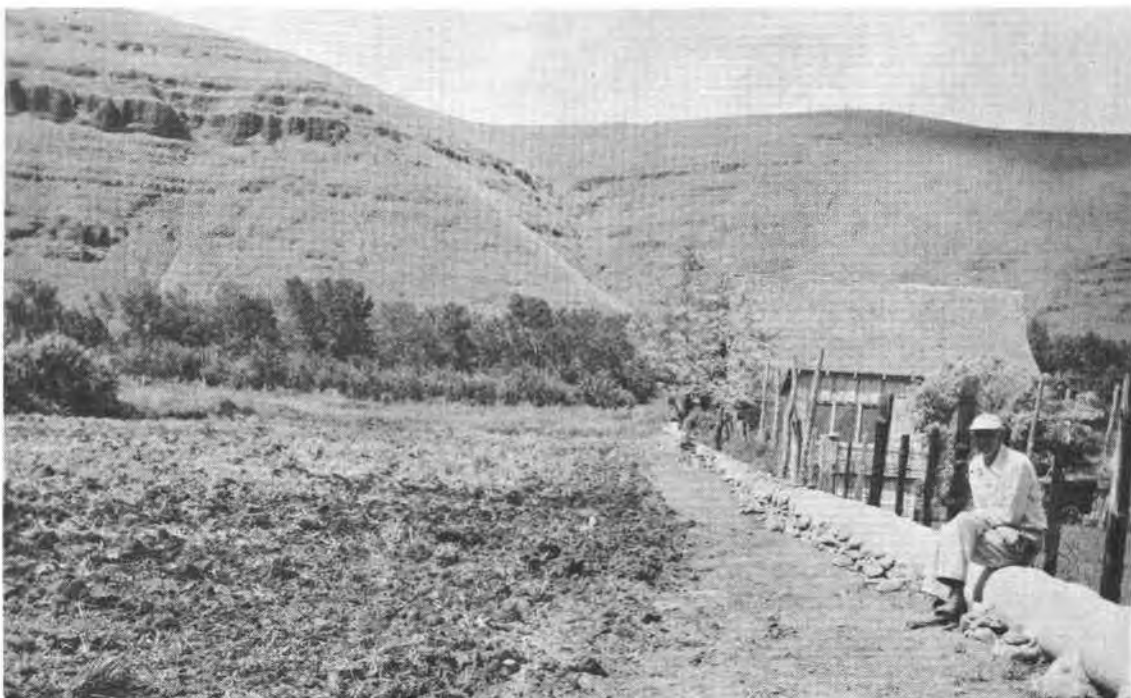
Figure 33.--A concrete pipe has been installed to replace an old wooden flume, subbasin 1. SCS photo. 7-1116-11
