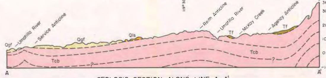
GEOLOGIC SECTION ALONG LINE A-A'
