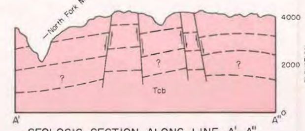
GEOLOGIC SECTION ALONG LINE A'-A''
