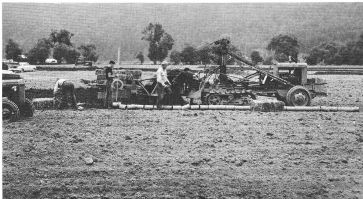
Photo 30.--Some fields are drained by a pattern-type tile system, Clatskanie Soil Conservation District, Oregon. SCS photo
