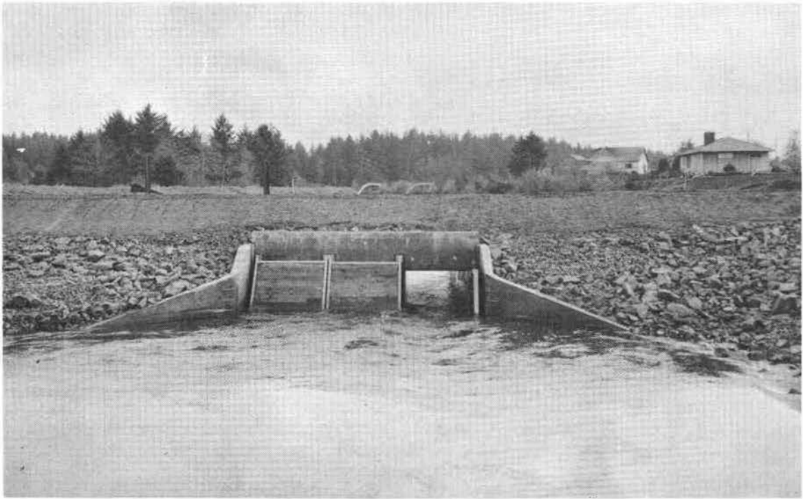
Photo 38.--These flood gates on the Skipanon River are part of the P. L. 566 project near Warrenton. SCS photo
