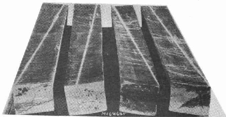
Figure 3.—Twisting of spirally grained wood during seasoning. The two pieces to the left have right-handed spiral grain and the two to the right have left-handed spiral grain, as indicated by the chalk lines on the upper surfaces, which are on the side toward the bark. The lower edges of the farther ends are horizontal (oak).
