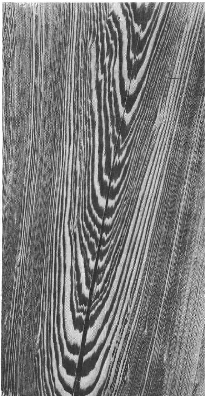
Figure 18. --Artificial spiral grain in baldcypress as indicated by alignment of apexes of annual rings on the tangential surface (when diagonal grain is present) with direction of fibers as shown by the radial split.
