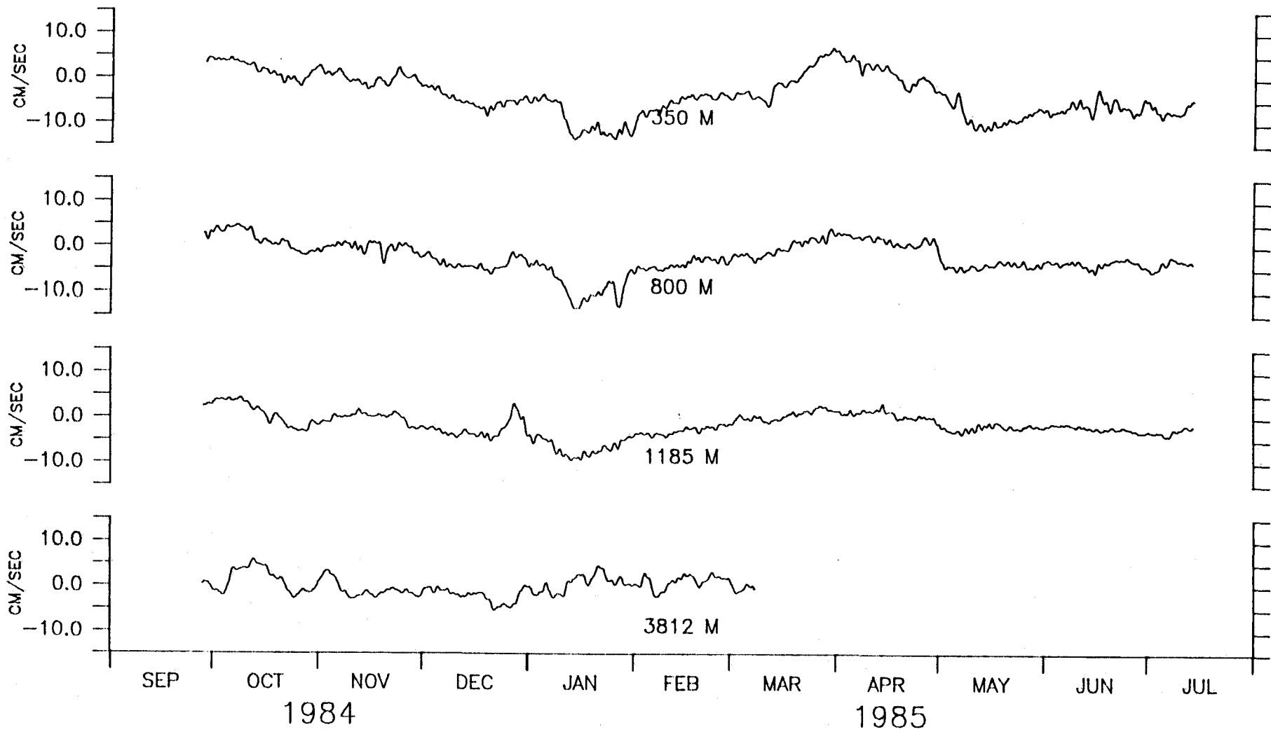
U COMPONENT, M-3.
