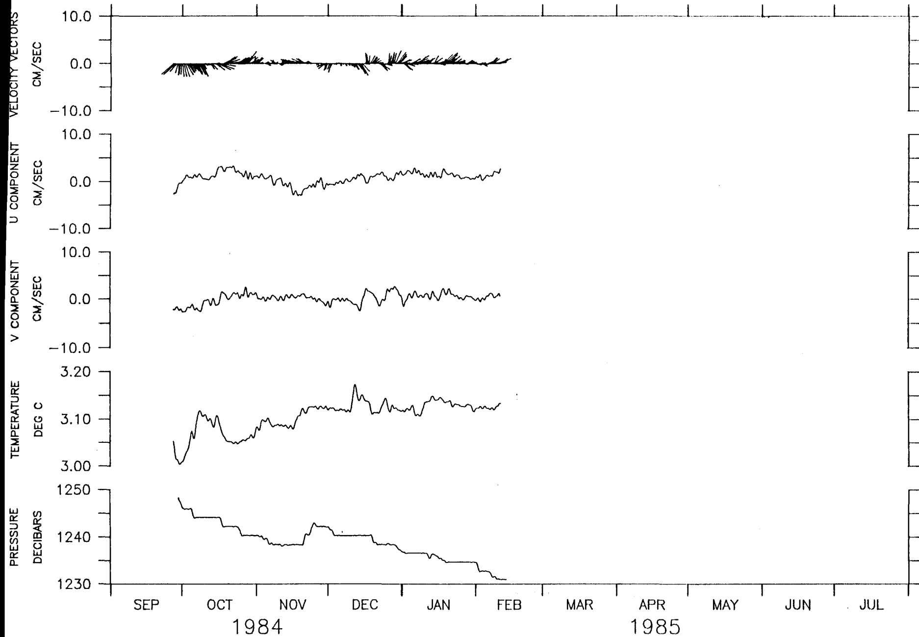
1220 M AT OPTOMA MOORING M1.
