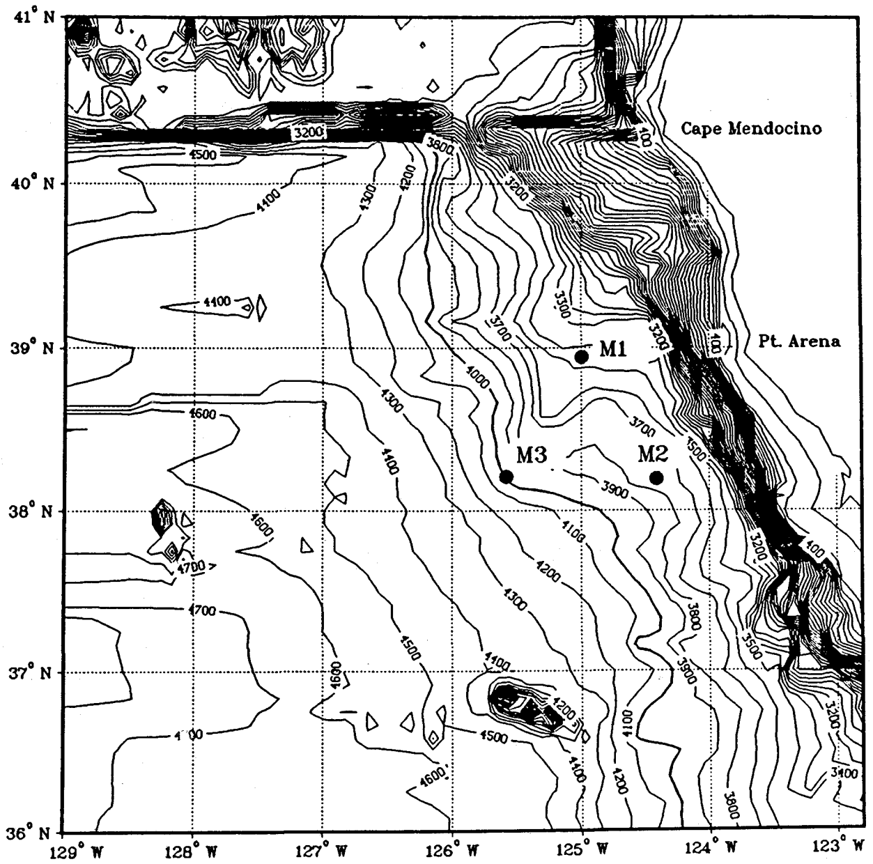
Figure 1. Locations of Moorings M-1, M-2, and M-3.
