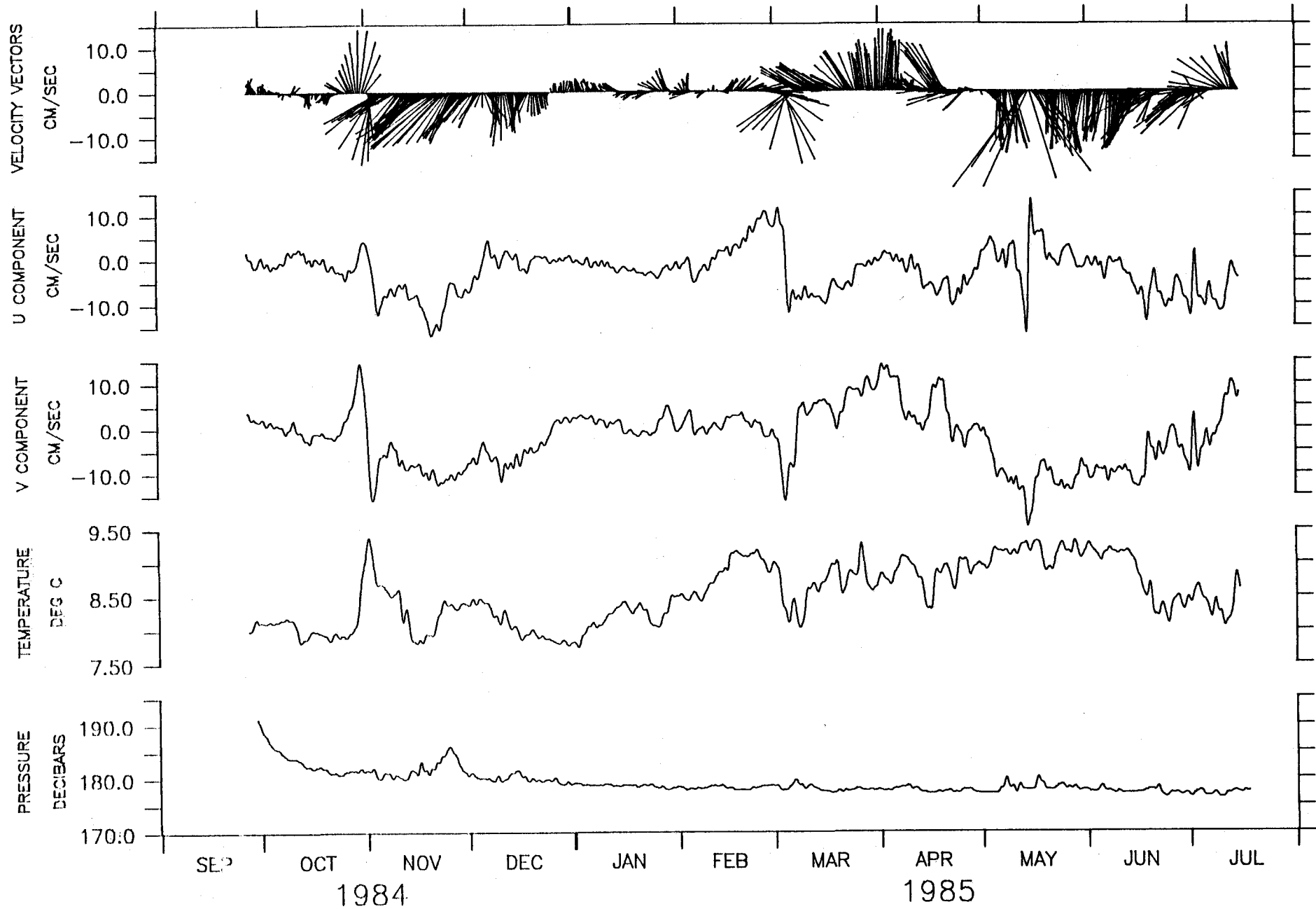
175 M AT OPTOMA MOORING M1.
