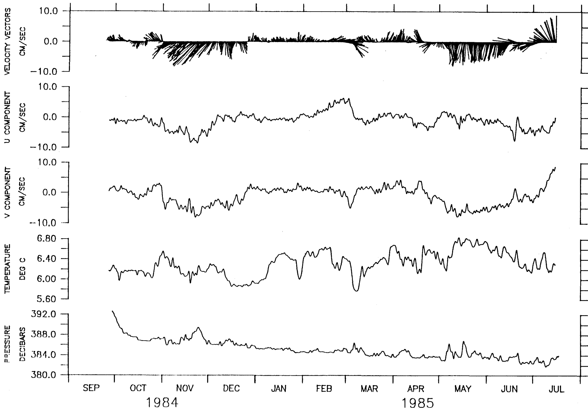
375 M AT OPTOMA MOORING M1.
