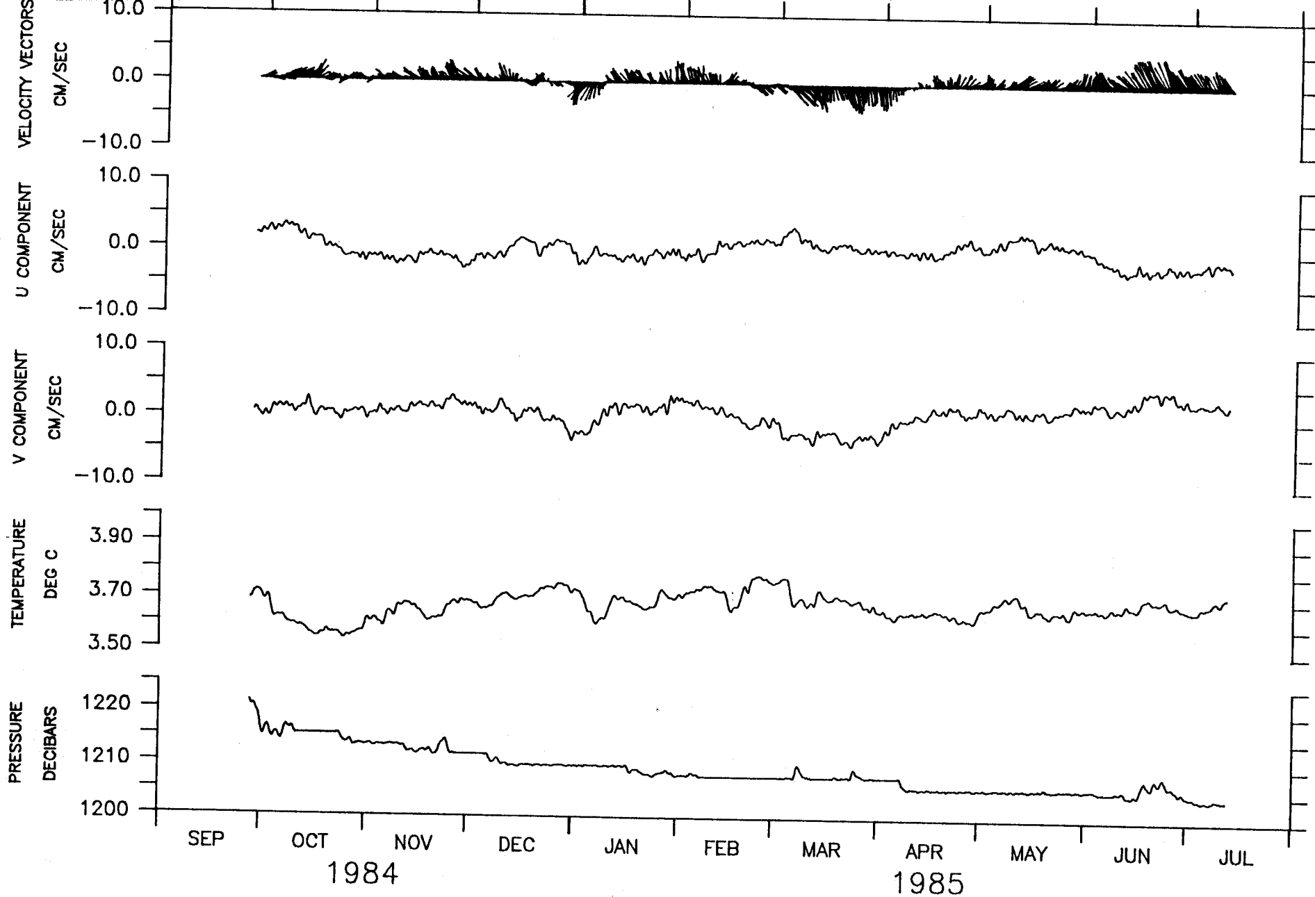
1190 M AT OPTOMA MOORING M-2.
