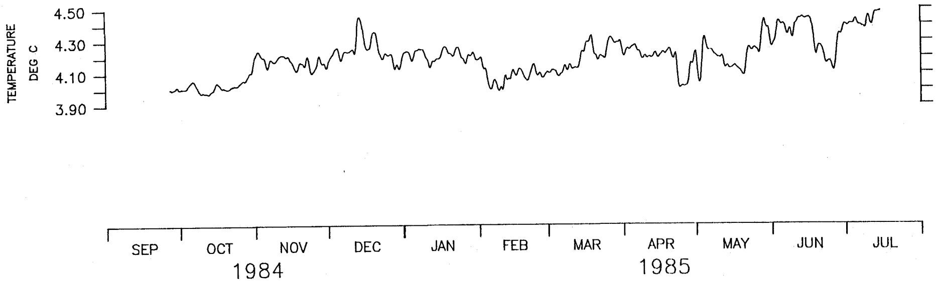
800 M AT OPTOMA MOORING M-1.
