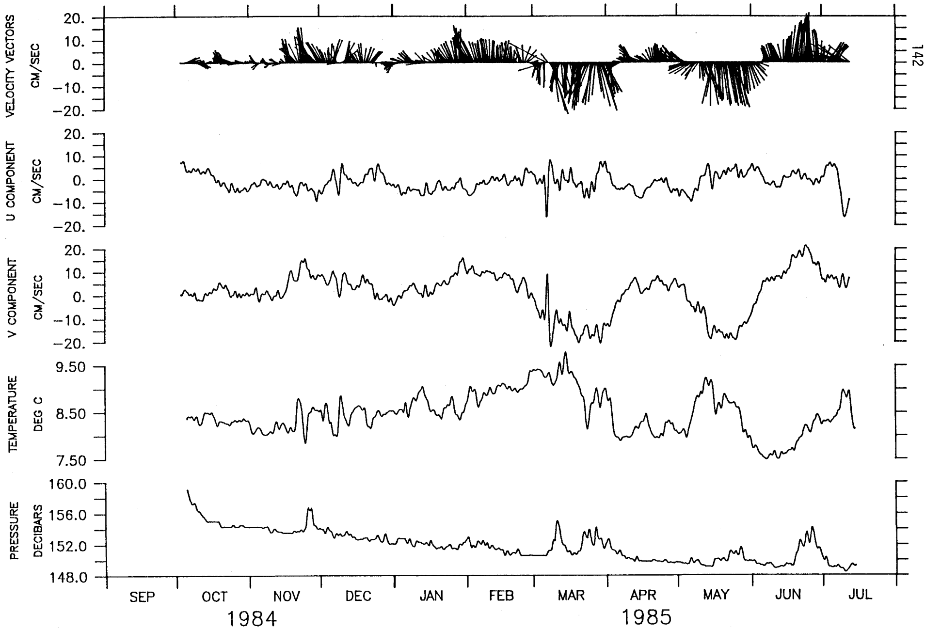
145 M AT OPTOMA MOORING M-2.
