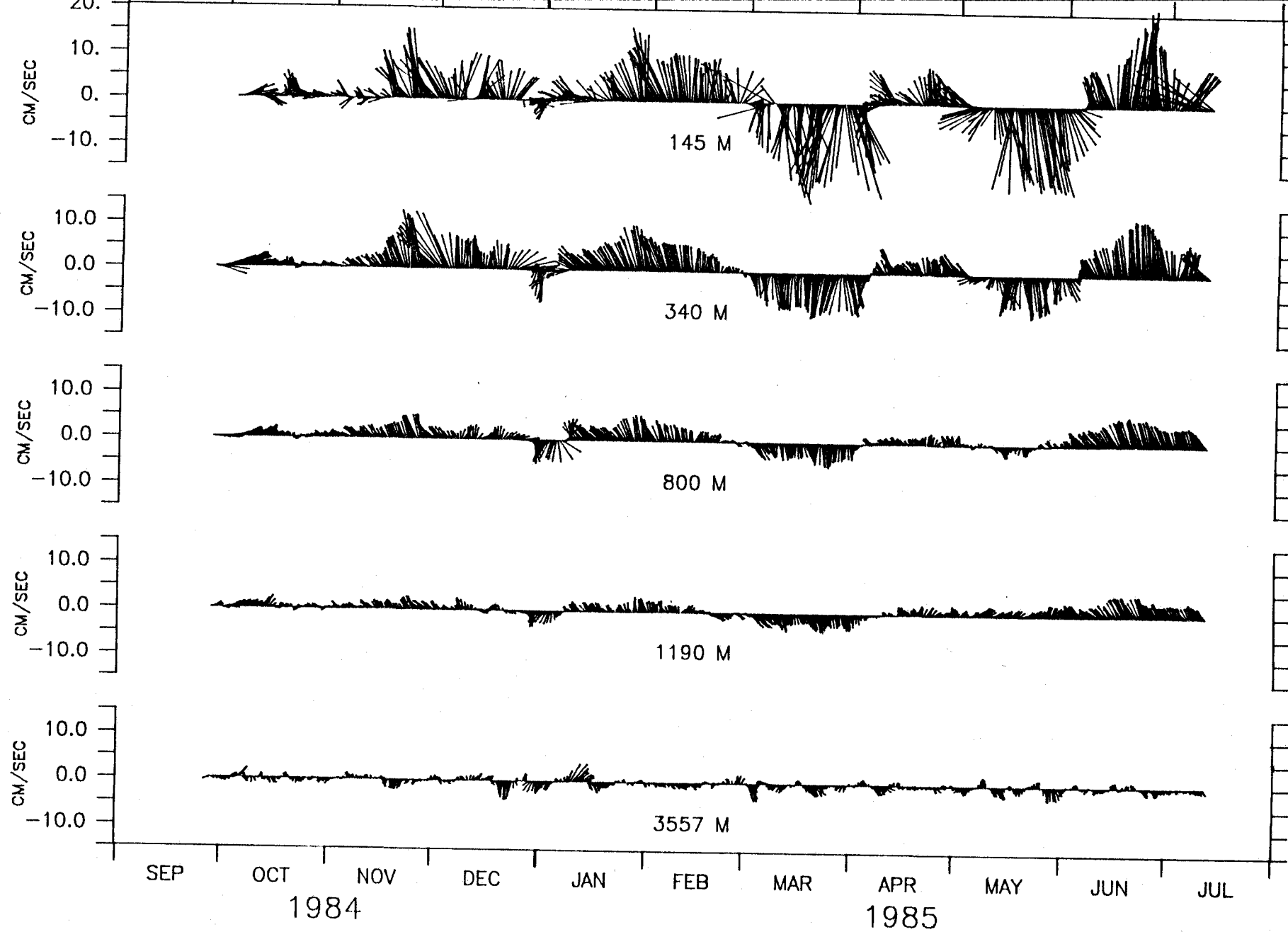
VELOCITY VECTORS, M-2.
