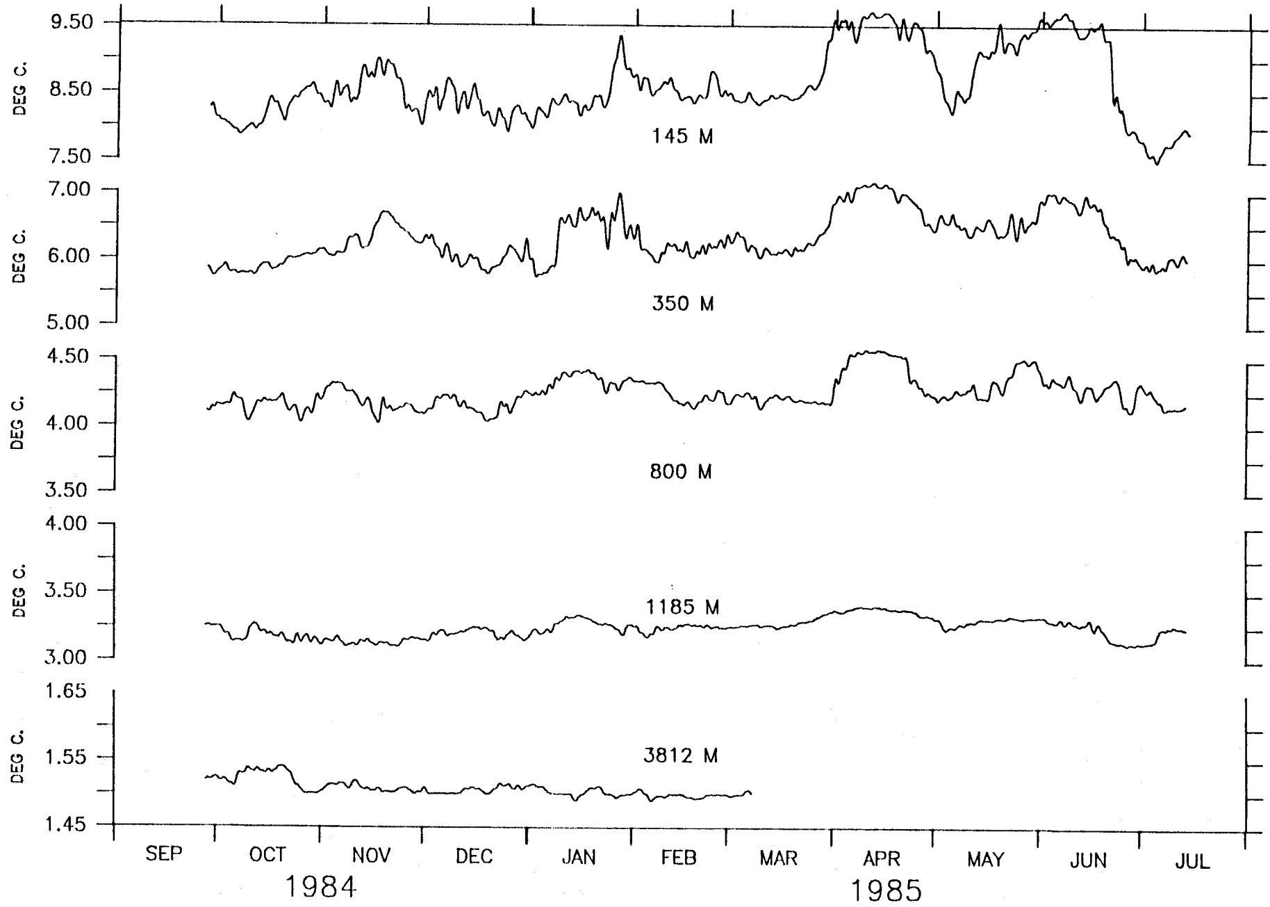
TEMPERATURE M-3.
