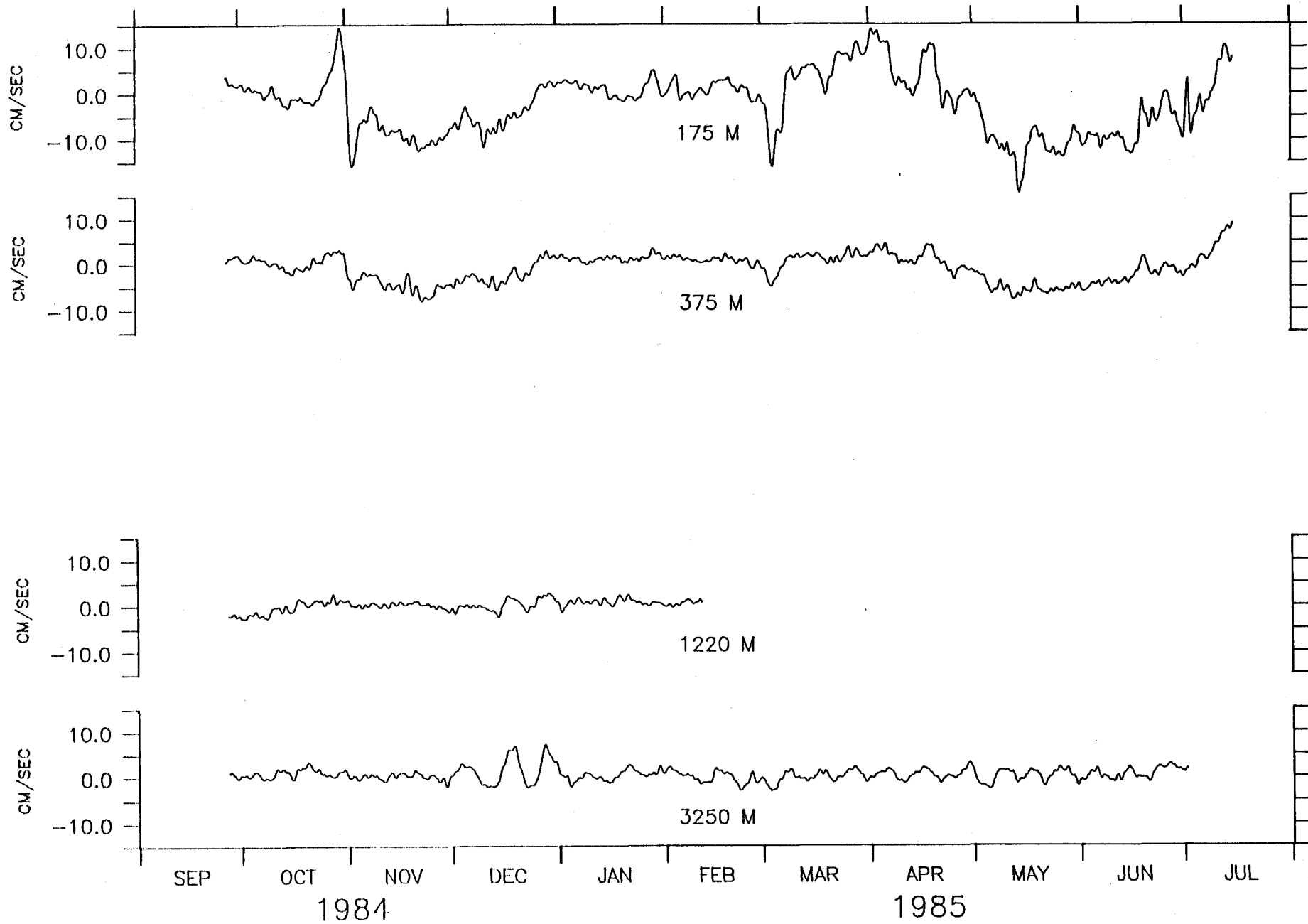
V COMPONENT, M-1.
