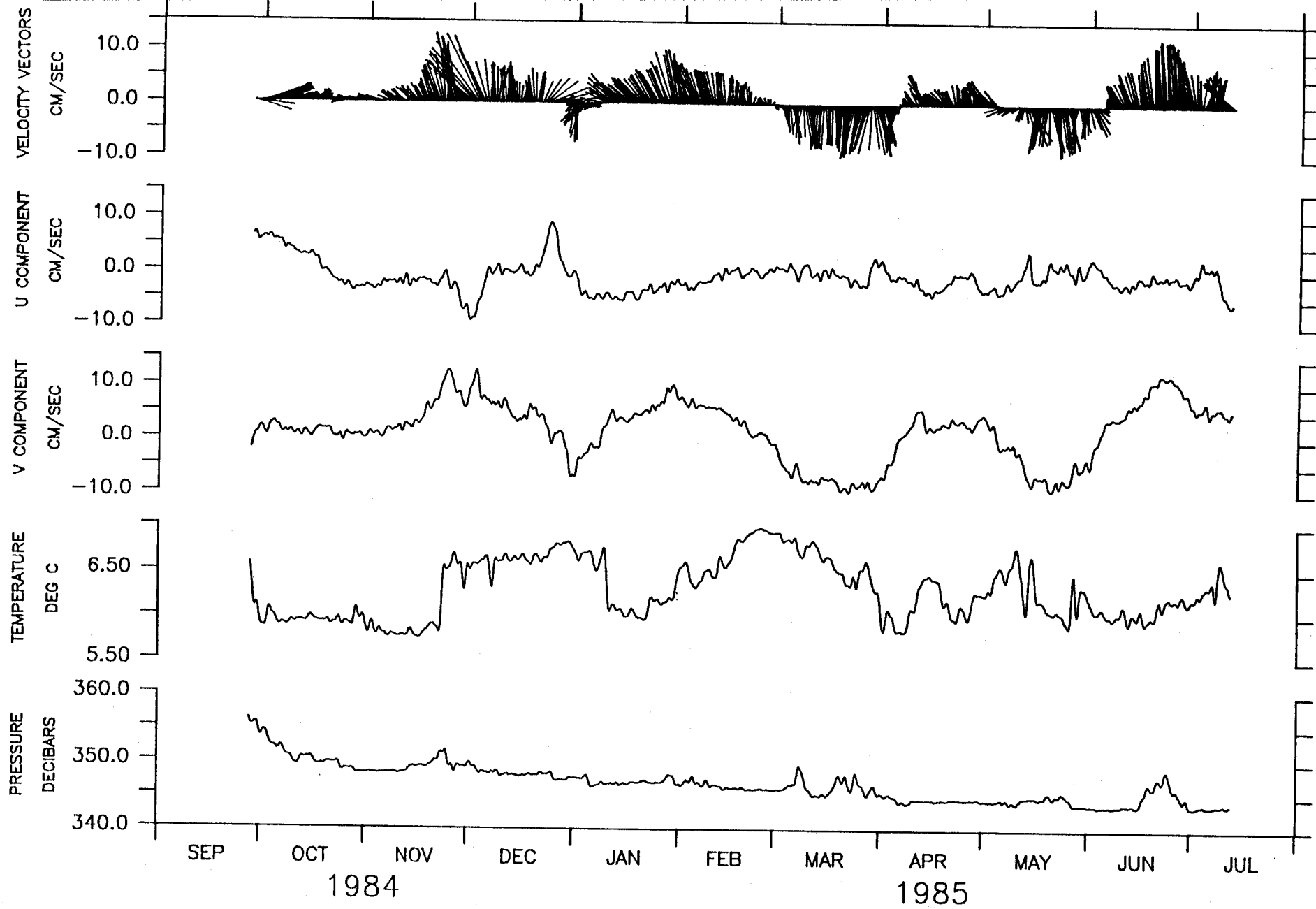
340 M AT OPTOMA MOORING M-2.
