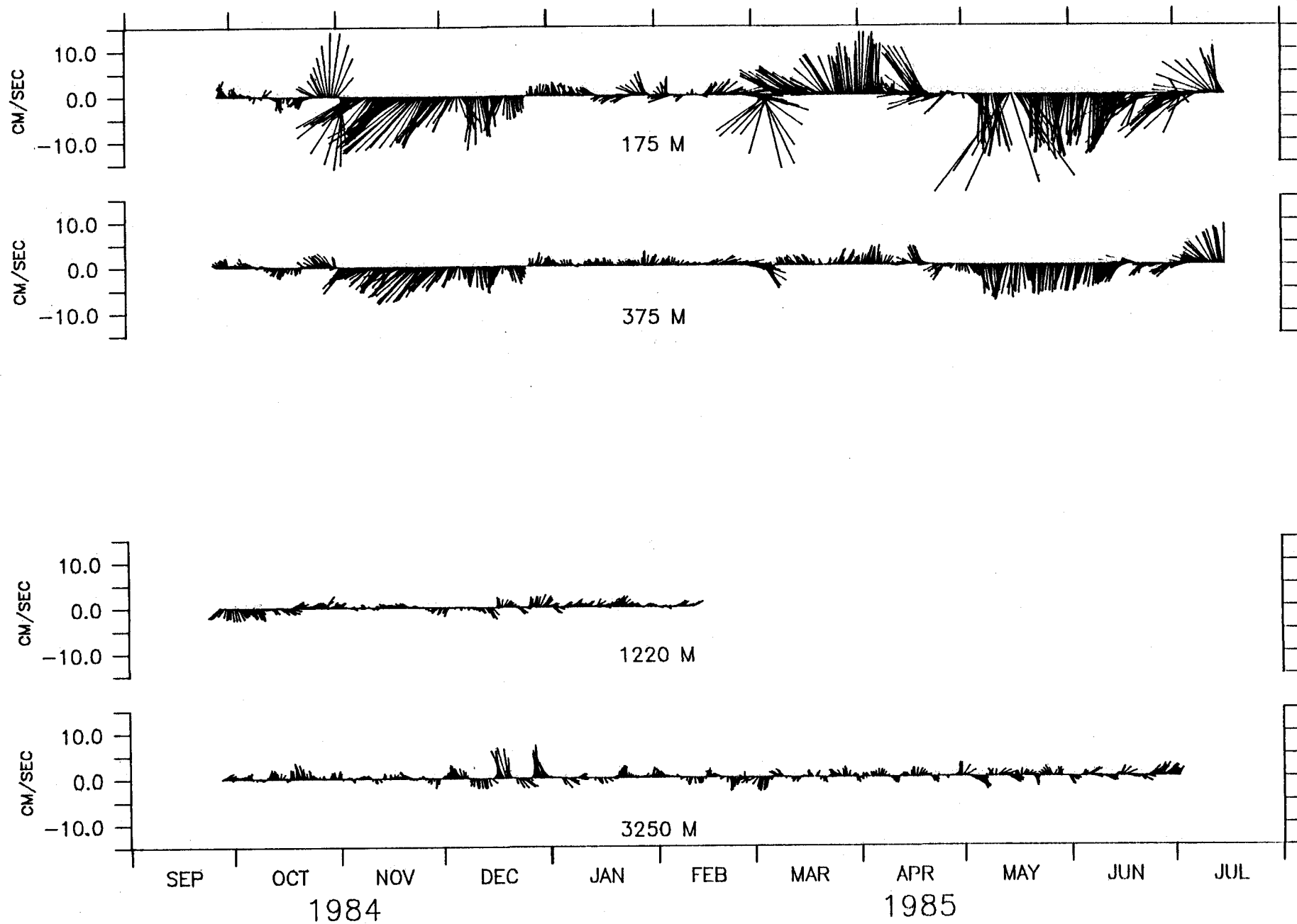
VELOCITY VECTORS, M-1.
