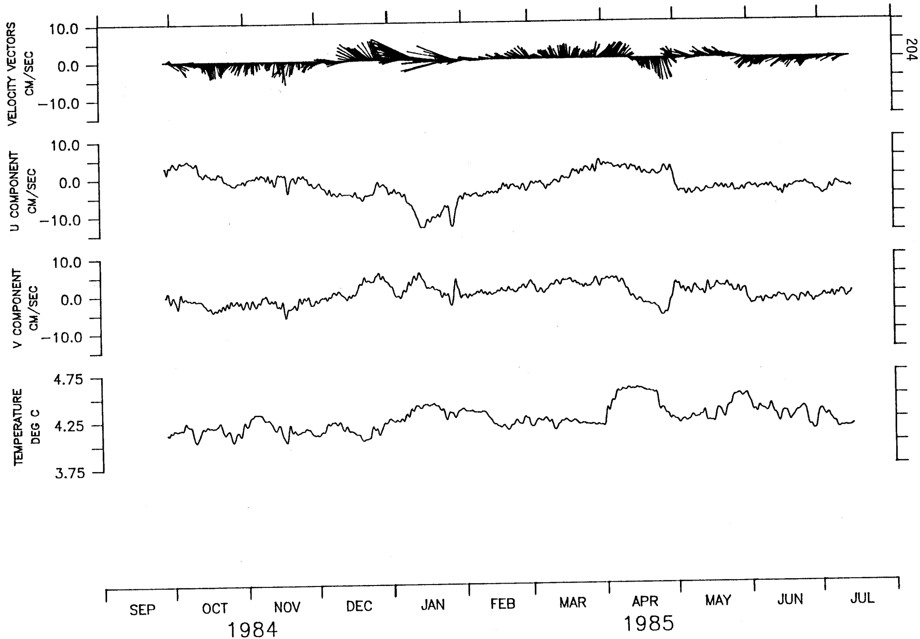
800 M AT OPTOMA MOORING M-3.
