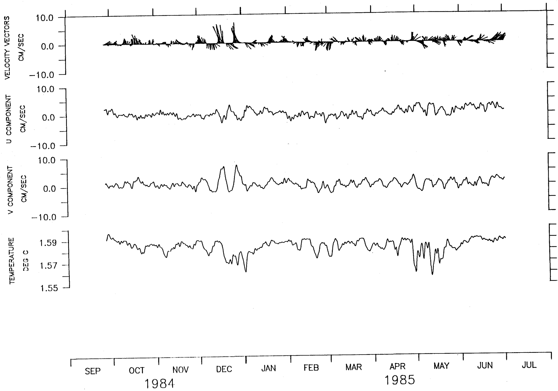
3250 M AT OPTOMA MOORING M1.
