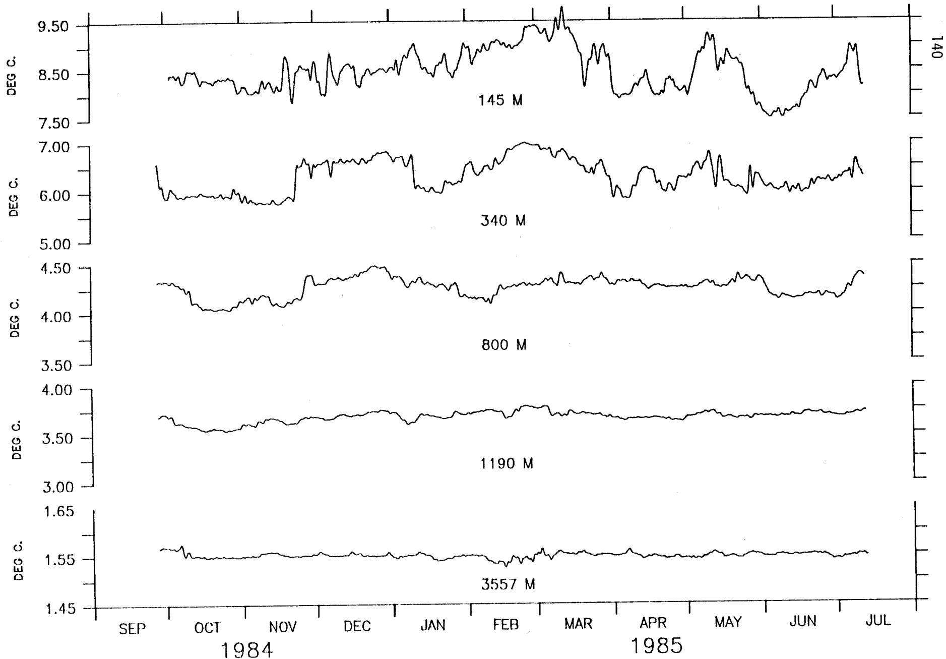
TEMPERATURE M-2.
