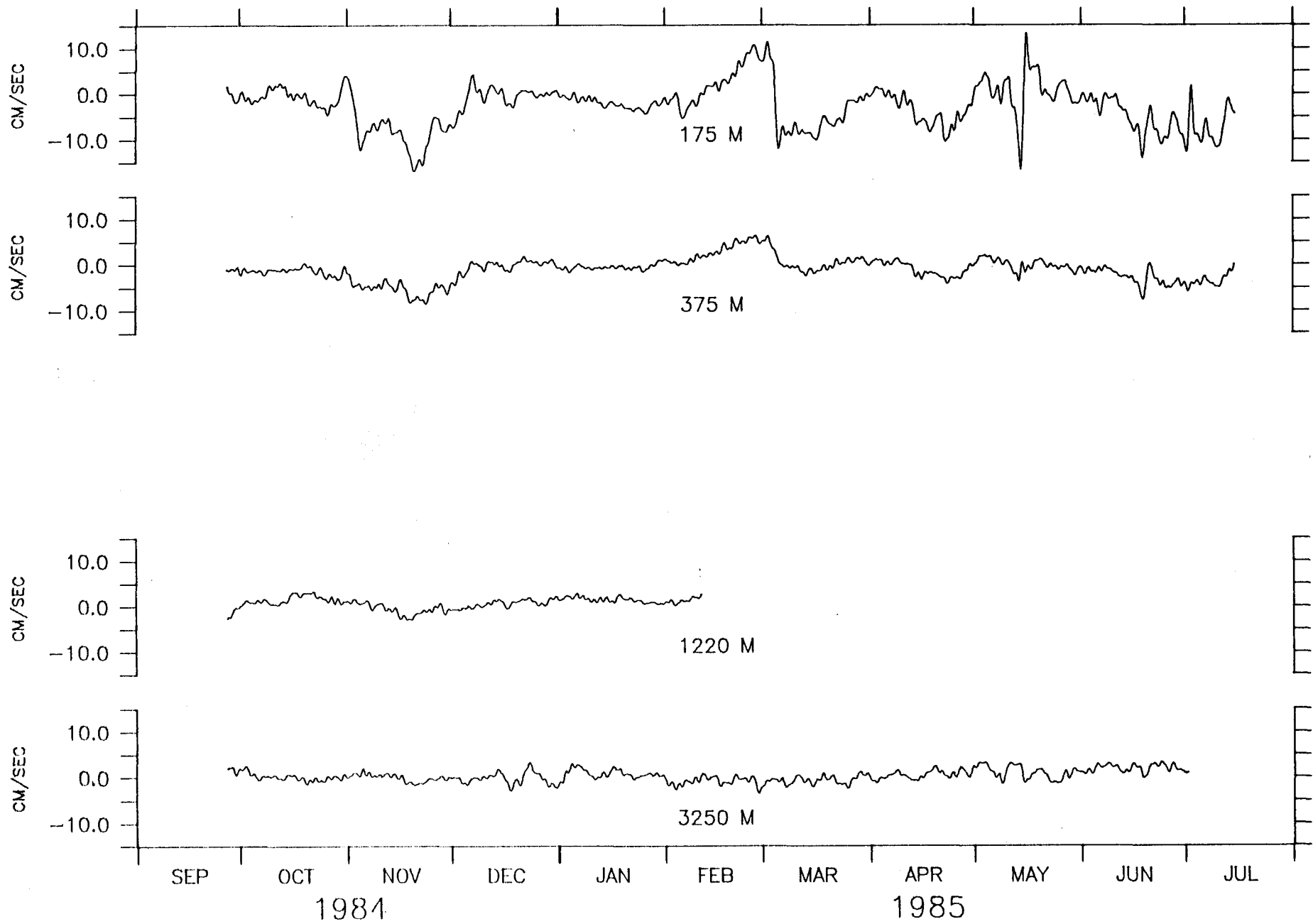
U COMPONENT, M-1.
