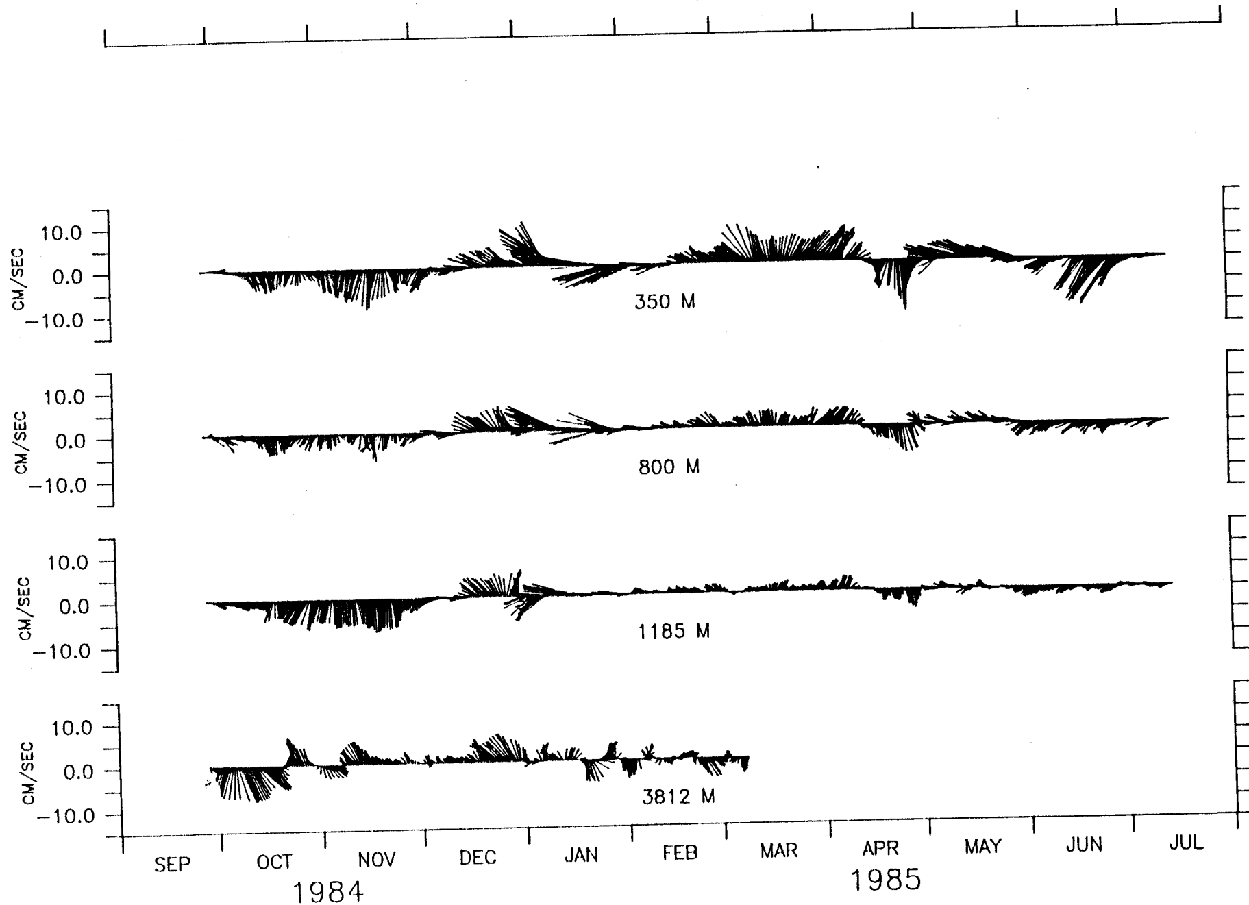
VELOCITY VECTORS, M-3.
