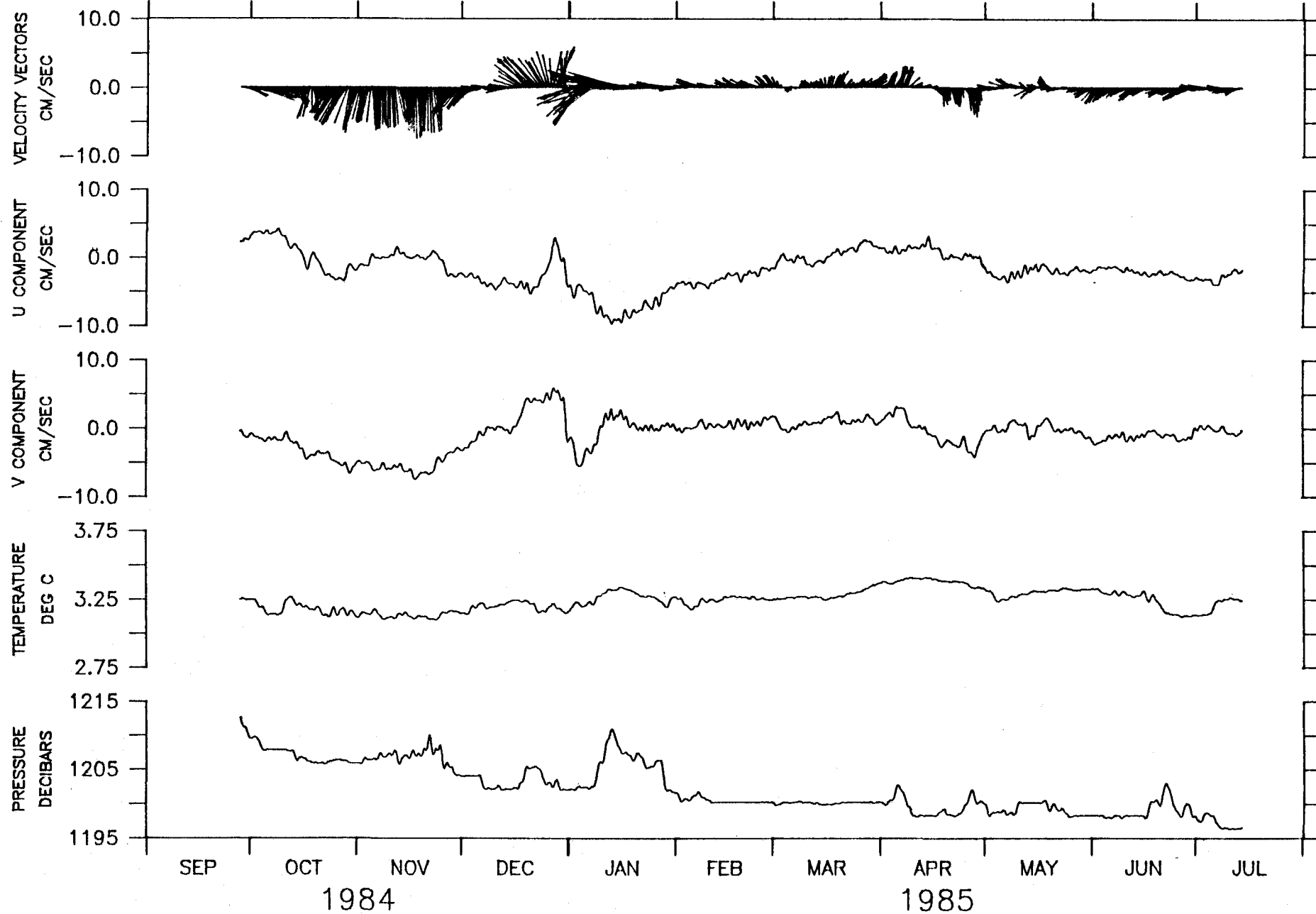
1185 M AT OPTOMA MOORING M-3.
