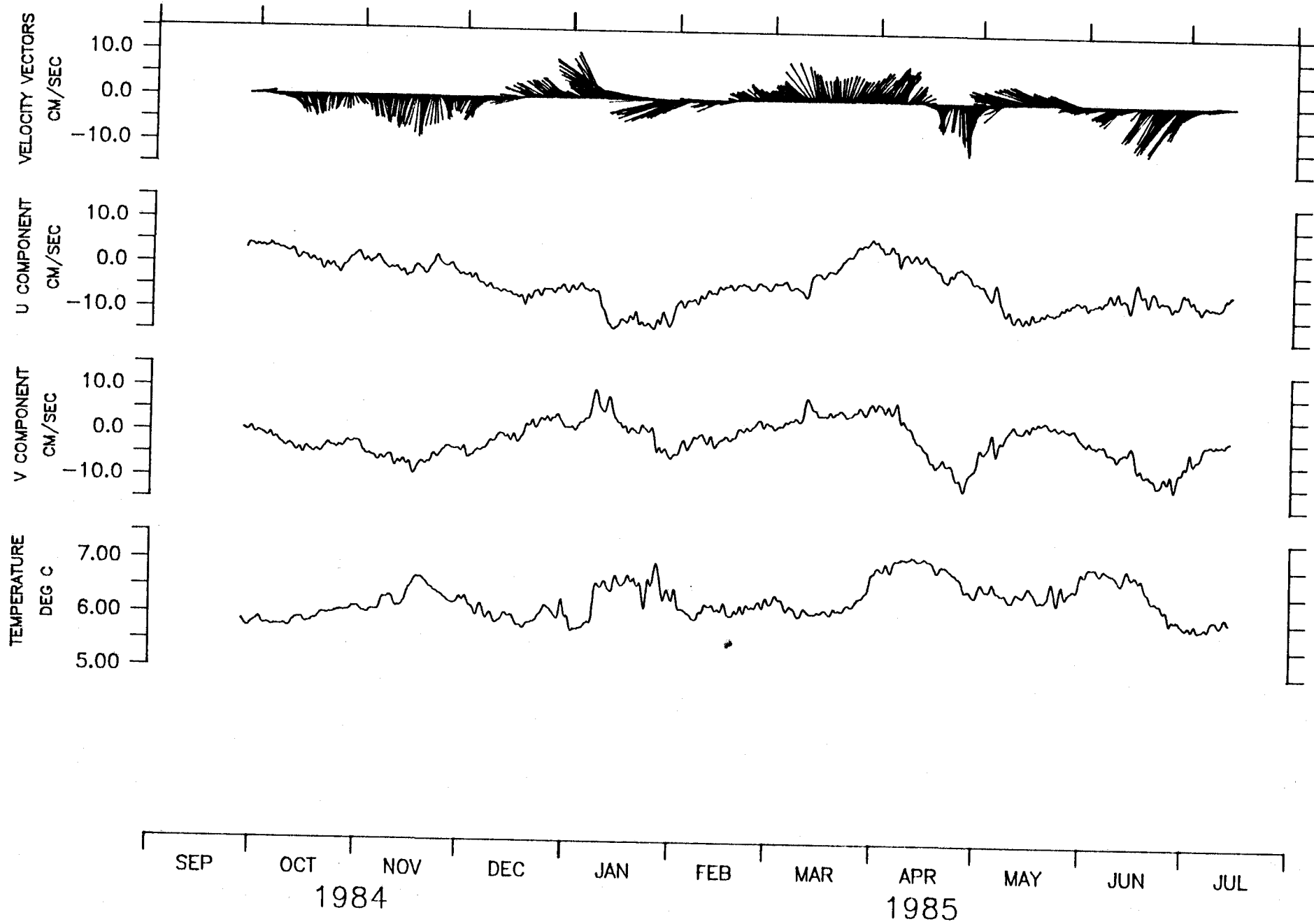
350 M AT OPTOMA MOORING M-3.
