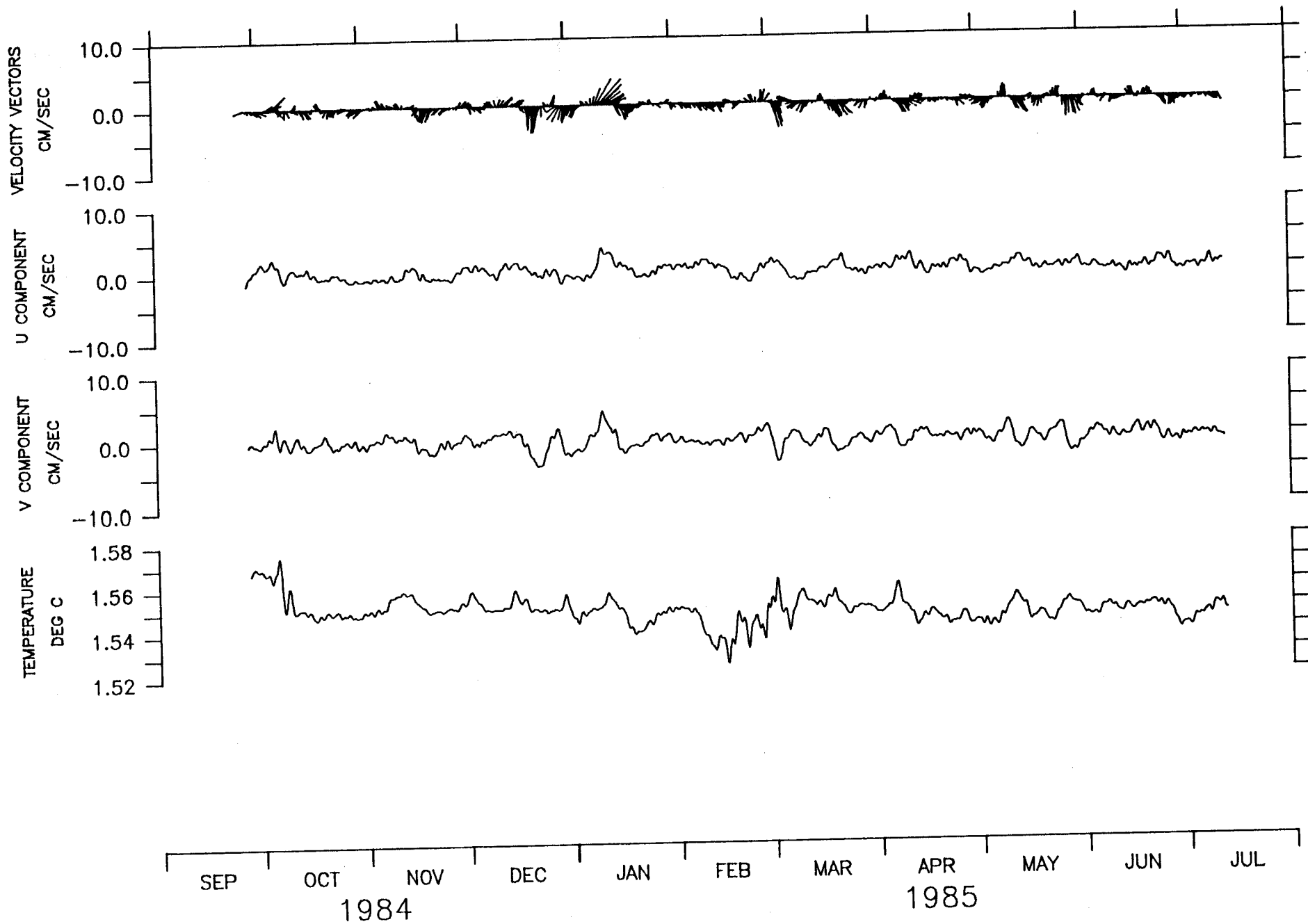
3557 M AT OPTOMA MOORING M-2.
