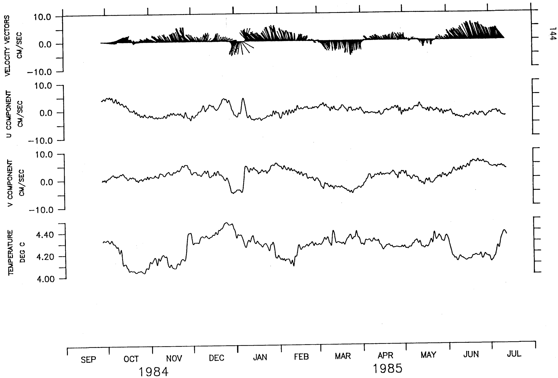
800 M AT OPTOMA MOORING M-2.
