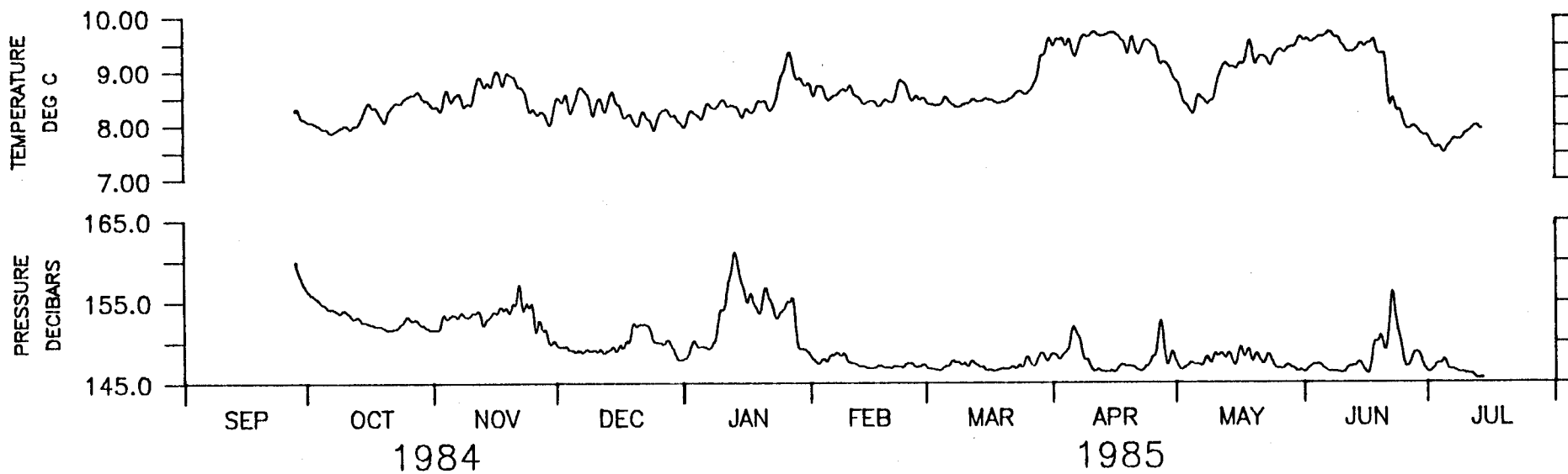
145 M AT OPTOMA MOORING M-3.
