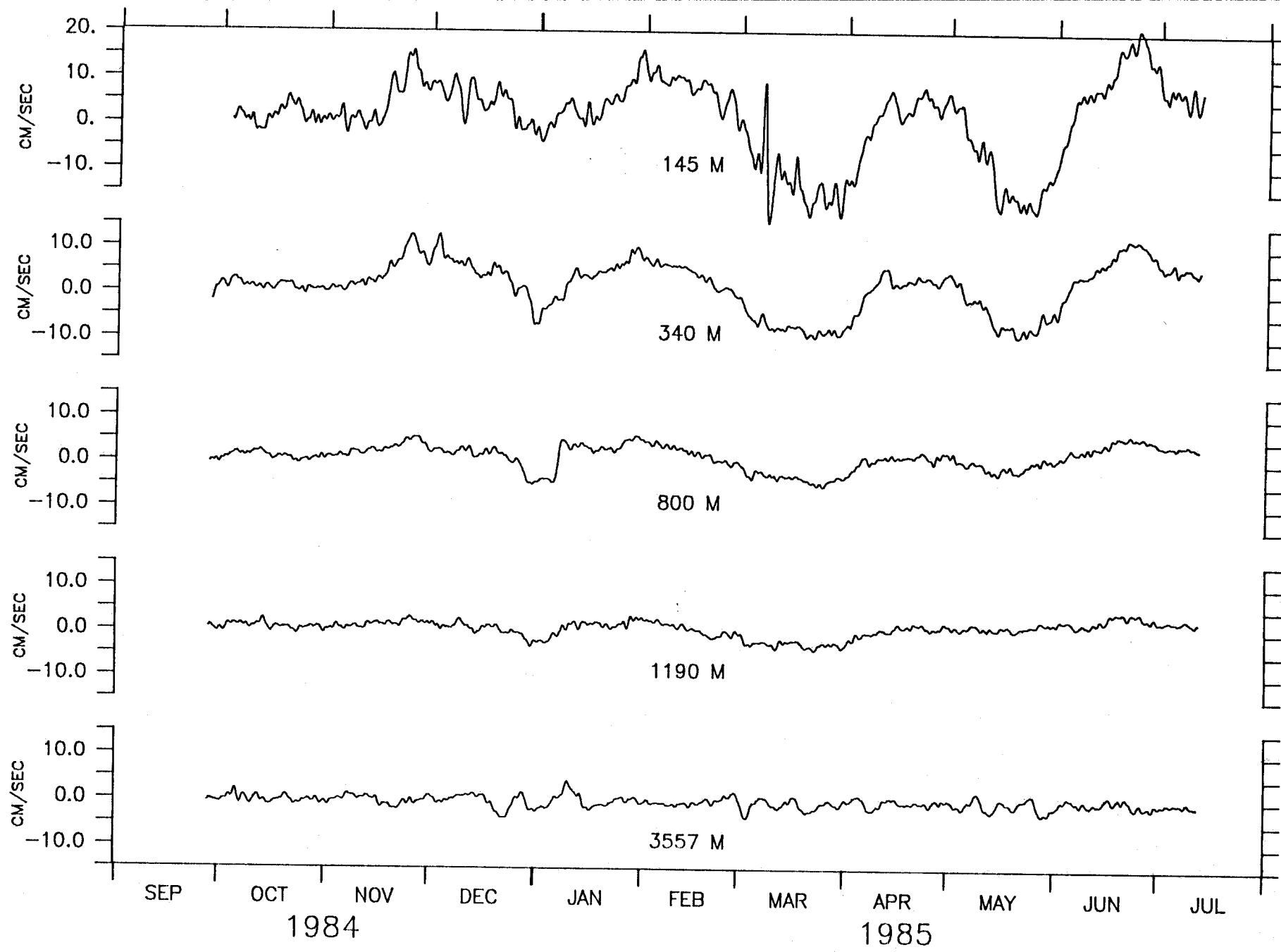
V COMPONENT, M-2.
