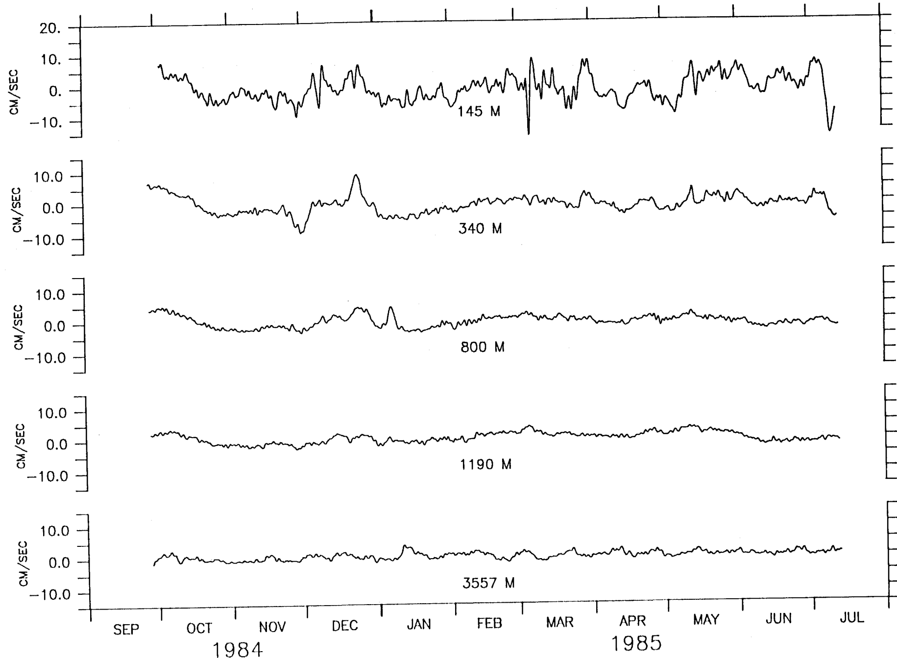
U COMPONENT, M-2.
