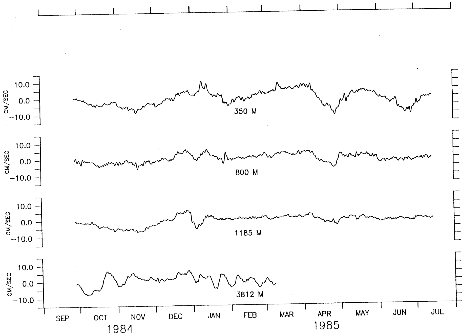
V COMPONENT, M-3.
