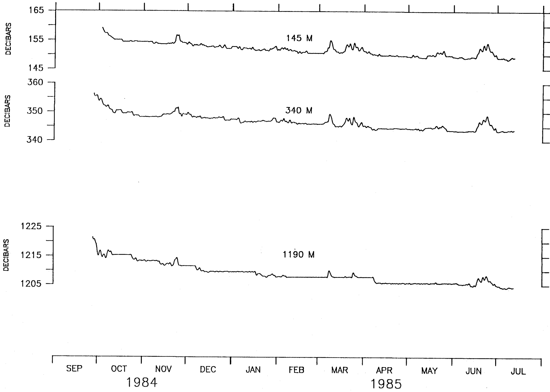
PRESSURE M-2.
