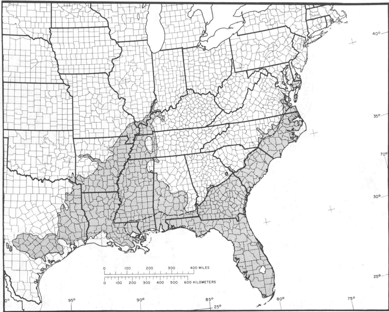
Figure 1.—Natural range of baldcypress, Taxodium distichum . The broken line indicates the northern limit of the variety pondcypress, T. distichum var. nutans (Ait.) Sweet.
