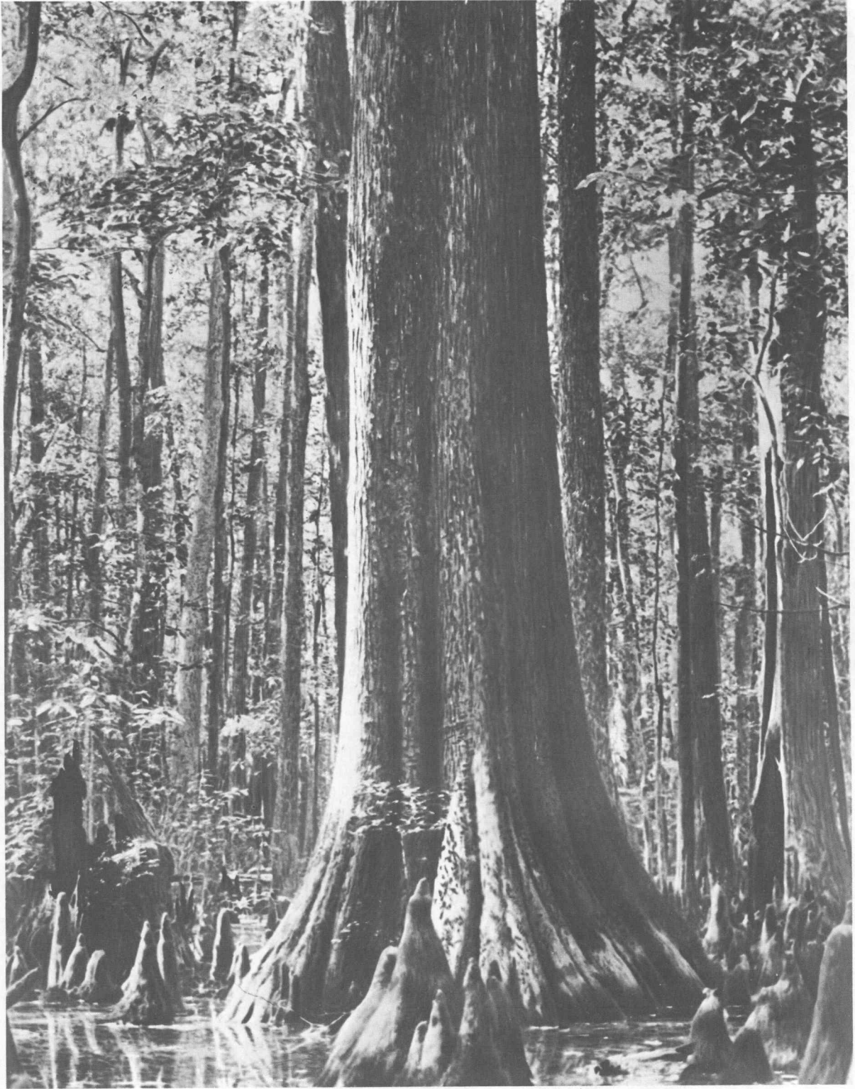
Figure 2.—Baldcypress “knees” may anchor the tree and supply additional oxygen.
