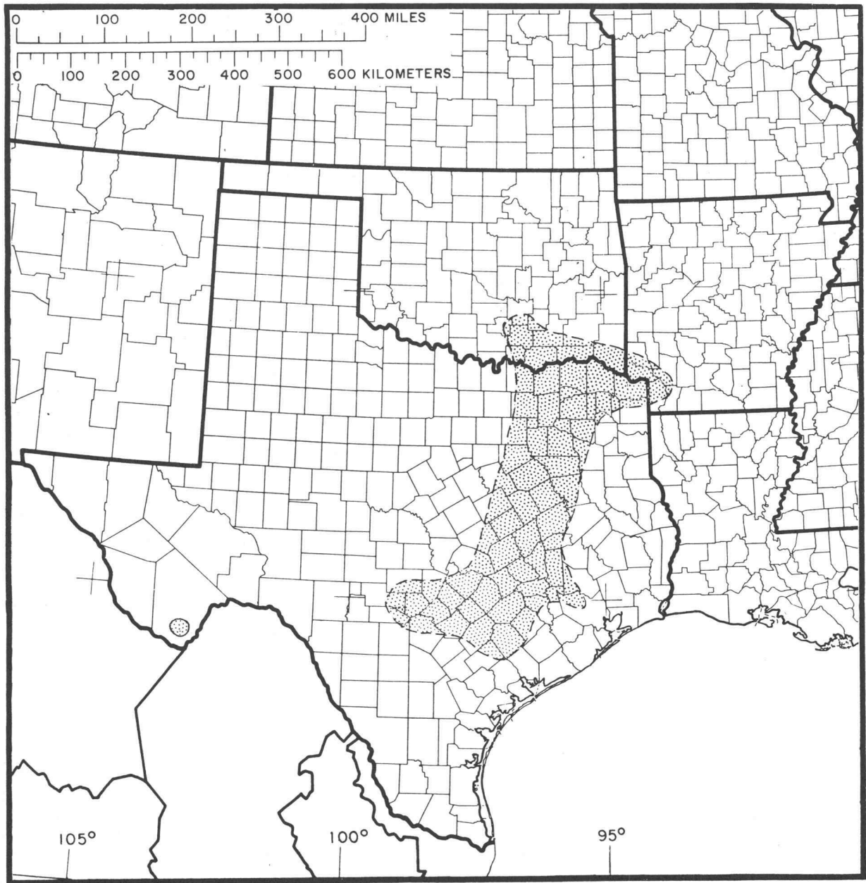
Figure 1.—Natural range of osage-orange, Maclura promifera Raf. Schneid. This map shows the approximate original natural distribution. The range has been extended greatly by planting.
